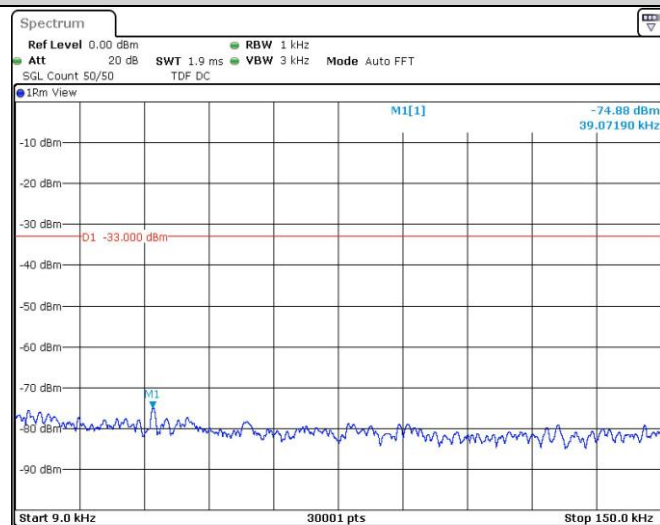
Band5-4182-3-0.009~0.15MHz
