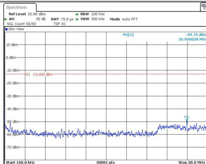
Band5-4182-2-0.15~30MHz
