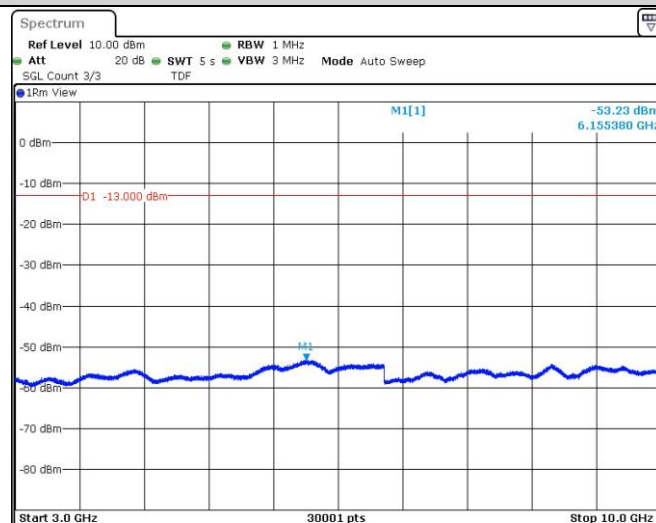
Band5-4132-2-3000~10000MHz
