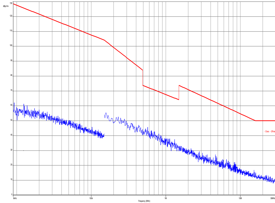
Plot 5: Channel 18900 (Traffic mode up to 30 MHz)
