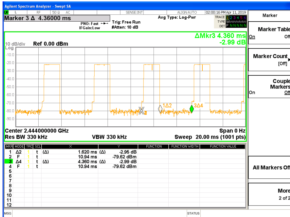
ON TIME AND DUTY CYCLE PLOT-2
