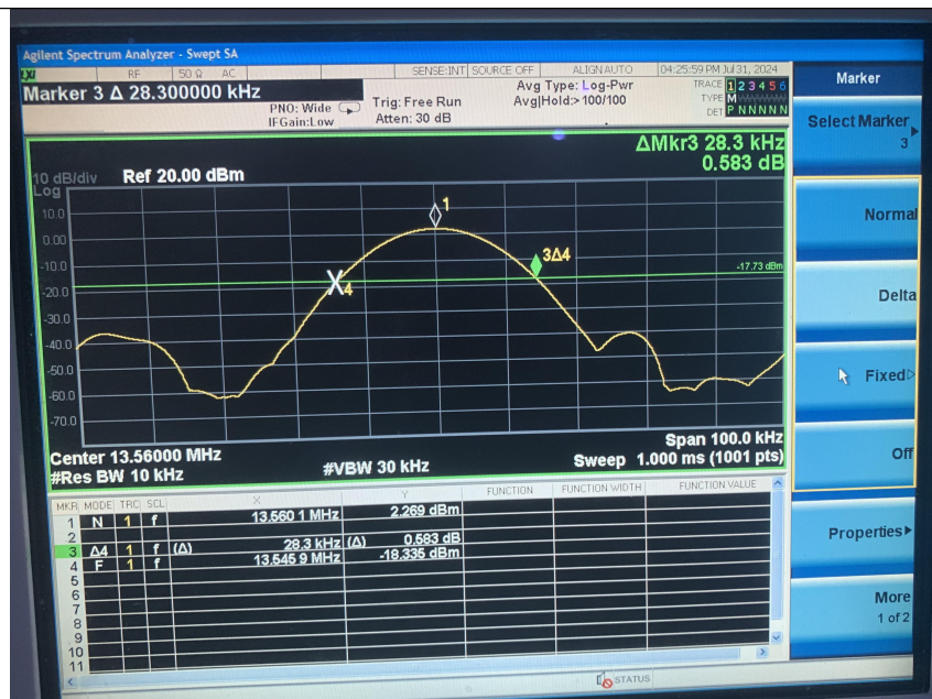
ASK Modulation
