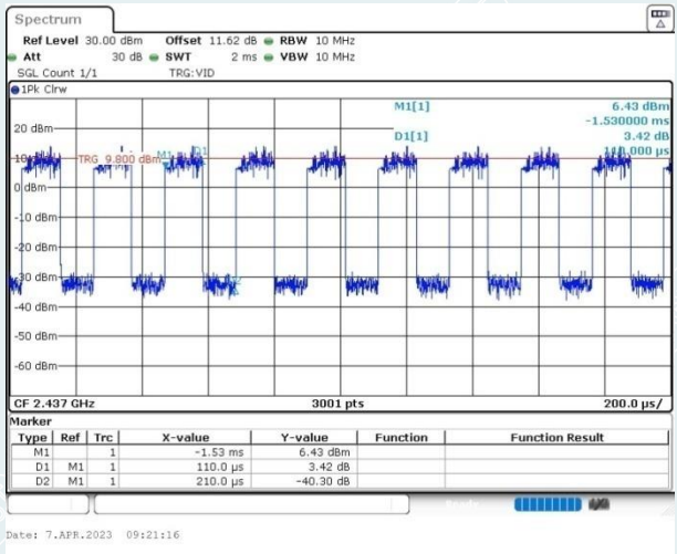
802.11n HT40_Ant1_2437MHz
