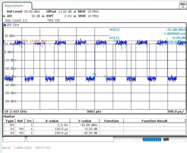
802.11n HT20_Ant1_2437MHz
