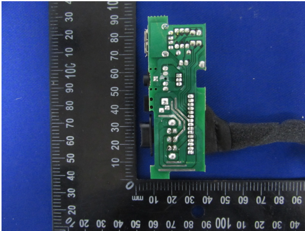
Internal Photos Model: BL1606B
