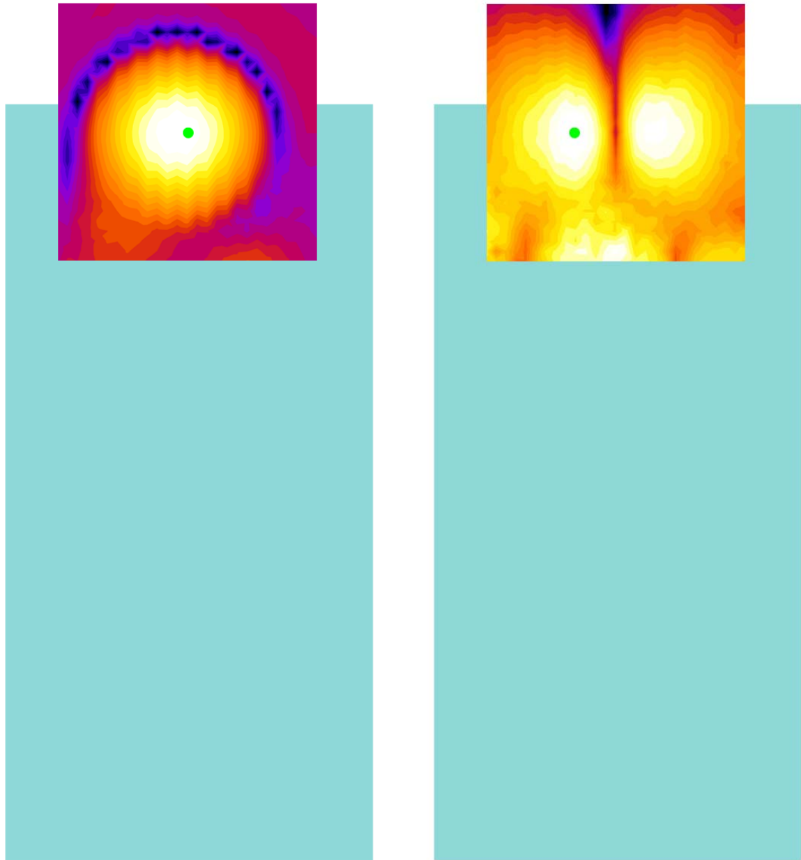
Figure 9-2 T-Coil Scan Overlay Magnetic Field Distributions for OTT VoIP Modes
