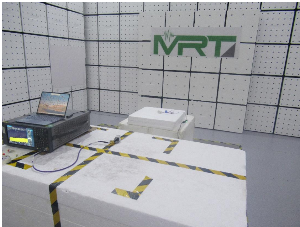
Photograph 5: Set-up photo for Radiated Spurious Emission, 40GHz ~ 50GHz
