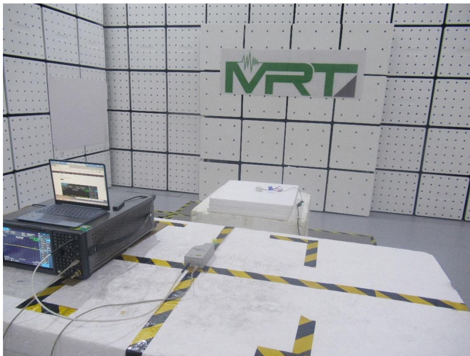
Photograph 7: Set-up photo for Radiated Spurious Emission, 75GHz ~ 100GHz
