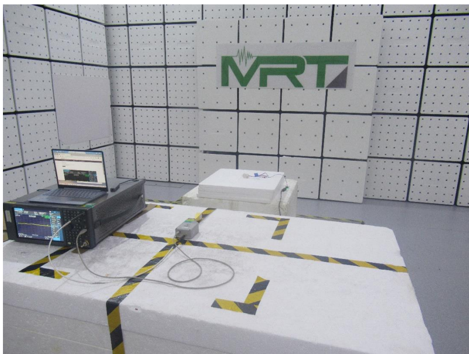
Photograph 6: Set-up photo for Radiated Spurious Emission, 50GHz ~ 75GHz
