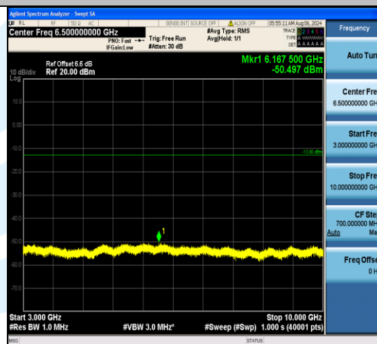
Band5_1.4MHz_QPSK_20525_1RB#0_3000~10000_3000~10000
