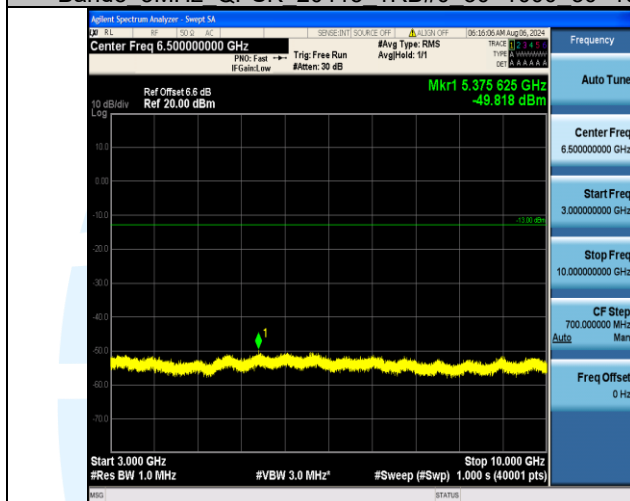
Band5_3MHz_QPSK_20415_1RB#0_3000~10000_3000~10000
