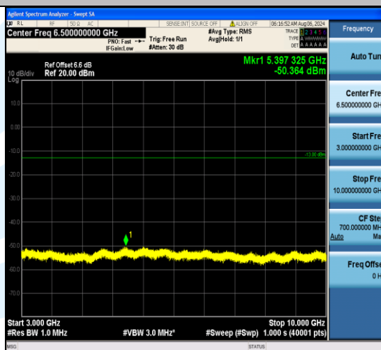
Band5_3MHz_QPSK_20415_1RB#14_3000~10000_3000~10000
