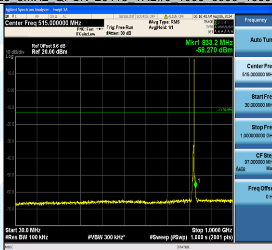
Band5_3MHz_QPSK_20415_1RB#14_30~1000_30~1000
