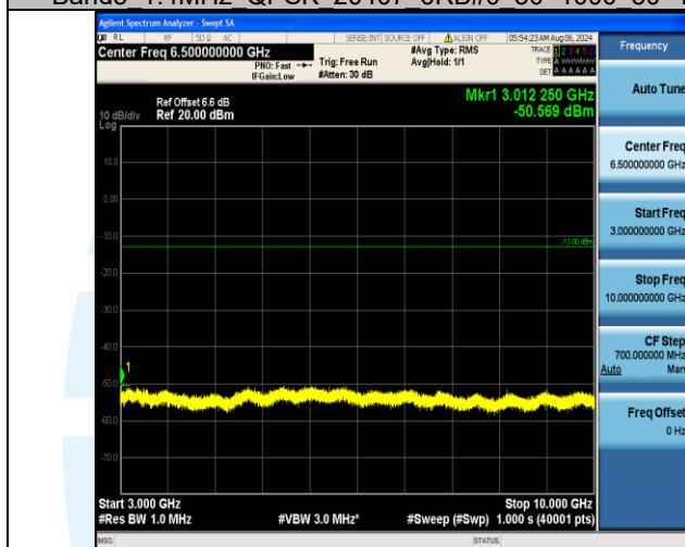
Band5_1.4MHz_QPSK_20407_6RB#0_3000~10000_3000~10000
