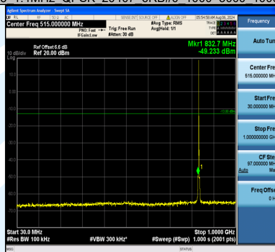
Band5_1.4MHz_QPSK_20525_1RB#0_30~1000_30~1000
