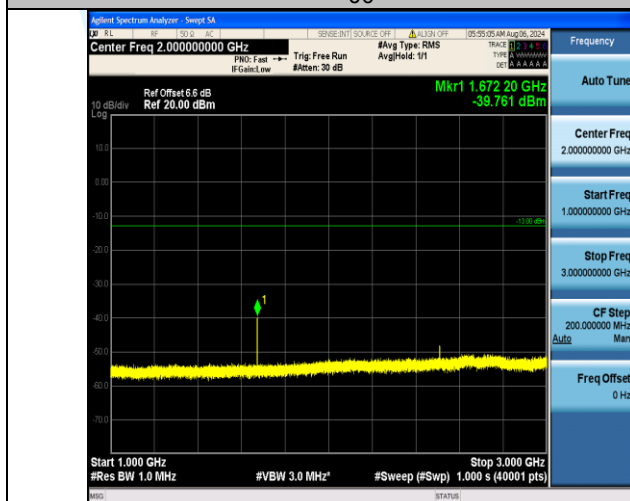
Band5_1.4MHz_QPSK_20525_1RB#0_1000~3000_1000~3000
