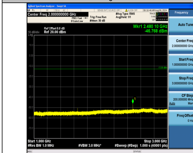
Band5_3MHz_QPSK_20415_1RB#14_1000~3000_1000~3000
