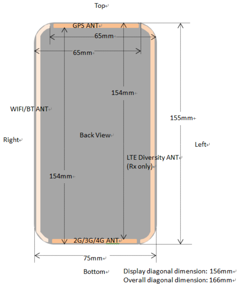
Fig.14.1 EUT Antenna Locations
