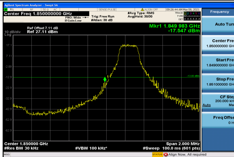
Band25-3MHz-16QAM-26055-1RB#0
