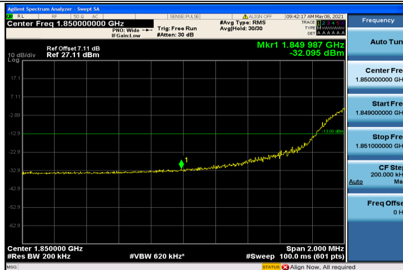
Band25-20MHz-QPSK-26140-100RB#0
