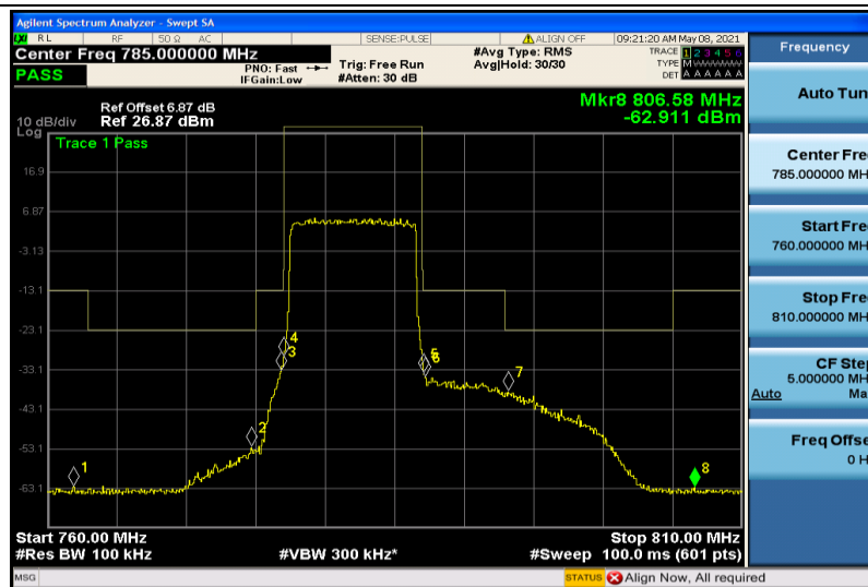
Band13-10MHz-QPSK-23230-50RB#0
