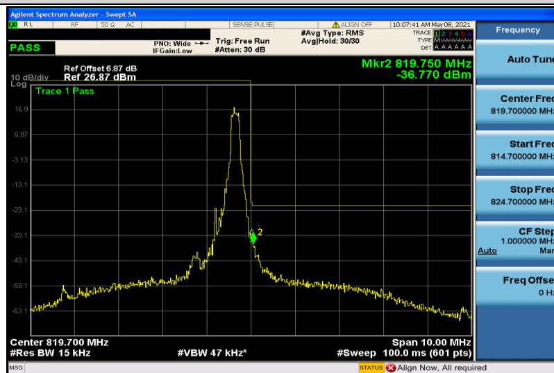
Band26-1.4MHz-QPSK-26740-1RB#5
