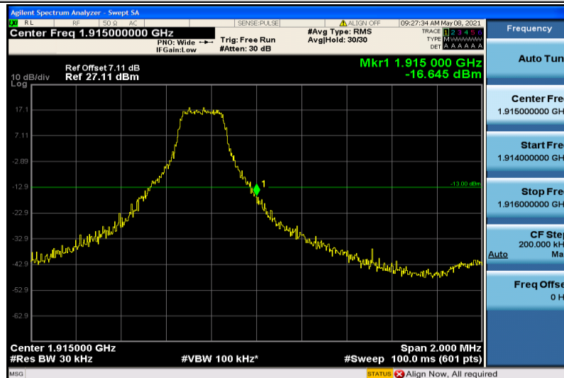
Band25-3MHz-16QAM-26675-1RB#14
