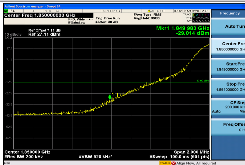
Band25-20MHz-16QAM-26140-1RB#0
