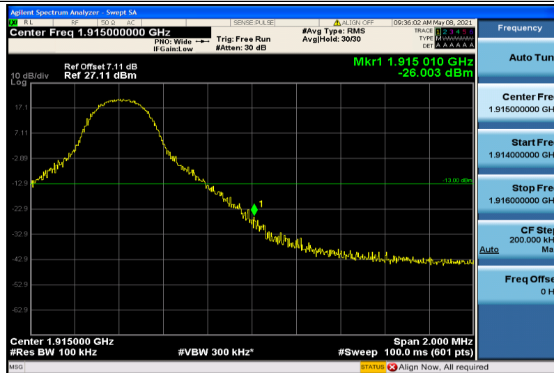
Band25-10MHz-16QAM-26640-1RB#49
