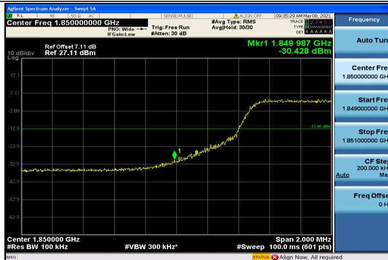
Band25-10MHz-16QAM-26090-50RB#0
