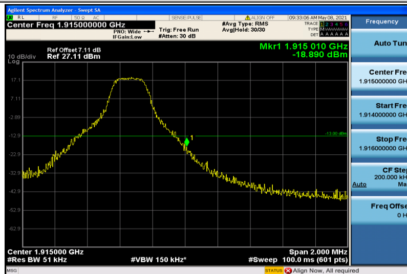
Band25-5MHz-16QAM-26665-1RB#24
