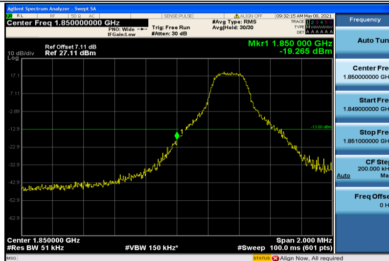
Band25-5MHz-16QAM-26065-1RB#0
