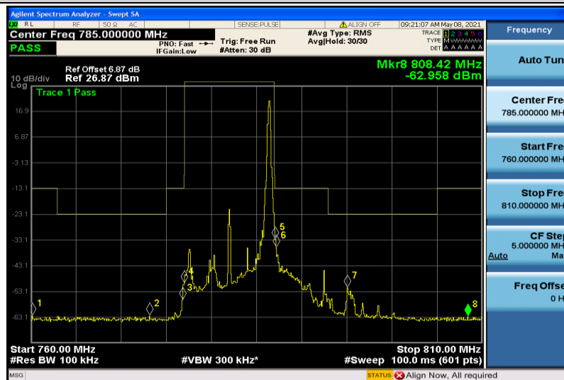
Band13-10MHz-16QAM-23230-1RB#49
