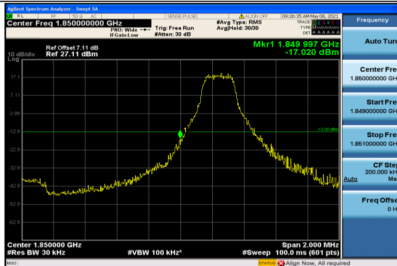
Band25-3MHz-QPSK-26055-1RB#0
