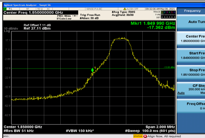
Band25-5MHz-QPSK-26065-1RB#0
