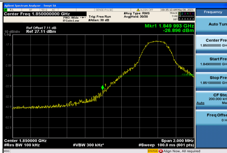
Band25-10MHz-16QAM-26090-1RB#0
