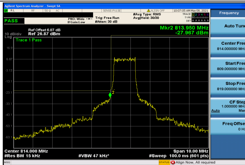
Band26-1.4MHz-QPSK-26697-6RB#0
