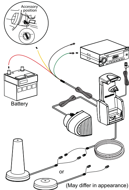
Globalstar Installation Kit Standard Components
