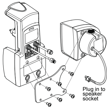
Globalstar Installation Kit Speaker Attachment
