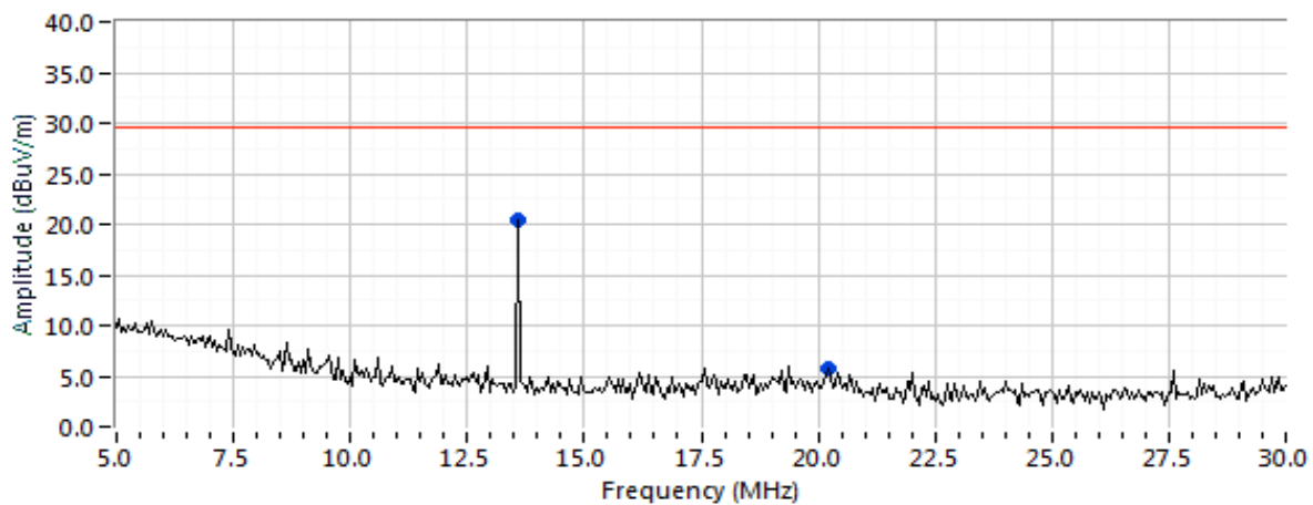
EUT Side, Open
