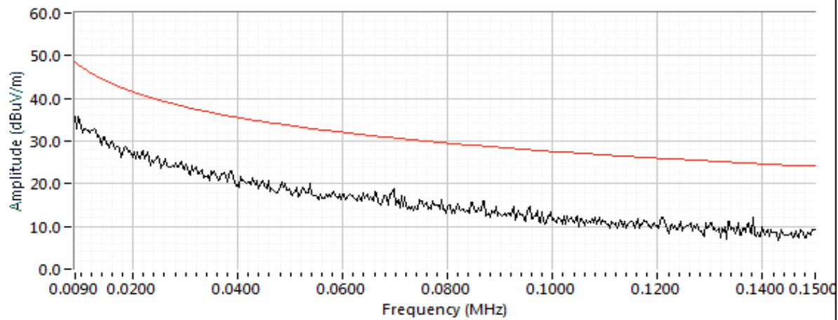
EUT Side, Open
