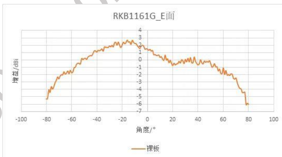
Antenna Radiation Pattern Measurement Data
