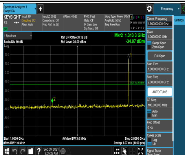
Band2-1.4MHz-QPSK-18900-1RB#0-Range4:1000~2000MHz
