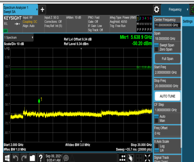
Band2-1.4MHz-QPSK-18900-1RB#0-Range5:2000~20000MHz
