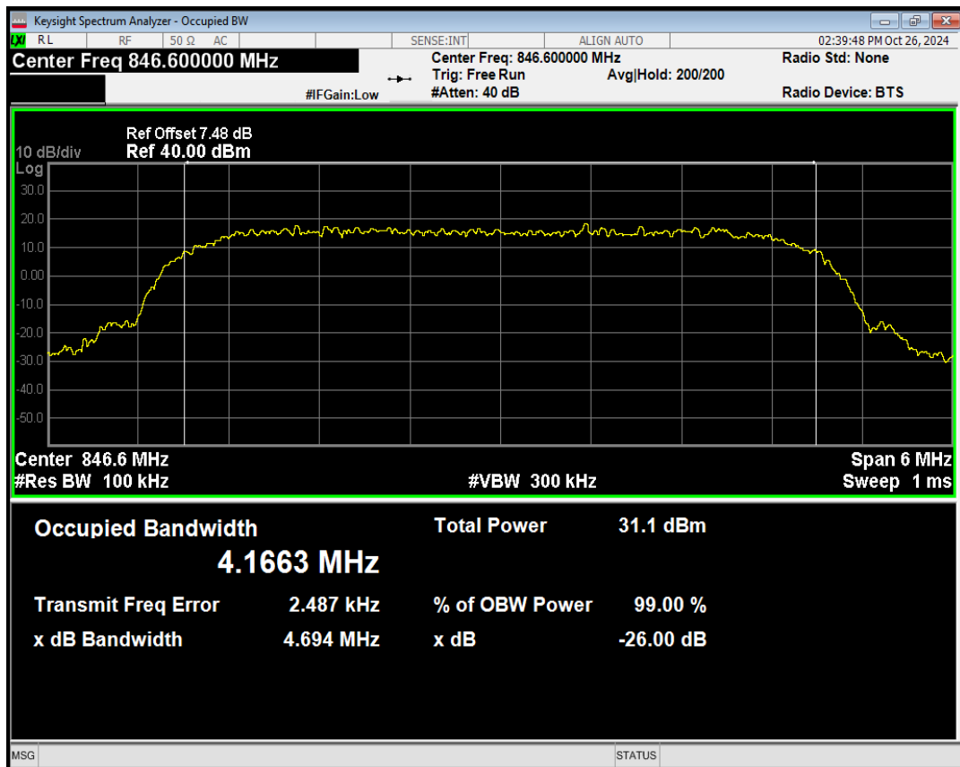
WCDMA Band5 HSUPA Channel=4233
