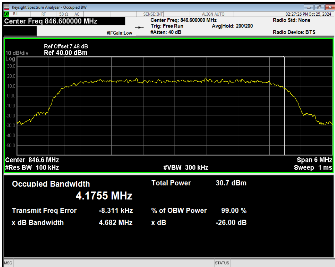
WCDMA Band5 RMC Channel=4233
