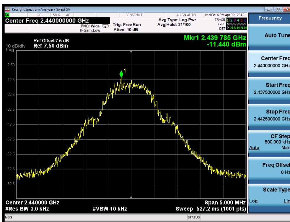
Mode 1 CH19(2440MHz)
