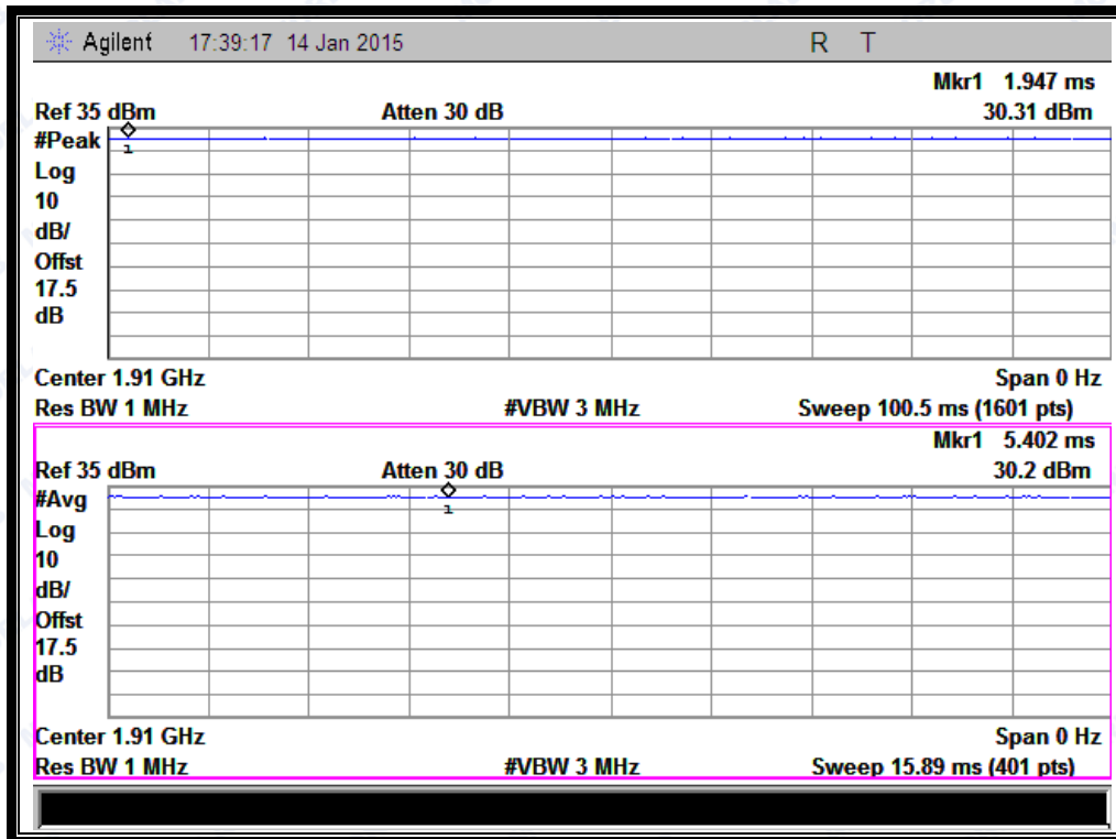
(Plot A3: GPRS 1900MHz Channel = 810)
