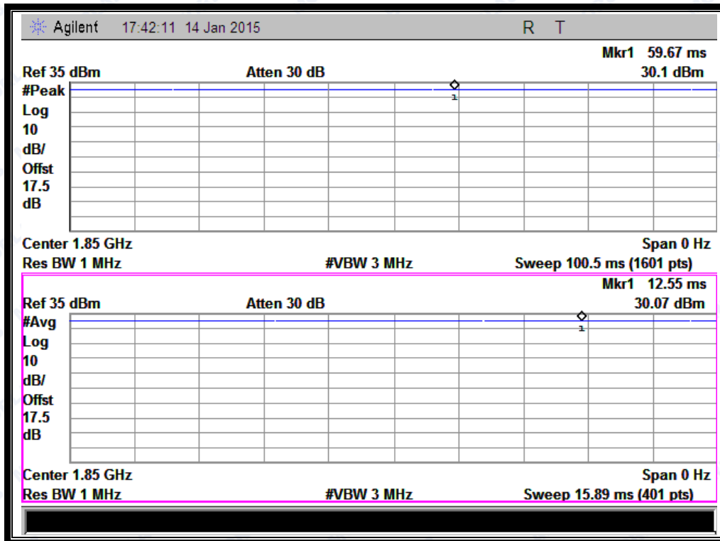
(Plot A1: GPRS 1900 MHz Channel = 512)
