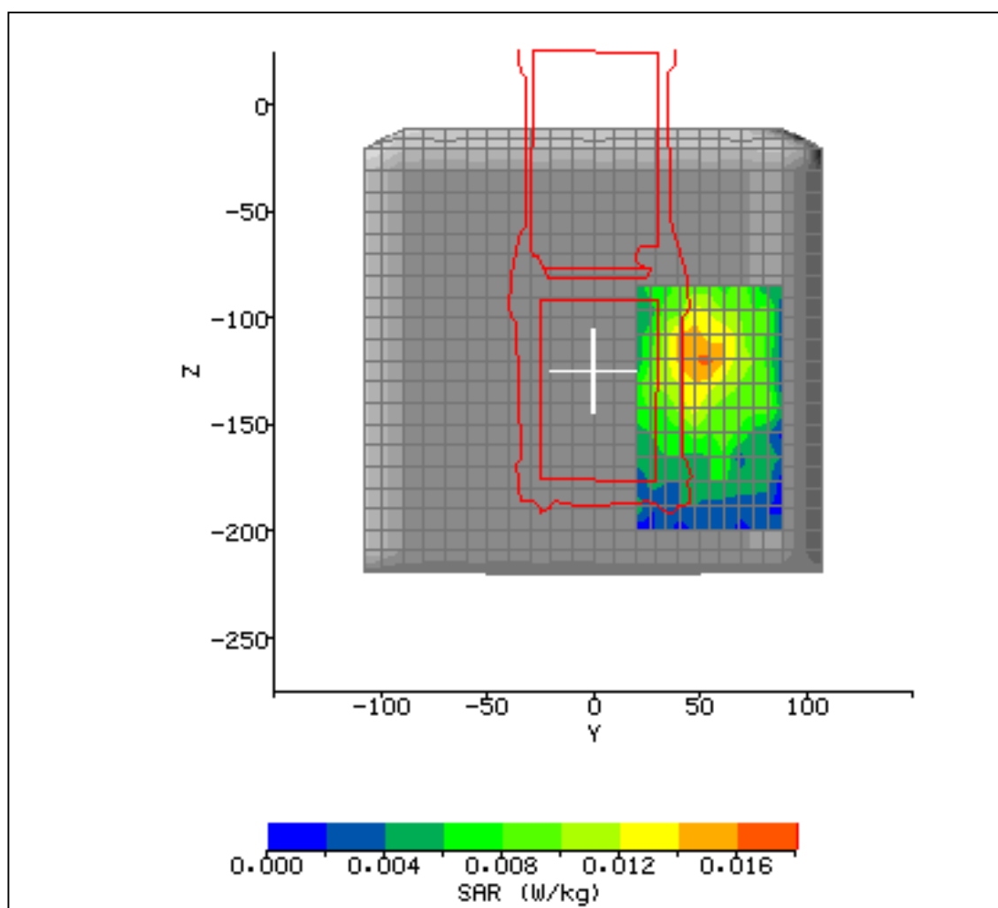
Figure 9 – Second High Energy Area, Bluetooth Radio
