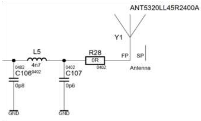
Component Value R28 Resistance 0Ω C106 Capacitor Murata 0.8 pF C107 Capacitor Yageo 0.6 pF L5 Inductor Yageo 4.7 nH
