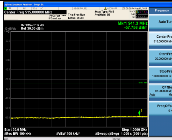
Band7_5MHz_16QAM_20775_1RB#0_30~1000_30~1000
