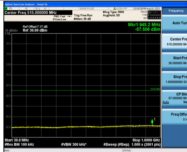
Band7_20MHz_QPSK_21350_1RB#0_30~1000_30~1000
