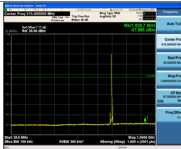
Band17_5MHz_QPSK_23755_1RB#0_30~1000_30~1000
