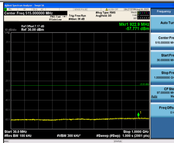
Band7_10MHz_QPSK_21100_1RB#0_30~1000_30~1000
