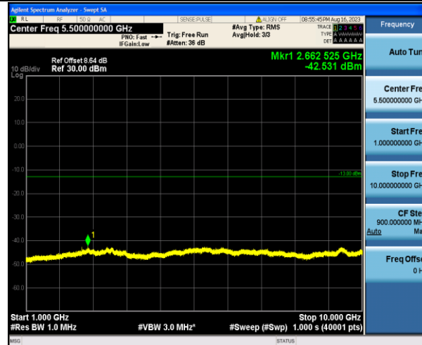
Band5_10MHz_16QAM_20525_1RB#0_1000~10000_1000~10000
