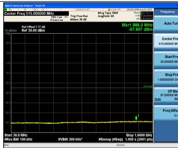
Band7_10MHz_16QAM_21100_1RB#0_30~1000_30~1000
