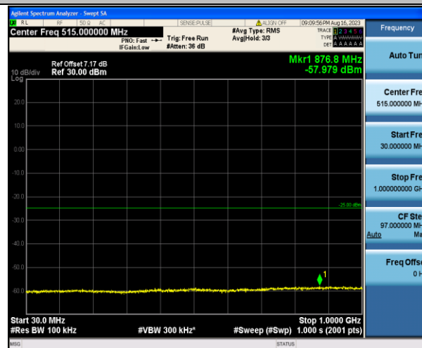
Band7_5MHz_QPSK_21100_1RB#0_30~1000_30~1000
