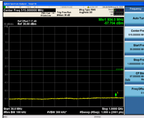
Band7_10MHz_QPSK_21400_1RB#0_30~1000_30~1000
