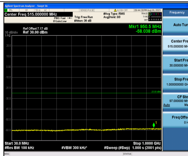
Band7_15MHz_QPSK_20825_1RB#0_30~1000_30~1000
