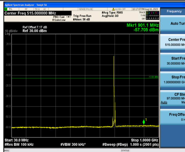
Band17_5MHz_16QAM_23755_1RB#0_30~1000_30~1000
