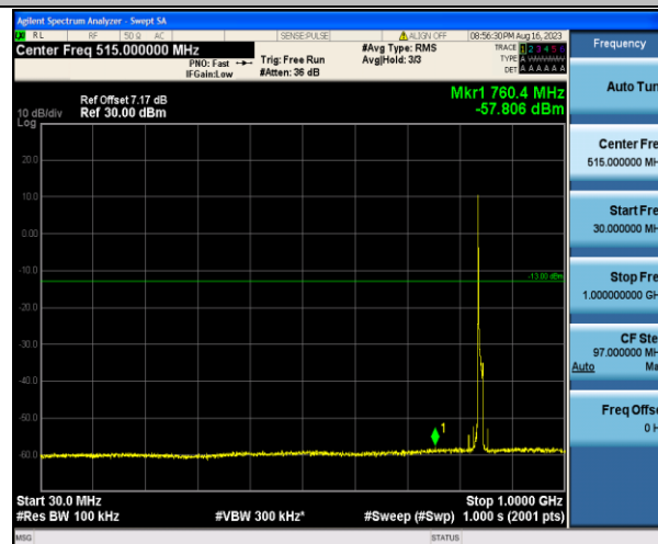
Band5_10MHz_16QAM_20600_1RB#0_30~1000_30~1000
