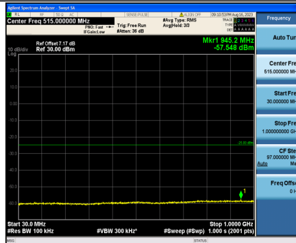
Band7_5MHz_QPSK_21425_1RB#0_30~1000_30~1000
