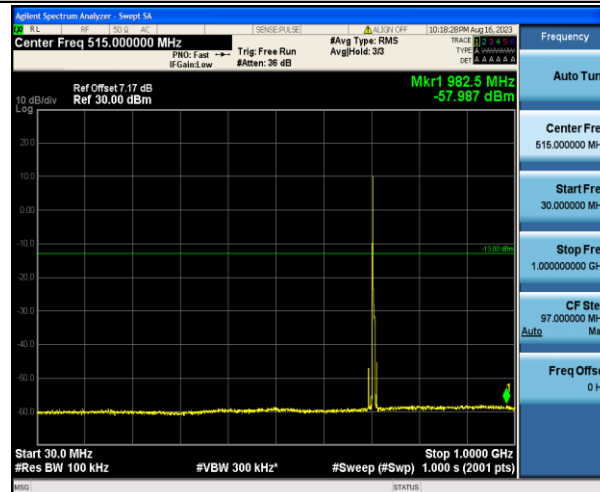
Band17_5MHz_QPSK_23825_1RB#0_30~1000_30~1000
