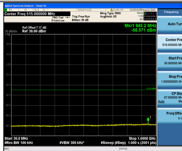
Band7_20MHz_QPSK_21100_1RB#0_30~1000_30~1000
