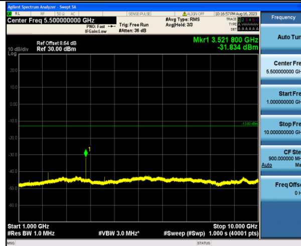
Band17_5MHz_QPSK_23755_1RB#0_1000~10000_1000~10000
