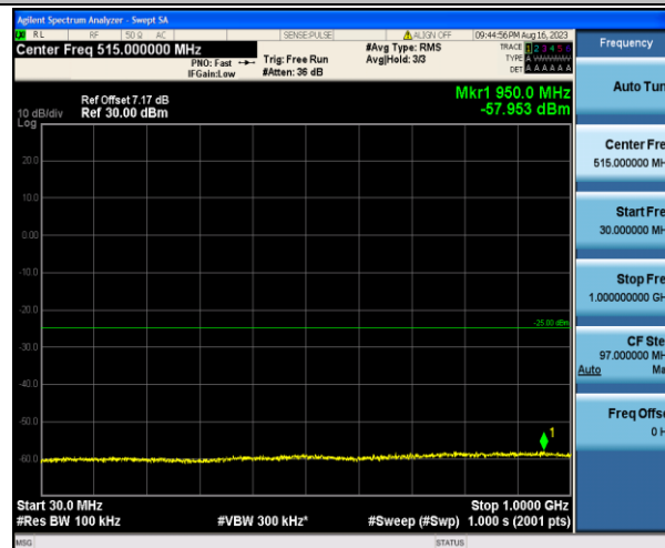
Band7_15MHz_16QAM_20825_1RB#0_30~1000_30~1000
