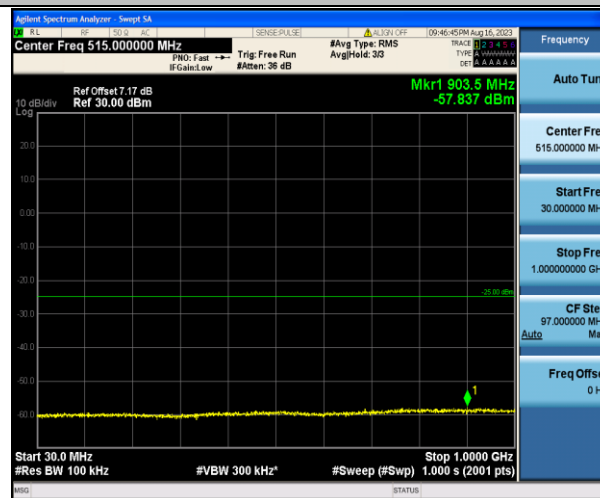
Band7_15MHz_16QAM_21375_1RB#0_30~1000_30~1000
