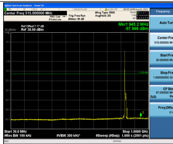
Band5_10MHz_16QAM_20525_1RB#0_30~1000_30~1000
