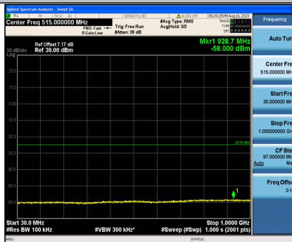
Band7_10MHz_16QAM_21400_1RB#0_30~1000_30~1000
