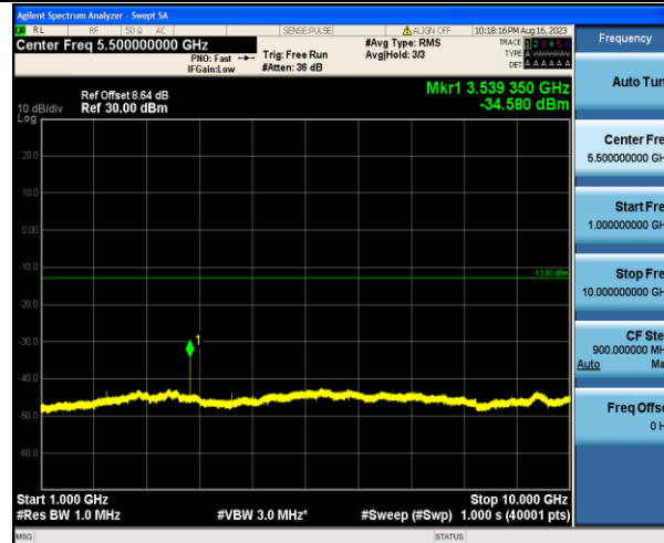
Band17_5MHz_16QAM_23790_1RB#0_1000~10000_1000~10000
