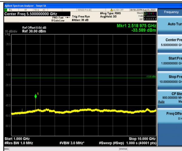
Band5_10MHz_QPSK_20600_1RB#0_1000~10000_1000~10000
