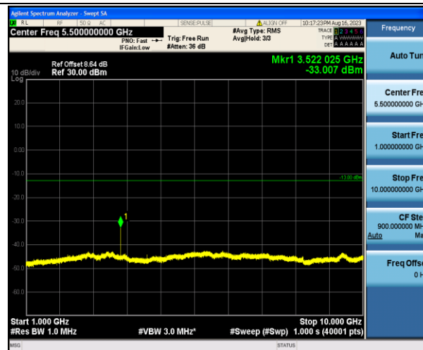
Band17_5MHz_16QAM_23755_1RB#0_1000~10000_1000~10000
