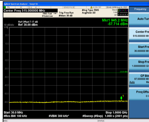
Band7_15MHz_QPSK_21375_1RB#0_30~1000_30~1000
