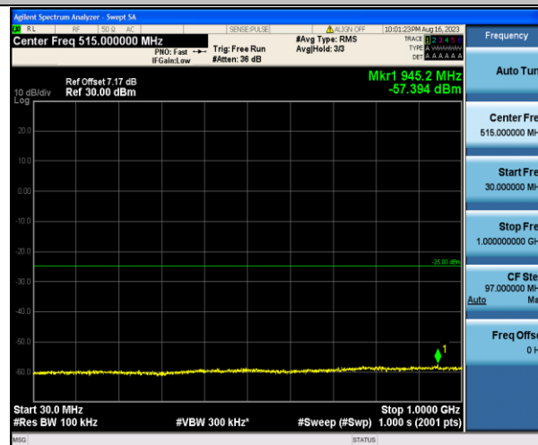
Band7_20MHz_16QAM_21350_1RB#0_30~1000_30~1000
