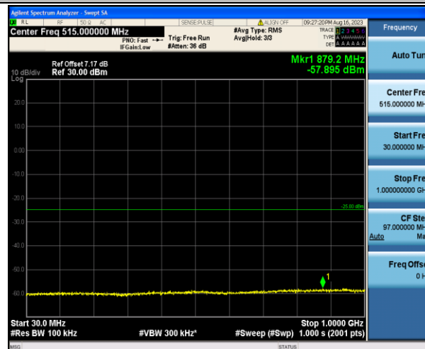
Band7_10MHz_16QAM_20800_1RB#0_30~1000_30~1000
