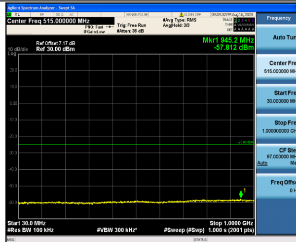
Band7_20MHz_16QAM_20850_1RB#0_30~1000_30~1000
