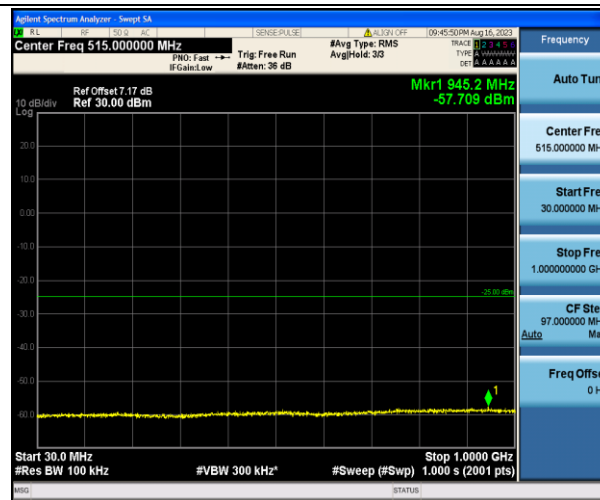
Band7_15MHz_16QAM_21100_1RB#0_30~1000_30~1000
