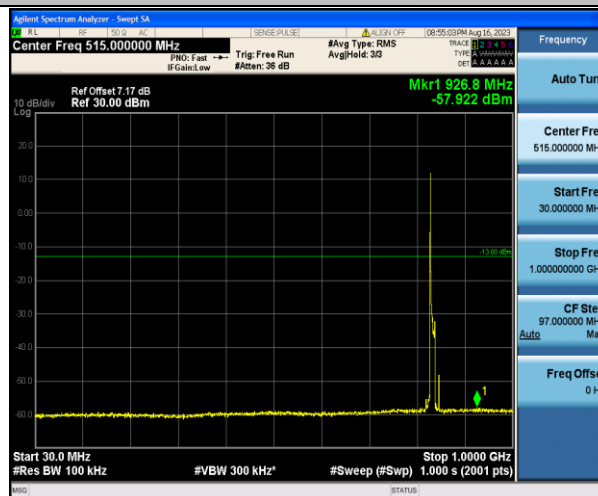
Band5_10MHz_QPSK_20525_1RB#0_30~1000_30~1000
