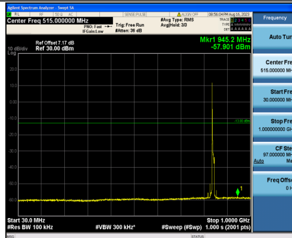
Band5_10MHz_QPSK_20600_1RB#0_30~1000_30~1000
