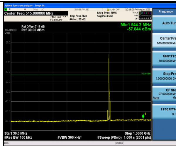
Band17_5MHz_16QAM_23790_1RB#0_30~1000_30~1000
