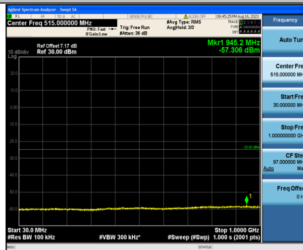
Band7_15MHz_QPSK_21100_1RB#0_30~1000_30~1000
