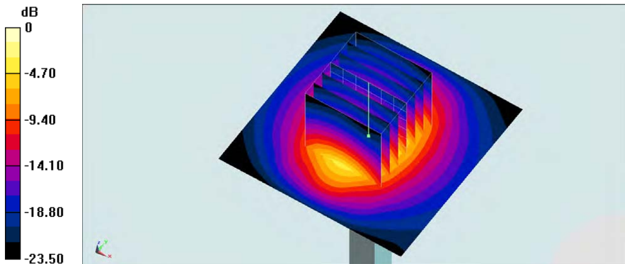
System Performance Check 2600MHz Head250mW
