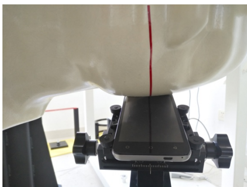
Left Head Tilt (15°)
