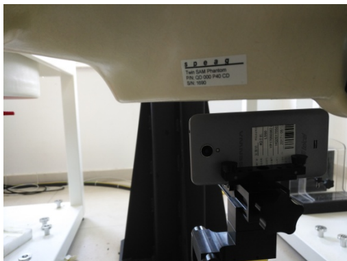
Hotspot mode - Left Side (10mm)
