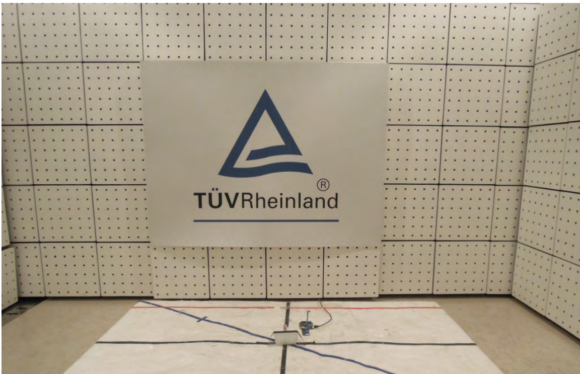
Photograph 13: Set-up for Spurious Emissions (Front View 1) - RFPCA381013IMAB701-ANT
