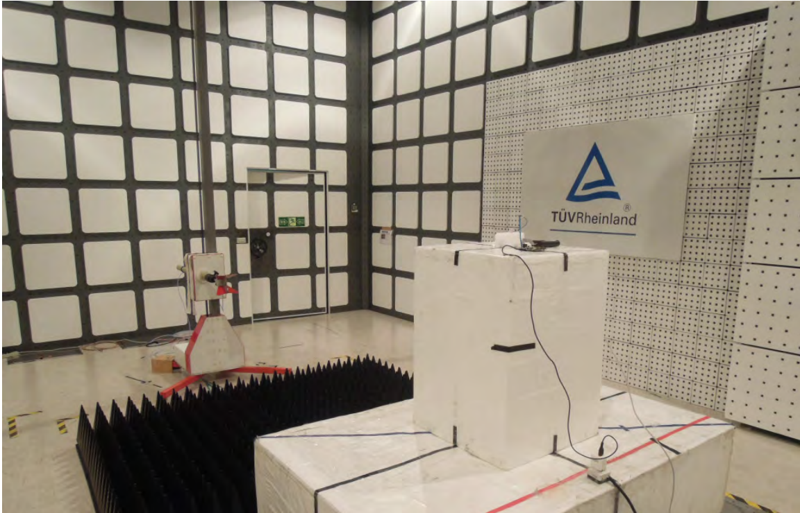
Photograph 11: Set-up for Spurious Emissions (Back View 3) - RFMTA331215IMAB701-ANT
