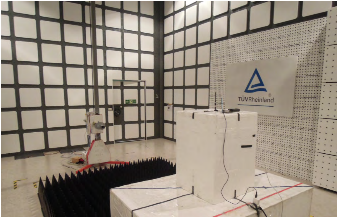
Photograph 7: Set-up for Spurious Emissions (Front view 1) - RFMTA331215IMAB701-ANT
