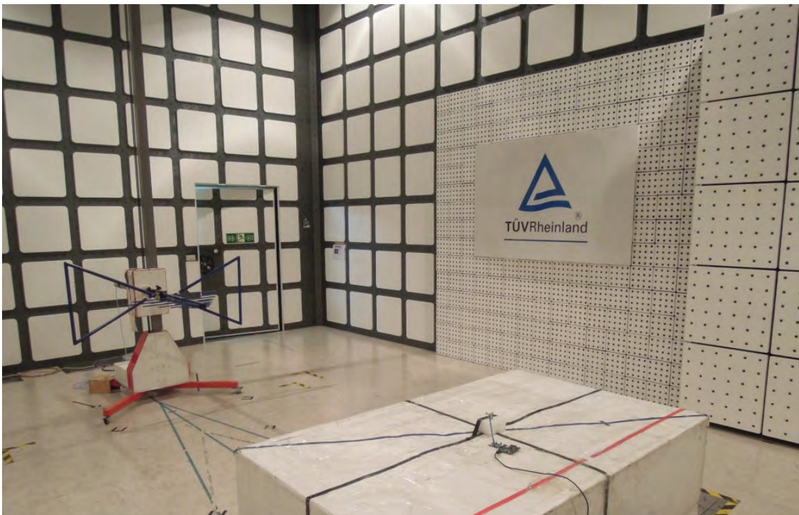
Photograph 15: Set-up for Spurious Emissions (Back View 1) - RFPCA381013IMAB701-ANT
