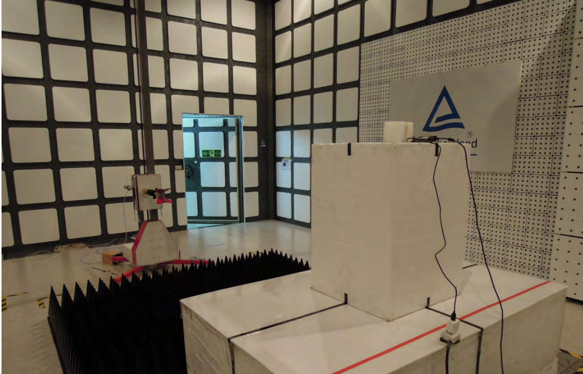
Photograph 25: Set-up for Spurious Emissions (Front View)- ACC-RN-SMA-S-DS -ANT
