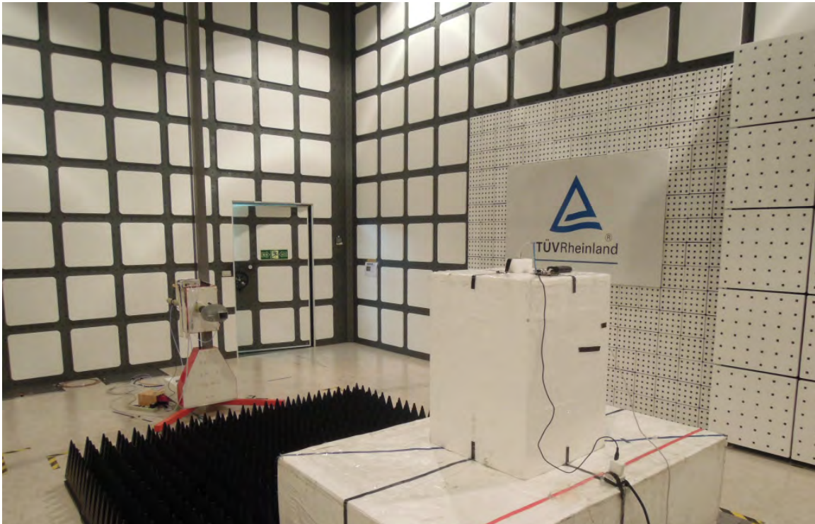
Photograph 19: Set-up for Spurious Emissions (Front View)- RFDPA870920IMLB301-ANT
