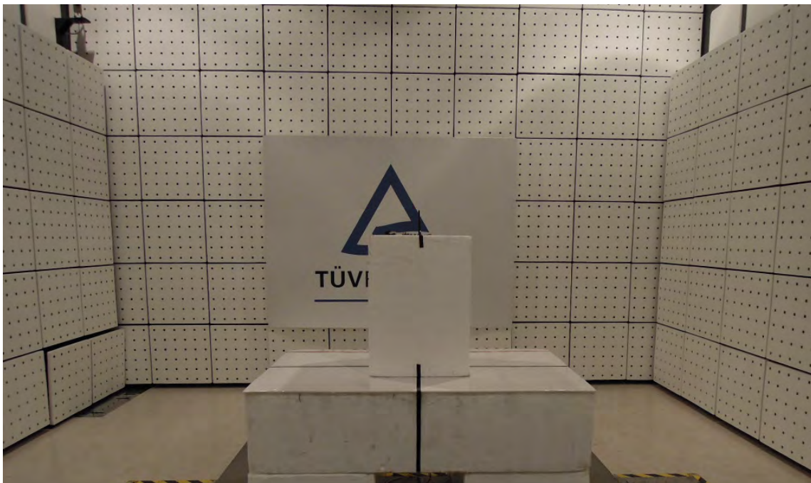
Photograph 21: Set-up for Spurious Emissions (Front View)- RFA-02-3-C5H1 -ANT
