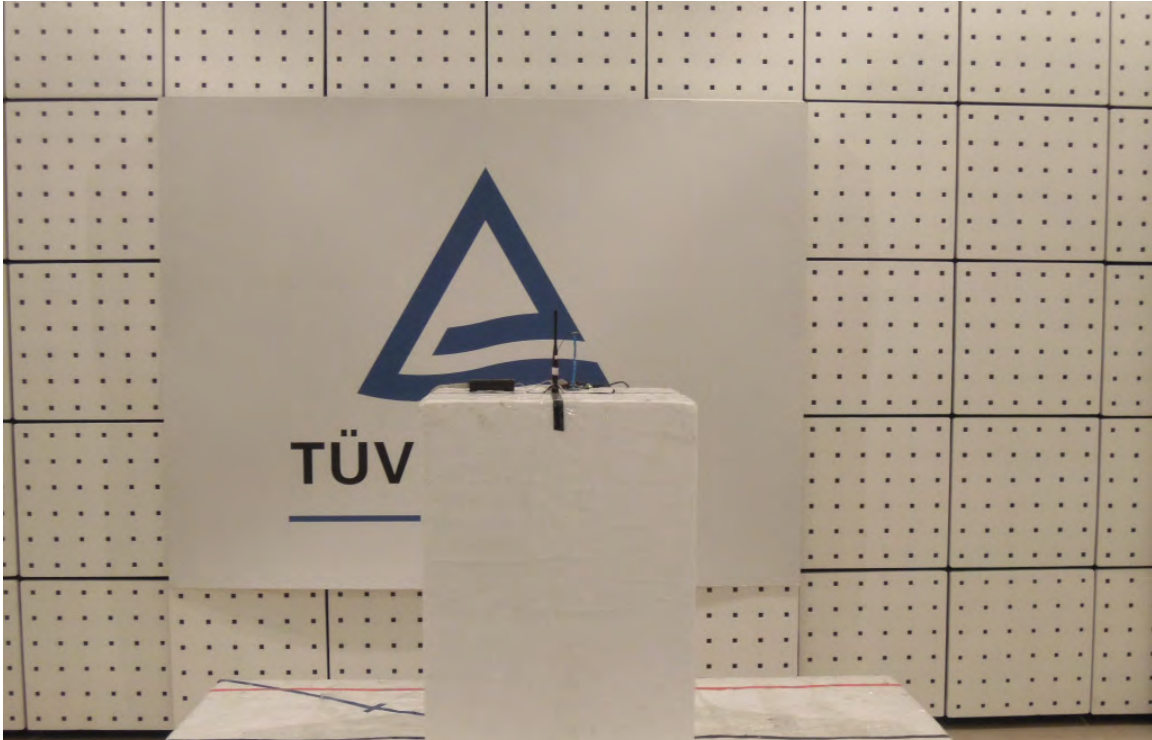
Photograph 3: Set-up for Spurious Emissions (Back View 1) - RFA-02-5-C7H1-ANT
