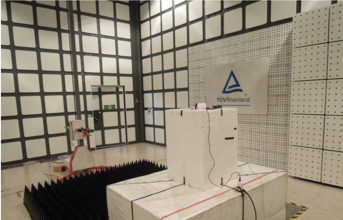
Photograph 17: Set-up for Spurious Emissions (Back View 3) - RFPCA381013IMAB701-ANT
