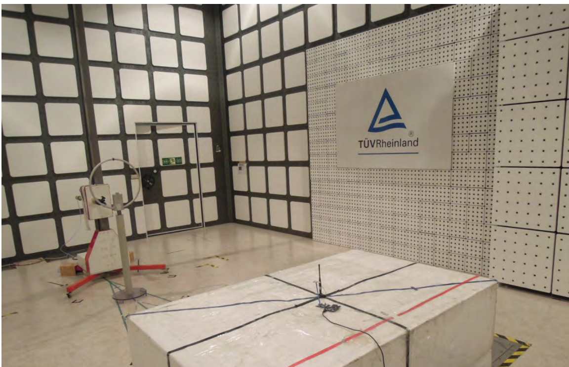
Photograph 5: Set-up for Spurious Emissions (Back View 3) - RFA-02-5-C7H1-ANT
