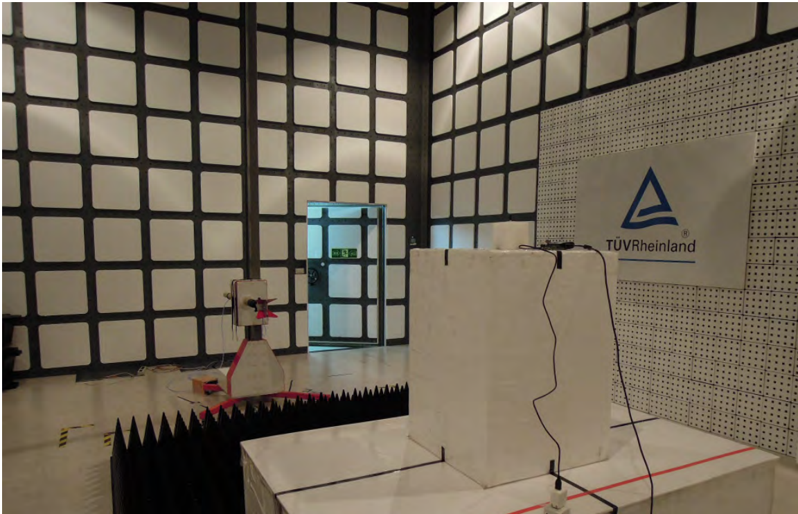
Photograph 27: Set-up for Spurious Emissions (Front View)- W3525B039-ANT
