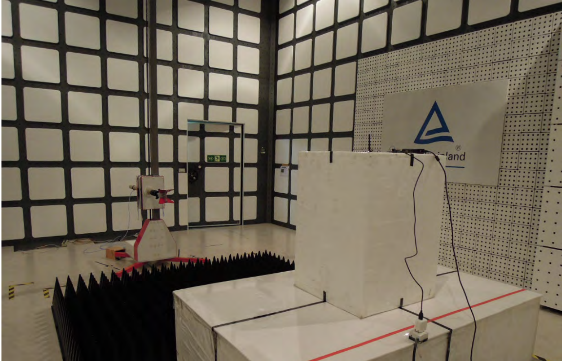
Photograph 20: Set-up for Spurious Emissions (Back View)- RFDPA870920IMLB301-ANT
