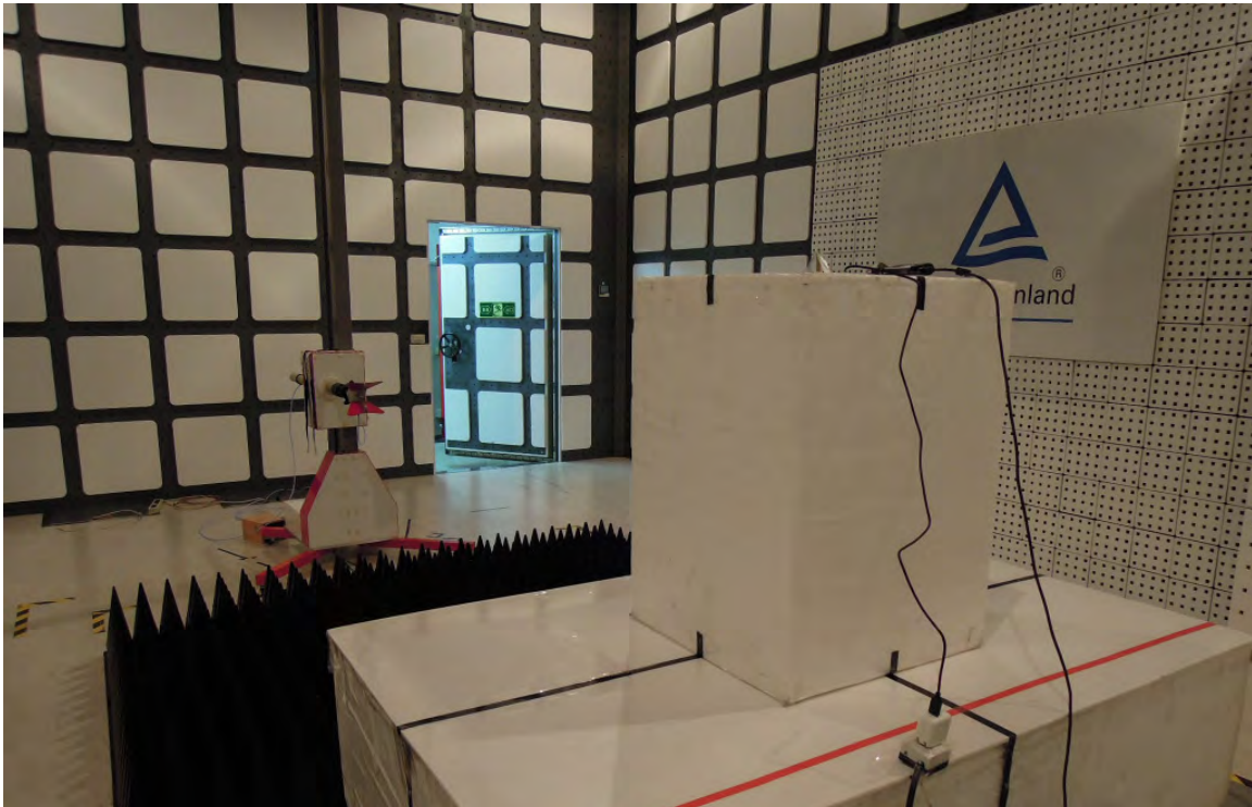
Photograph 28: Set-up for Spurious Emissions (Back View)- W3525B039-ANT
