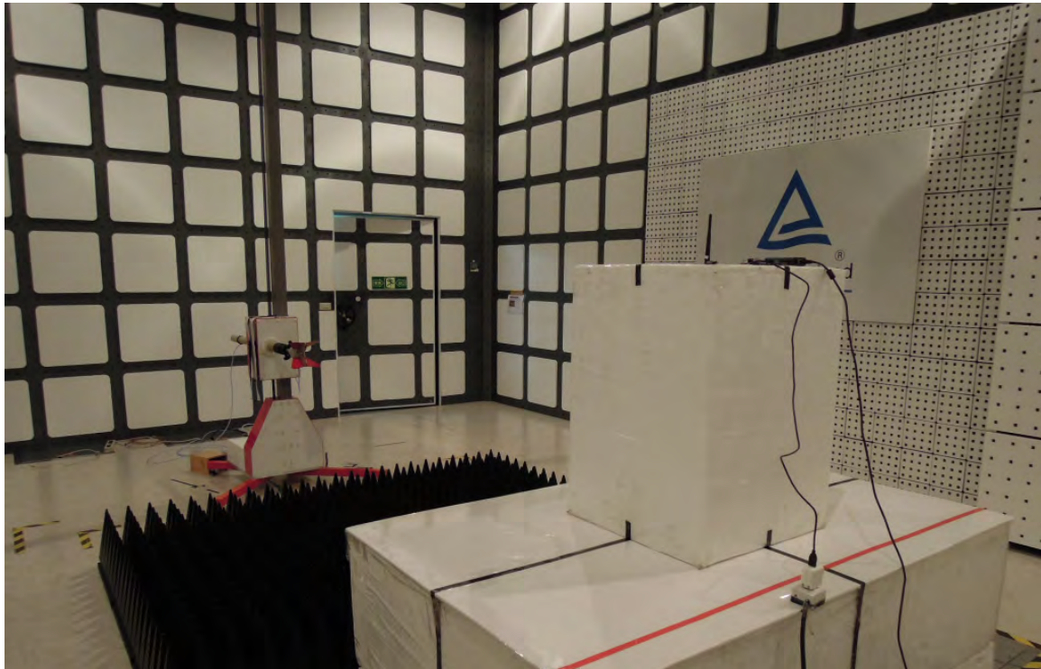
Photograph 22: Set-up for Spurious Emissions (Back View)- RFA-02-3-C5H1 -ANT
