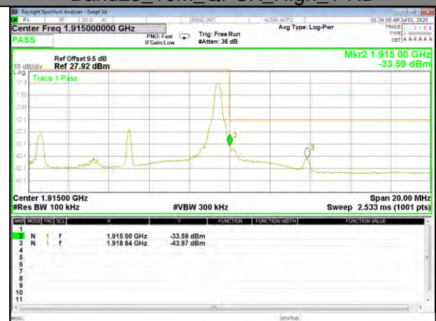
Band25_10M_QPSK_High_1-RB
