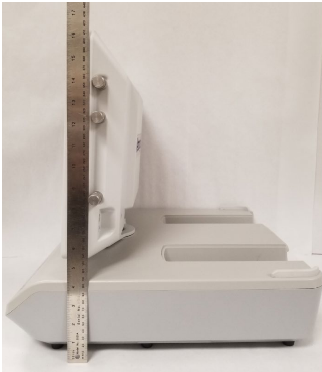
Figure 6 NIM Vital Console, Model NIM4CM01, Right Side View (Height) with dimensions
