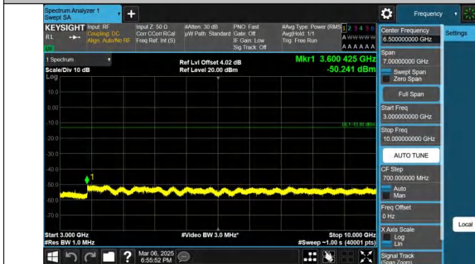
Band26(824-849)-10MHz-QPSK-26915-1RB#0-3000~10000-PASS S
