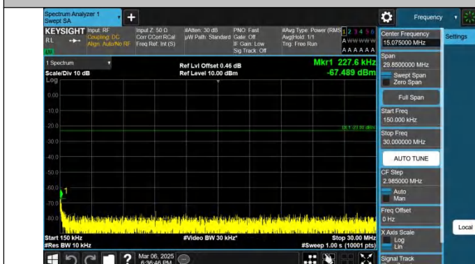
Band26(824-849)-1.4MHz-QPSK-27033-1RB#5-0.15~30-PASS
