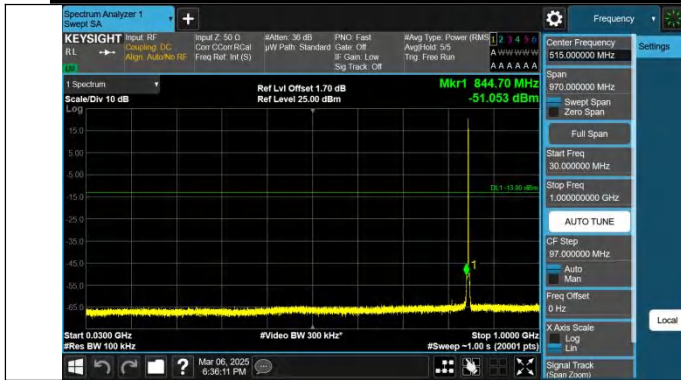
Band26(824-849)-1.4MHz-QPSK-27033-1RB#0-30~1000-PASS
