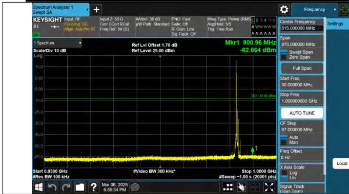
Band26(824-849)-10MHz-QPSK-26915-1RB#0-30~1000-PASS
