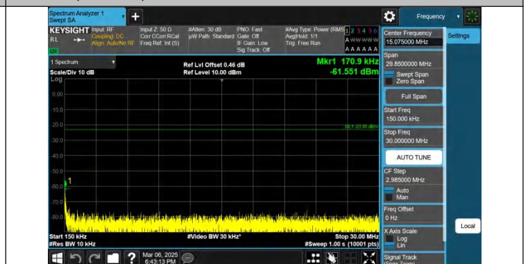
Band26(824-849)-3MHz-QPSK-27025-1RB#0-0.15~30-PASS
