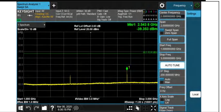
Band26(824-849)-1.4MHz-QPSK-27033-1RB#0-1000~3000-PASS
