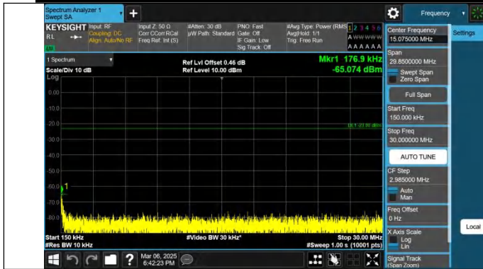
Band26(824-849)-3MHz-QPSK-26915-1RB#14-0.15~30-PASS
