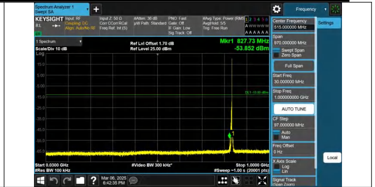
Band26(824-849)-3MHz-QPSK-26915-1RB#14-30~1000-PASS
