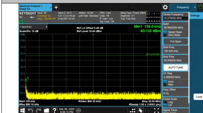
Band26(824-849)-10MHz-QPSK-26915-1RB#49-0.15~30-PASS
