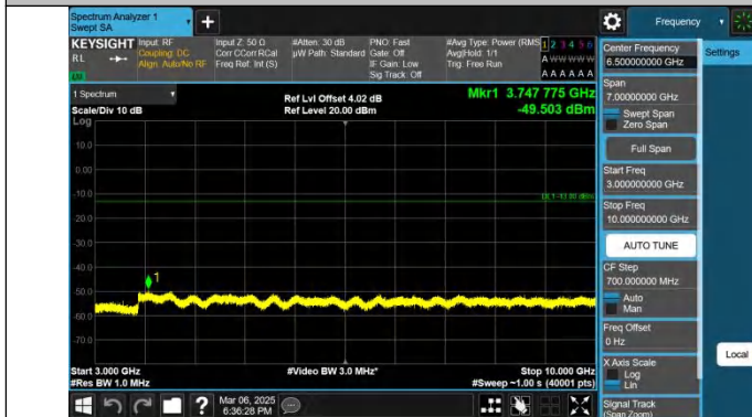
Band26(824-849)-1.4MHz-QPSK-27033-1RB#0-3000~10000-PASS S
