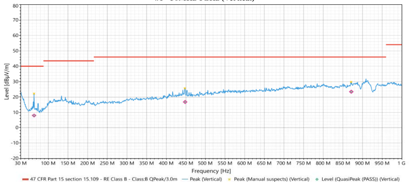
#1 - 30MHz-1GHz (Vertical)
