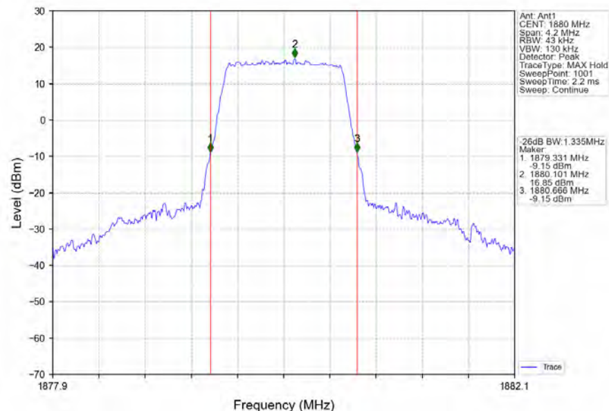
Band2_1.4MHz_64QAM_MCH_1880MHz_RB_6_0_NTNV
