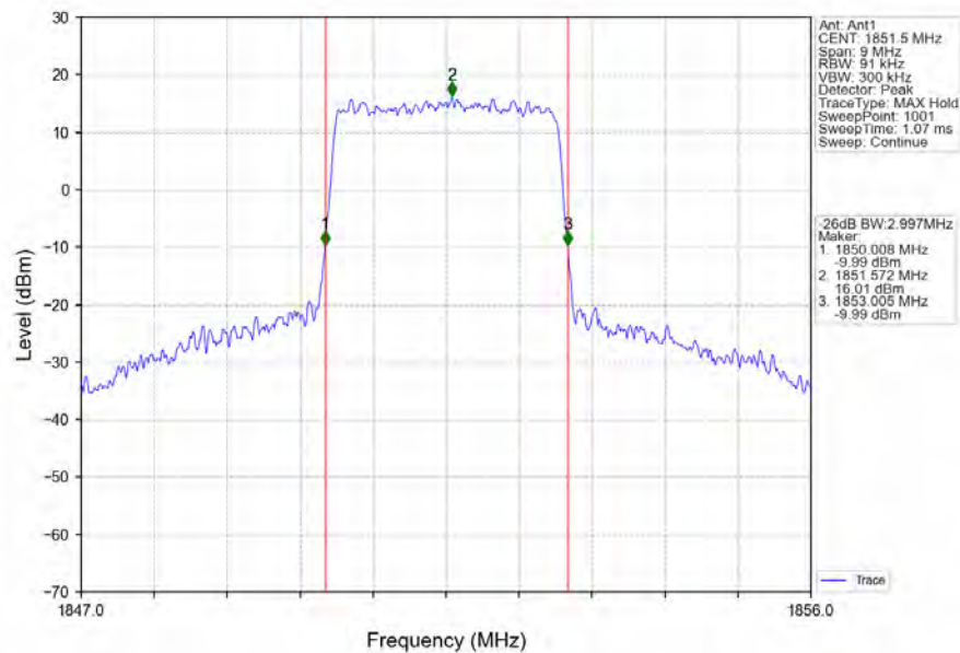
Band2_3MHz_64QAM_LCH_1851.5MHz_RB_15_0_NTNV
