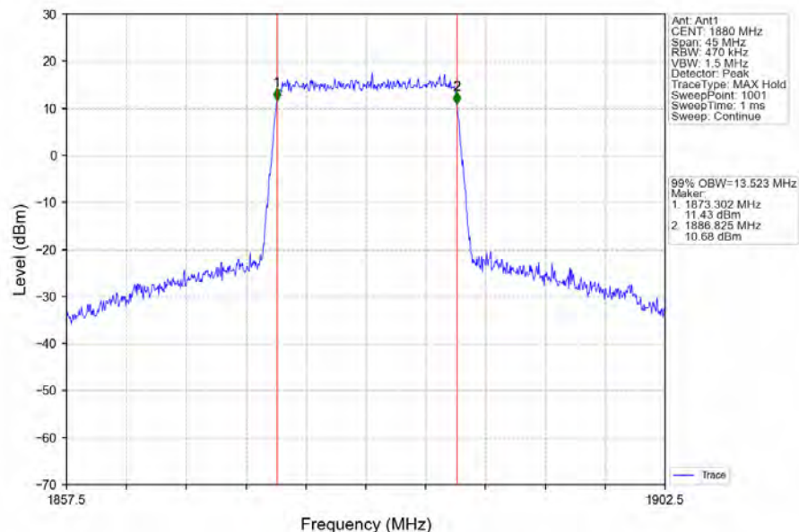
Band2_15MHz_64QAM_MCH_1880MHz_RB_75_0_NTNV
