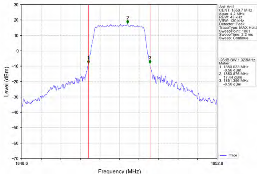
Band2_1.4MHz_16QAM_LCH_1850.7MHz_RB_6_0_NTNV
