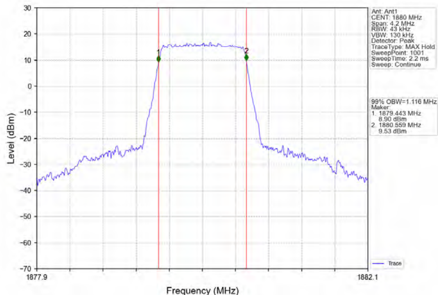
Band2_1.4MHz_64QAM_MCH_1880MHz_RB_6_0_NTNV
