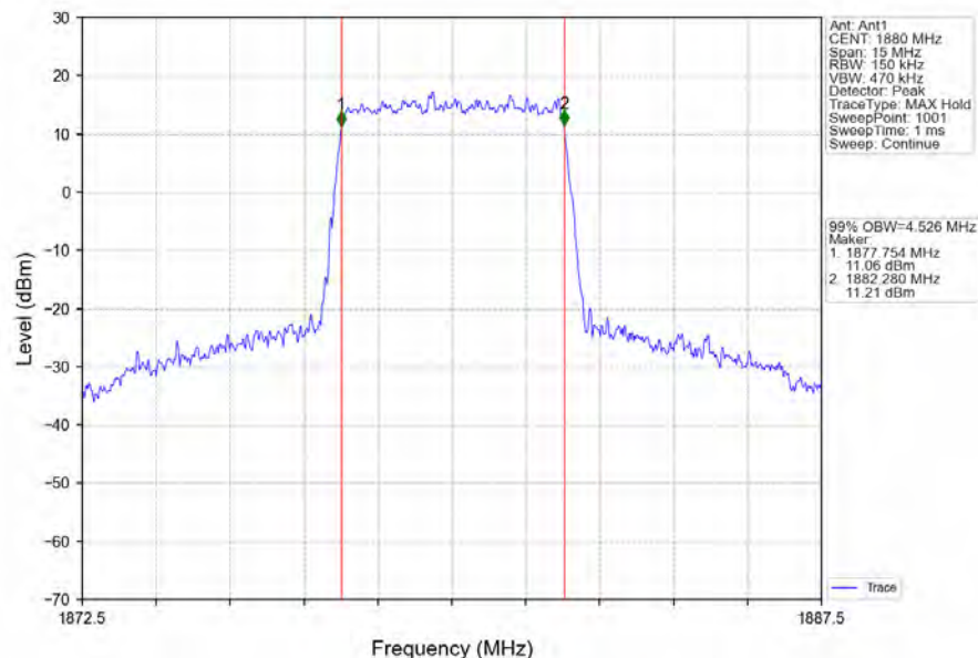
Band2_5MHz_64QAM_MCH_1880MHz_RB_25_0_NTNV
