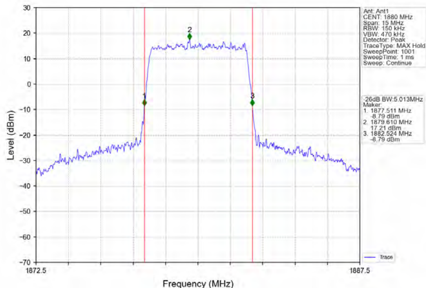
Band2_5MHz_64QAM_MCH_1880MHz_RB_25_0_NTNV
