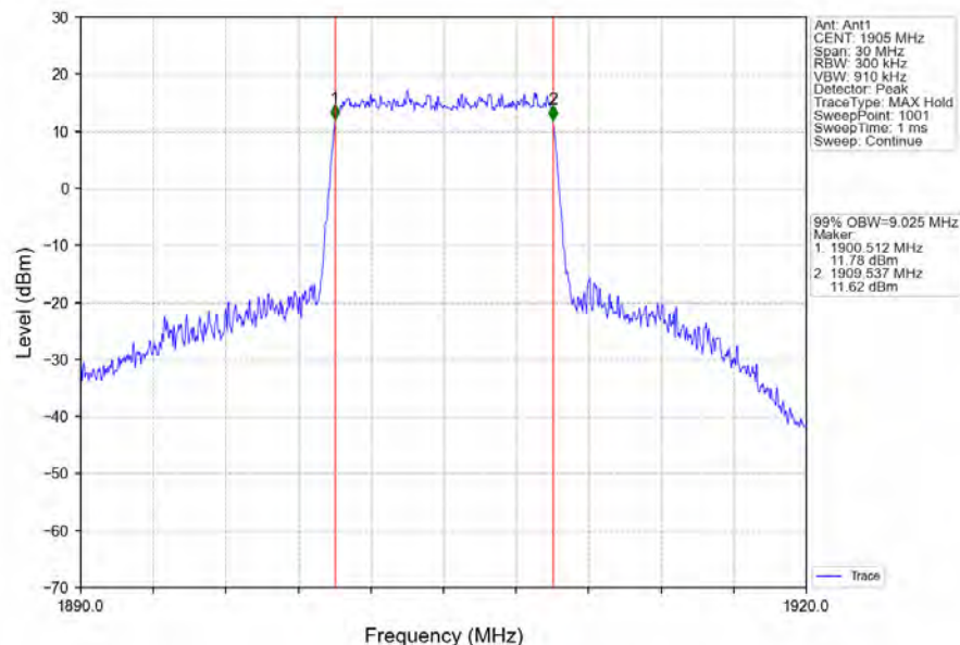
Band2_10MHz_64QAM_HCH_1905MHz_RB_50_0_NTNV
