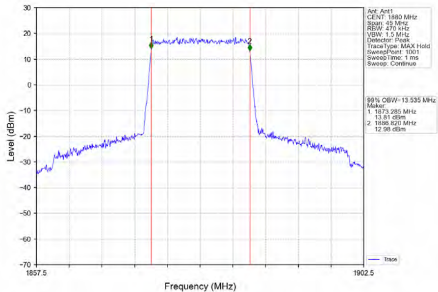
Band2_15MHz_QPSK_MCH_1880MHz_RB_75_0_NTNV
