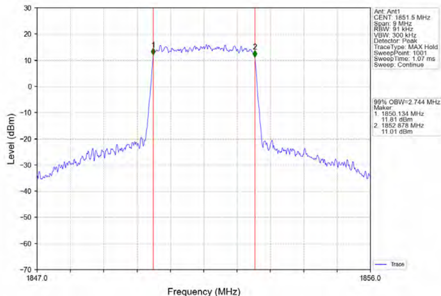
Band2_3MHz_64QAM_LCH_1851.5MHz_RB_15_0_NTNV
