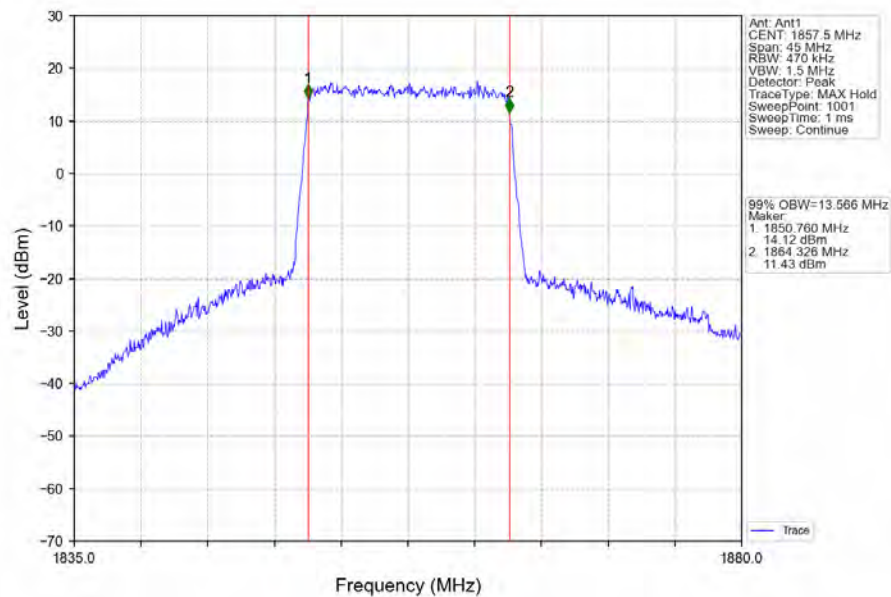
Band2_15MHz_16QAM_LCH_1857.5MHz_RB_75_0_NTNV
