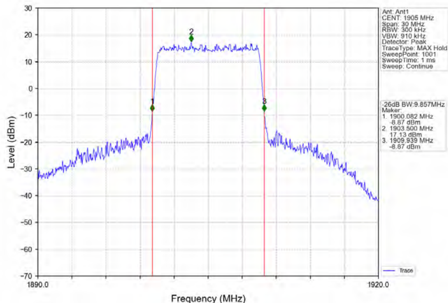
Band2_10MHz_64QAM_HCH_1905MHz_RB_50_0_NTNV
