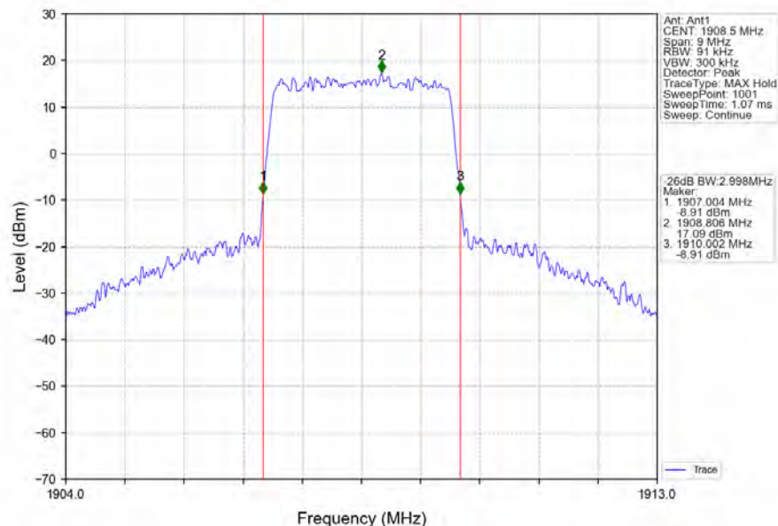
Band2_3MHz_64QAM_HCH_1908.5MHz_RB_15_0_NTNV
