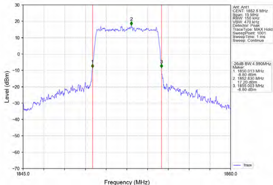
Band2_5MHz_16QAM_LCH_1852.5MHz_RB_25_0_NTNV
