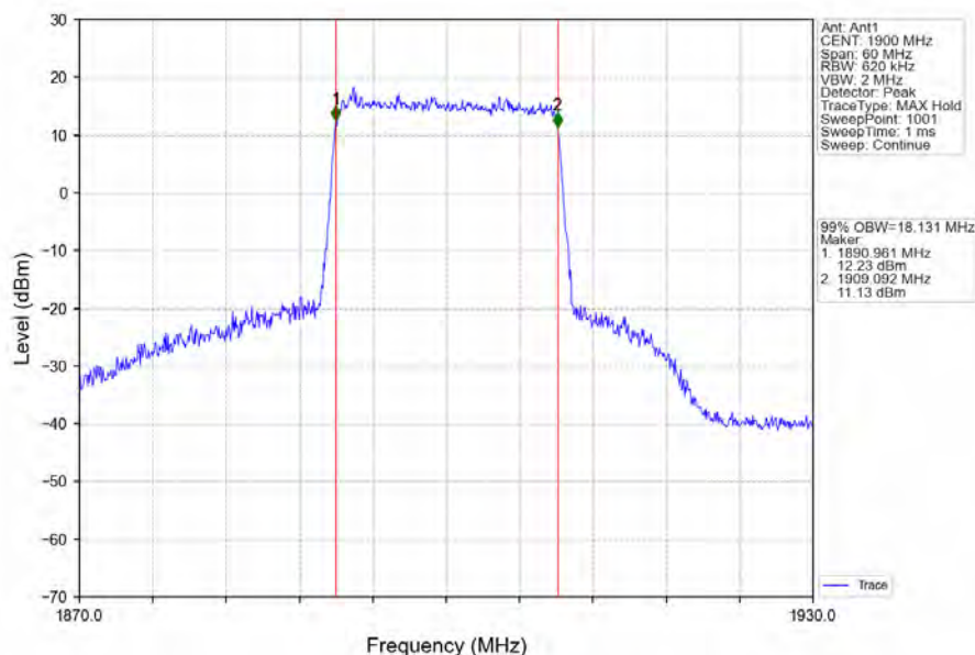
Band2_20MHz_64QAM_HCH_1900MHz_RB_100_0_NTNV
