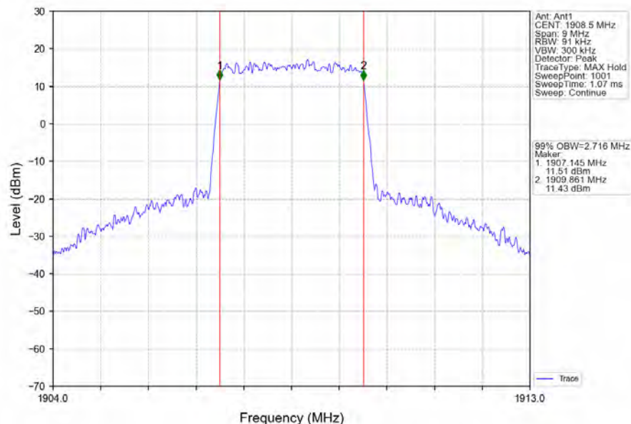
Band2_3MHz_64QAM_HCH_1908.5MHz_RB_15_0_NTNV
