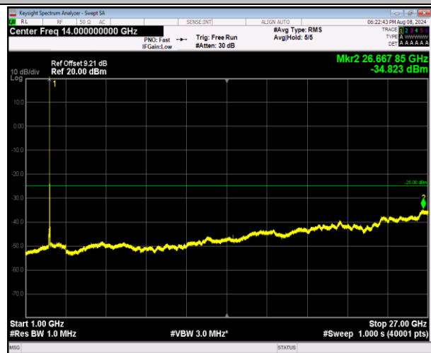
7-7-10MHz-20MHz-QPSK-QPSK-21206-21350-1RB#49-0 RB#0-1000~27000MHz-PASS
