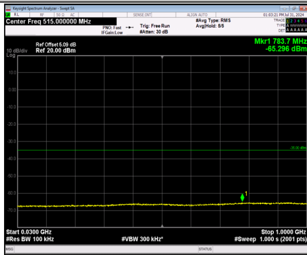
7-7-20MHz-10MHz-64QAM-64QAM-20850-20994-1RB# 99-0RB#0-30~1000MHz-PASS
