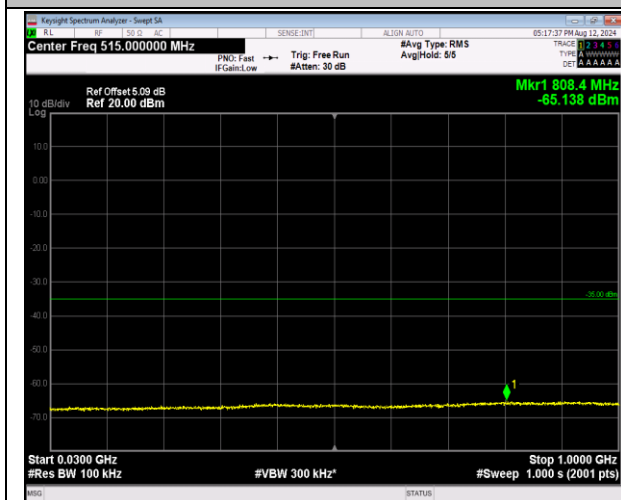
7-7-20MHz-10MHz-16QAM-16QAM-20850-20994-1RB# 0-0RB#0-30~1000MHz-PASS
