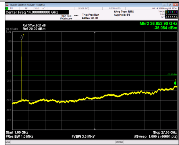
7-7-10MHz-20MHz-16QAM-16QAM-20805-20949-1RB#0-0-1RB#99-1000~27000MHz-PASS
