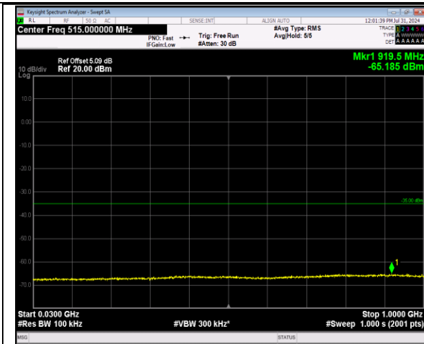
7-7-10MHz-20MHz-64QAM-64QAM-20805-20949-1RB# 0-1RB#99-30~1000MHz-PASS
