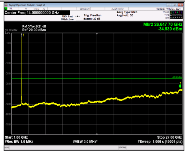
7-7-20MHz-10MHz-64QAM-64QAM-20850-20994-1RB#9 9-0RB#0-1000~27000MHz-PASS
