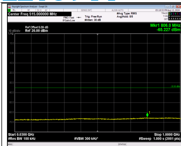
7-7-20MHz-10MHz-16QAM-16QAM-20850-20994-1RB# 99-0RB#0-30~1000MHz-PASS
