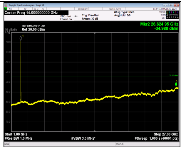
7-7-20MHz-10MHz-64QAM-64QAM-20850-20994-1RB#0 -1RB#49-1000~27000MHz-PASS
