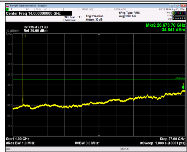
7-7-20MHz-10MHz-16QAM-16QAM-21051-21195-1RB#0-0RB#0-1000~27000MHz-PASS
