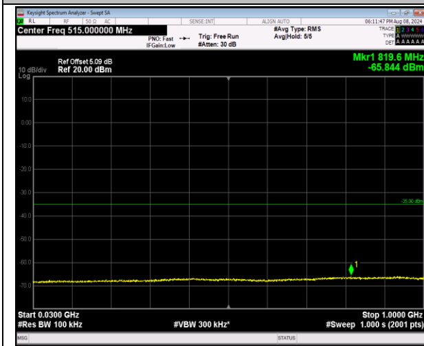
7-7-10MHz-20MHz-16QAM-16QAM-20805-20949-1RB#0-0RB#0-30~1000MHz-PASS
