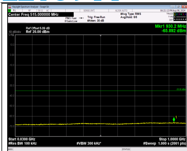
7-7-10MHz-20MHz-QPSK-QPSK-21206-21350-1RB#0-0 RB#0-30~1000MHz-PASS
