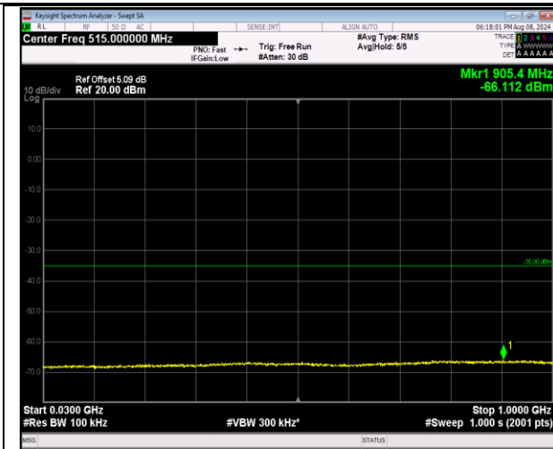
7-7-10MHz-20MHz-16QAM-16QAM-21006-21150-1RB# 49-0RB#0-30~1000MHz-PASS
