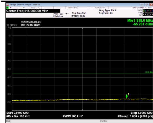
7-7-10MHz-20MHz-64QAM-64QAM-21206-21350-1RB# 0-0RB#0-30~1000MHz-PASS
