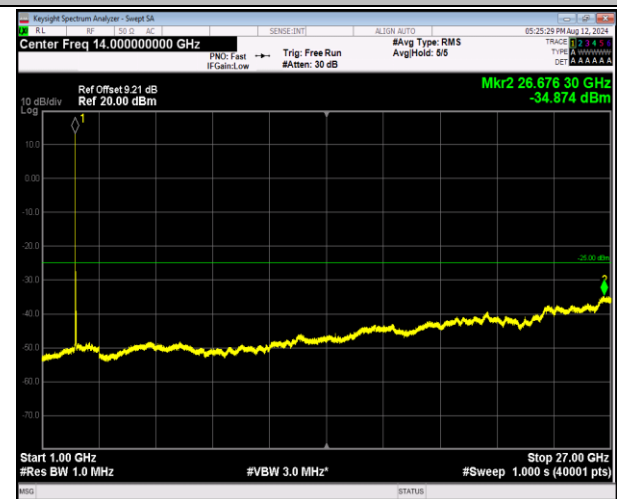
7-7-20MHz-10MHz-16QAM-16QAM-21051-21195-1RB#0-0-1RB#49-1000~27000MHz-PASS
