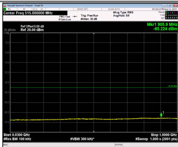
7-7-20MHz-10MHz-QPSK-QPSK-20850-20994-1RB#99-0 ORB#0-30~1000MHz-PASS
