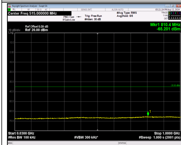
7-7-20MHz-10MHz-16QAM-16QAM-20850-20994-100R B#0-50RB#0-30~1000MHz-PASS
