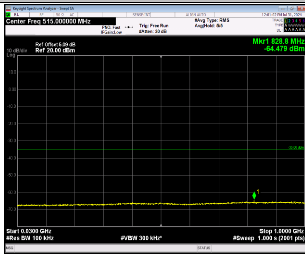
7-7-10MHz-20MHz-64QAM-64QAM-20805-20949-1RB# 49-0RB#0-30~1000MHz-PASS
