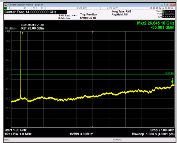
7-7-10MHz-20MHz-64QAM-64QAM-20805-20949-1RB#4 9-0RB#0-1000~27000MHz-PASS
