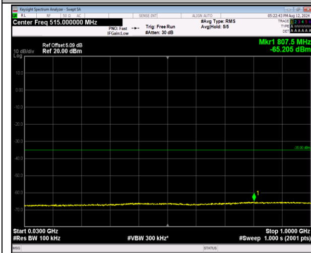
7-7-20MHz-10MHz-16QAM-16QAM-21051-21195-1RB#0-0RB#0-30~1000MHz-PASS
