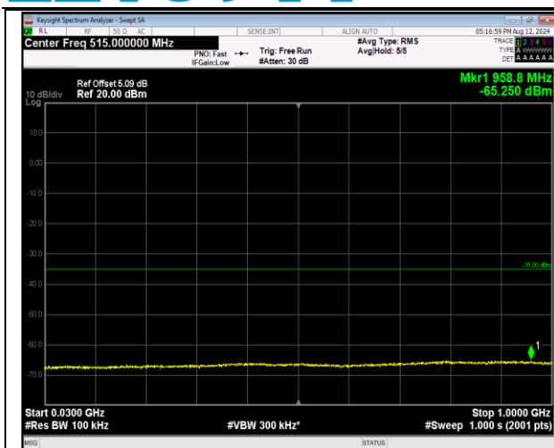
7-7-20MHz-10MHz-QPSK-QPSK-20850-20994-1RB#0-0 RB#0-30~1000MHz-PASS
