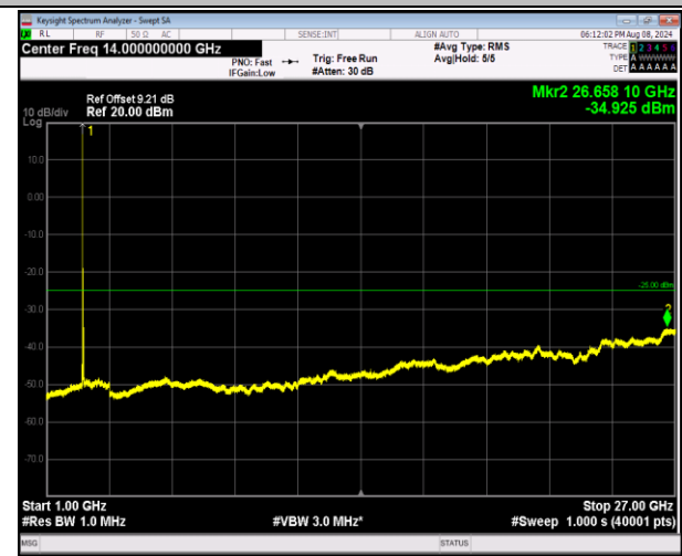
7-7-10MHz-20MHz-16QAM-16QAM-20805-20949-1RB#0-0RB#0-1000~27000MHz-PASS
