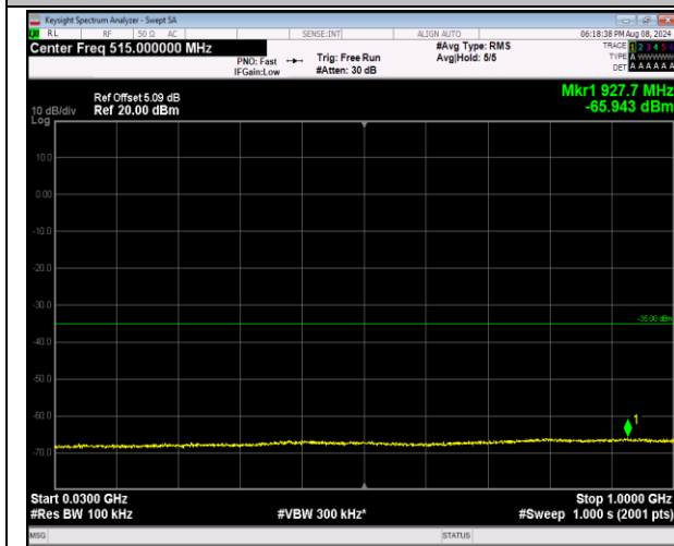
7-7-10MHz-20MHz-QPSK-QPSK-21006-21150-1RB#0-1 RB#99-30~1000MHz-PASS
