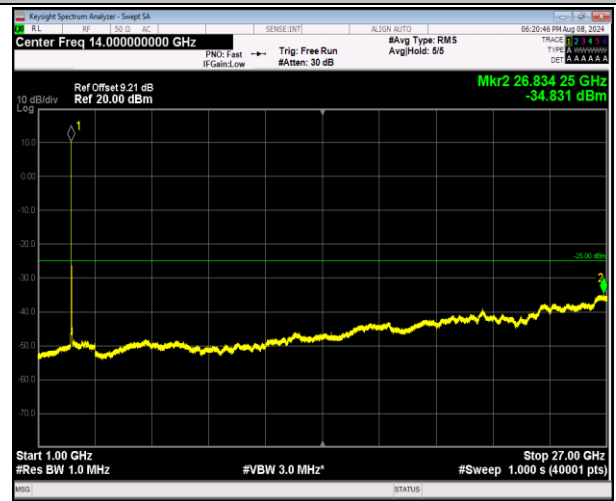
7-7-10MHz-20MHz-16QAM-16QAM-21006-21150-50RB# 0-100RB#0-1000~27000MHz-PASS
