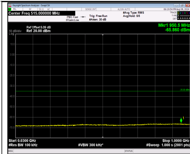
7-7-10MHz-20MHz-QPSK-QPSK-21006-21150-50RB#0-100RB#0-30~1000MHz-PASS
