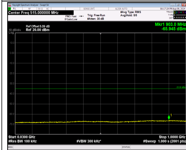
7-7-10MHz-20MHz-QPSK-QPSK-21006-21150-1RB#49- ORB#0-30~1000MHz-PASS
