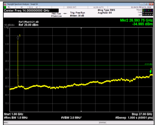
7-7-20MHz-10MHz-64QAM-64QAM-20850-20994-100RB #0-50RB#0-1000~27000MHz-PASS
