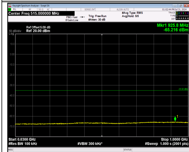
7-7-20MHz-10MHz-64QAM-64QAM-20850-20994-1RB# 0-0RB#0-30~1000MHz-PASS
