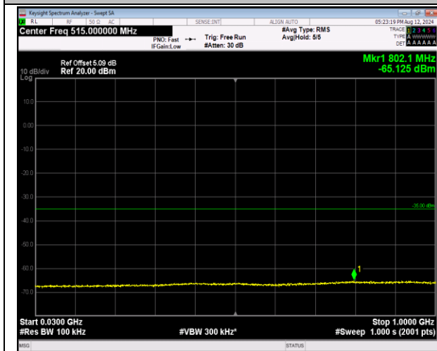
7-7-20MHz-10MHz-QPSK-QPSK-21051-21195-1RB#99- ORB#0-30~1000MHz-PASS
