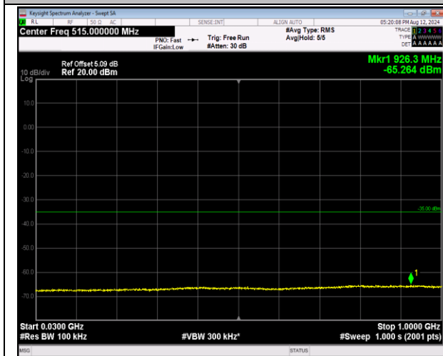
7-7-20MHz-10MHz-16QAM-16QAM-20850-20994-1RB# 0-1RB#49-30~1000MHz-PASS
