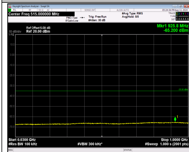
7-7-20MHz-10MHz-QPSK-QPSK-21051-21195-1RB#0-1 RB#49-30~1000MHz-PASS
