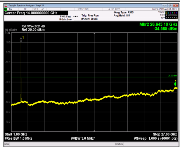
7-7-10MHz-20MHz-16QAM-16QAM-21206-21350-50RB# 0-100RB#0-1000~27000MHz-PASS
