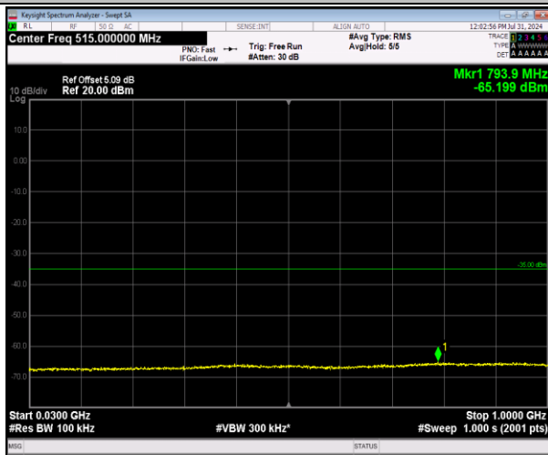
7-7-10MHz-20MHz-64QAM-64QAM-21006-21150-1RB# 0-0RB#0-30~1000MHz-PASS
