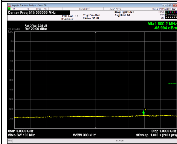
7-7-10MHz-20MHz-16QAM-16QAM-21006-21150-1RB#0-0-0RB#0-30~1000MHz-PASS
