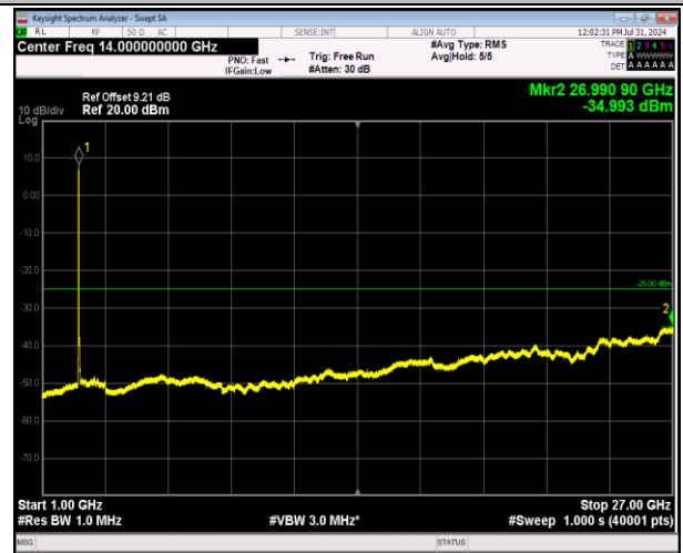
7-7-10MHz-20MHz-64QAM-64QAM-20805-20949-50RB# 0-100RB#0-1000~27000MHz-PASS
