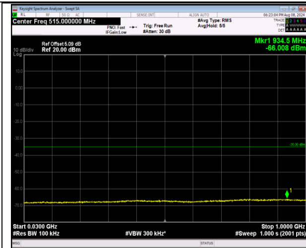
7-7-10MHz-20MHz-16QAM-16QAM-21206-21350-1RB# 49-0RB#0-30~1000MHz-PASS
