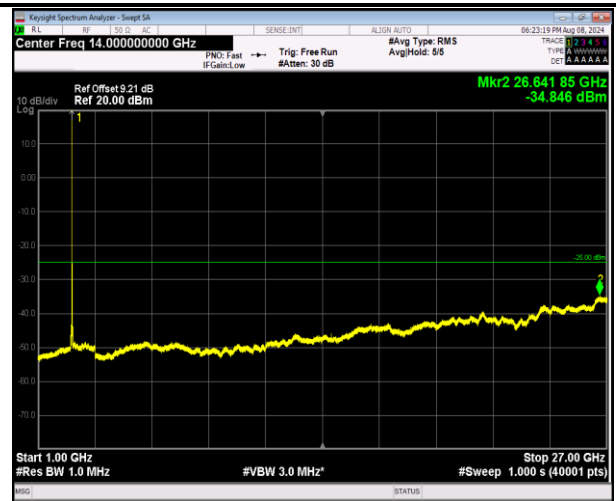
7-7-10MHz-20MHz-16QAM-16QAM-21206-21350-1RB#4 9-0RB#0-1000~27000MHz-PASS
