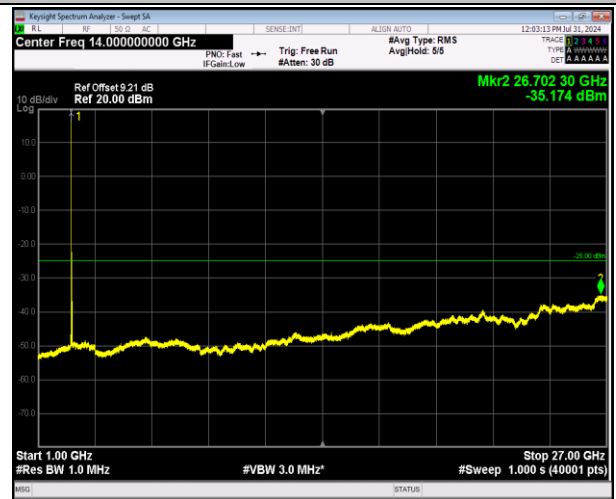
7-7-10MHz-20MHz-64QAM-64QAM-21006-21150-1RB#0- 0RB#0-1000~27000MHz-PASS
