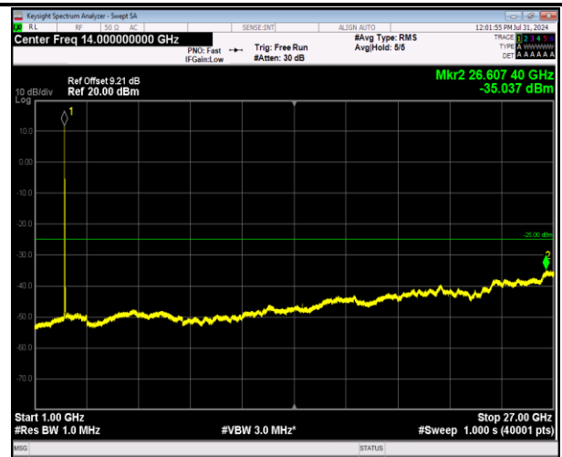
7-7-10MHz-20MHz-64QAM-64QAM-20805-20949-1RB#0 -1RB#99-1000~27000MHz-PASS
