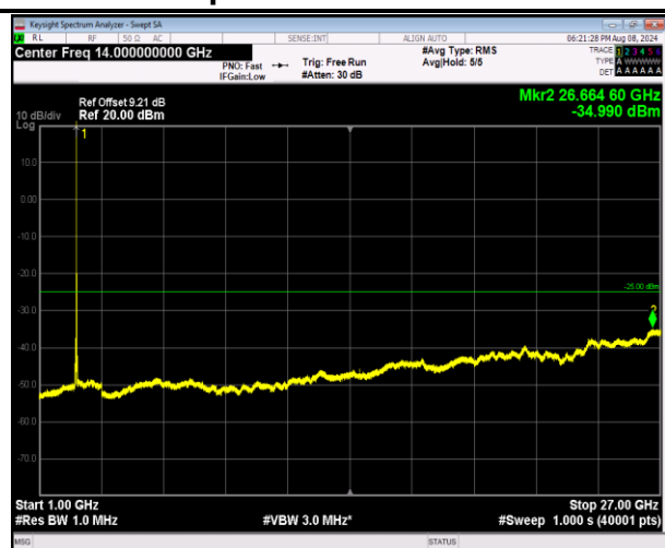
7-7-10MHz-20MHz-QPSK-QPSK-21206-21350-1RB#0-0 RB#0-1000~27000MHz-PASS
