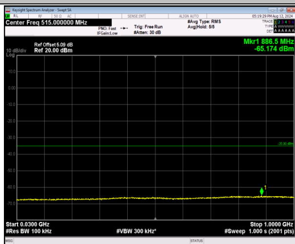
7-7-20MHz-10MHz-QPSK-QPSK-20850-20994-1RB#0-1 RB#49-30~1000MHz-PASS
