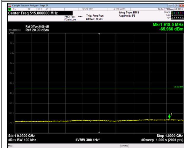
7-7-10MHz-20MHz-16QAM-16QAM-21206-21350-1RB#0-0RB#99-30~1000MHz-PASS
