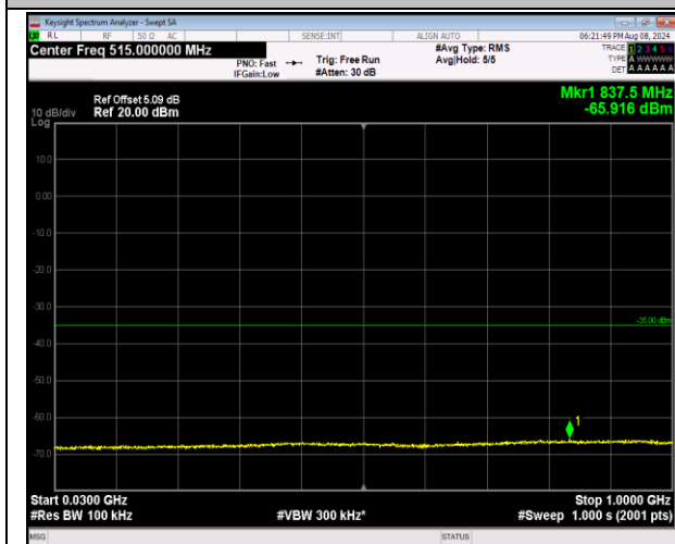
7-7-10MHz-20MHz-16QAM-16QAM-21206-21350-1RB#0-0RB#0-30~1000MHz-PASS
