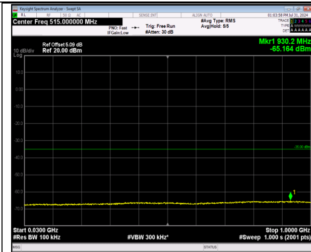
7-7-20MHz-10MHz-64QAM-64QAM-20850-20994-1RB# 0-1RB#49-30~1000MHz-PASS
