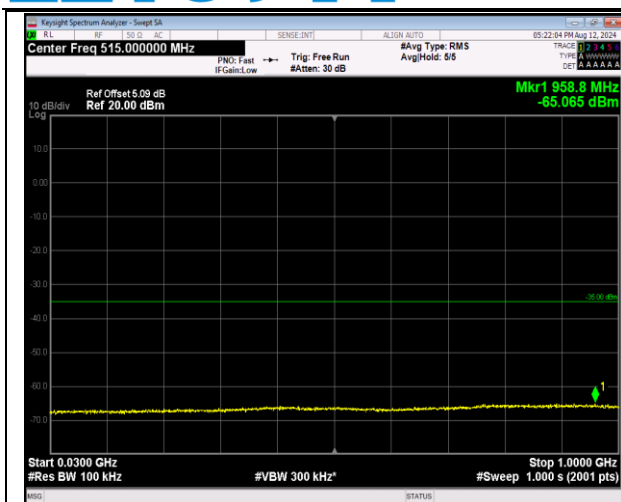
7-7-20MHz-10MHz-QPSK-QPSK-21051-21195-1RB#0-0 RB#0-30~1000MHz-PASS
