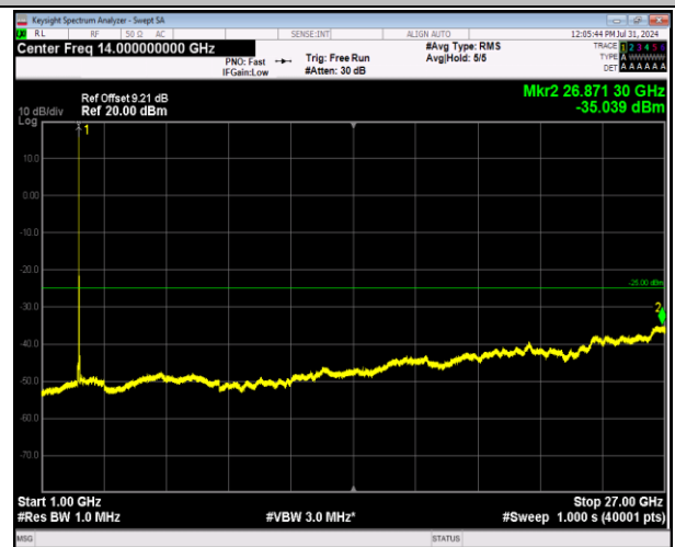
7-7-10MHz-20MHz-64QAM-64QAM-21206-21350-1RB#0 -0RB#0-1000~27000MHz-PASS
