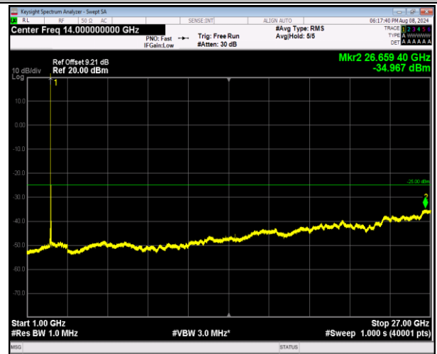
7-7-10MHz-20MHz-QPSK-QPSK-21006-21150-1RB#49-0 RB#0-1000~27000MHz-PASS
