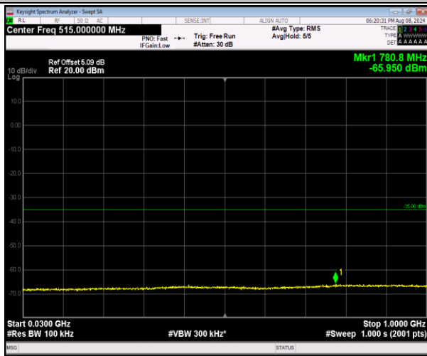
7-7-10MHz-20MHz-16QAM-16QAM-21006-21150-50RB #0-100RB#0-30~1000MHz-PASS
