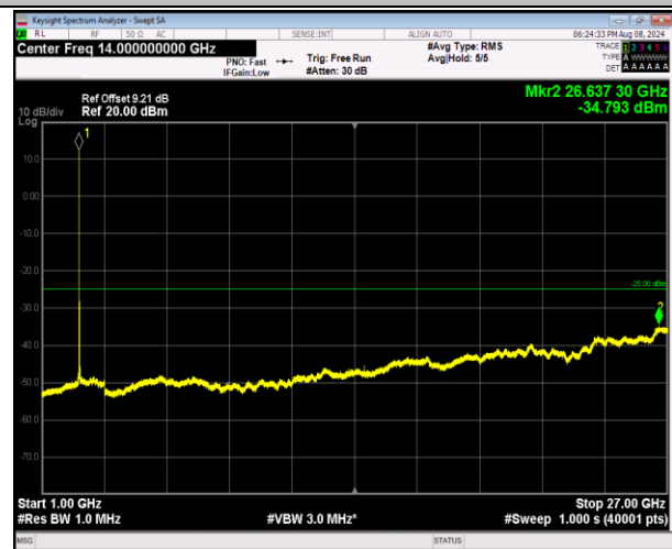
7-7-10MHz-20MHz-16QAM-16QAM-21206-21350-1RB#0-0RB#99-1000~27000MHz-PASS
