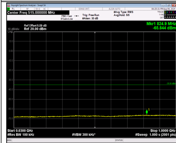
7-7-10MHz-20MHz-16QAM-16QAM-21206-21350-50RB #0-100RB#0-30~1000MHz-PASS
