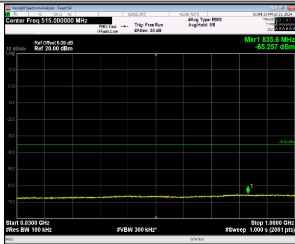
7-7-20MHz-10MHz-64QAM-64QAM-20850-20994-100R B#0-50RB#0-30~1000MHz-PASS
