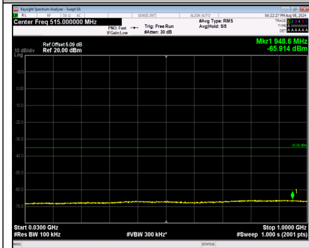
7-7-10MHz-20MHz-QPSK-QPSK-21206-21350-1RB#49-0 ORB#0-30~1000MHz-PASS
