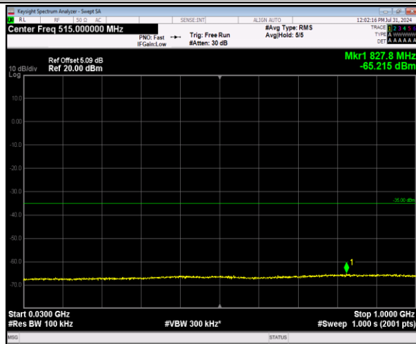
7-7-10MHz-20MHz-64QAM-64QAM-20805-20949-50RB #0-100RB#0-30~1000MHz-PASS
