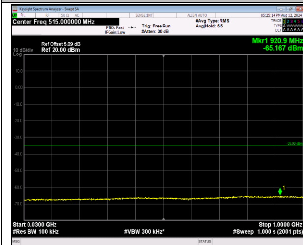
7-7-20MHz-10MHz-16QAM-16QAM-21051-21195-1RB#0-0-1RB#49-30~1000MHz-PASS
