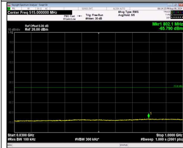
7-7-10MHz-20MHz-16QAM-16QAM-20805-20949-1RB#0-0-1RB#99-30~1000MHz-PASS
