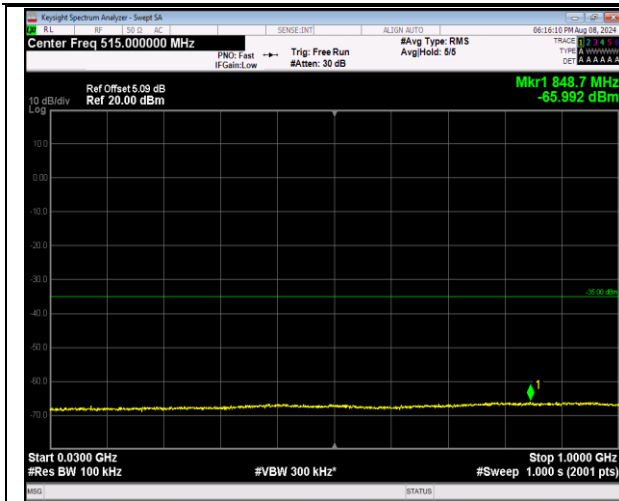
7-7-10MHz-20MHz-QPSK-QPSK-21006-21150-1RB#0-0 RB#0-30~1000MHz-PASS
