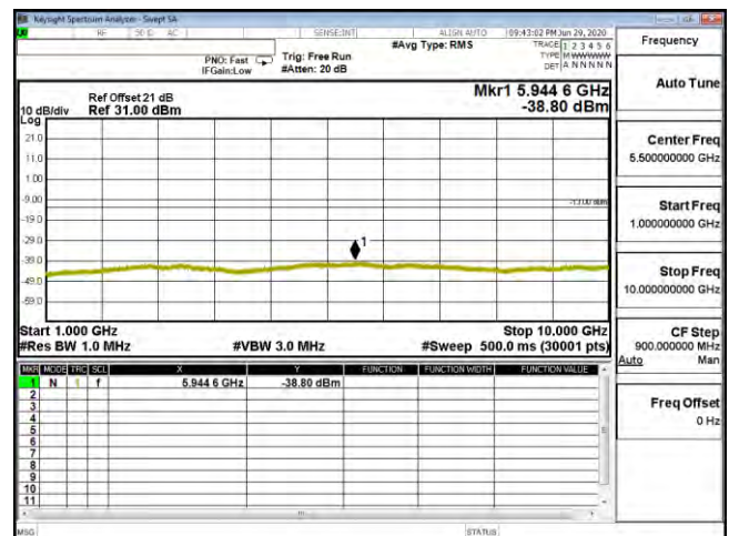
CSE B26 15M CH26865 64QAM(1,37) 1G-10G
