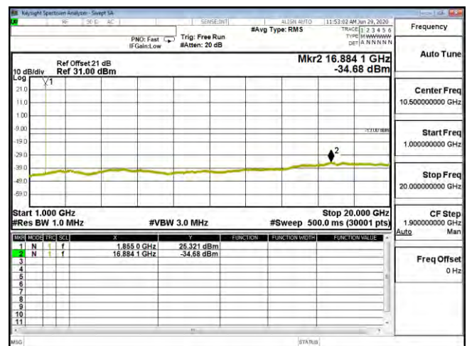
CSE B25 10M CH26090 16QAM(1,25) 1G-20G
