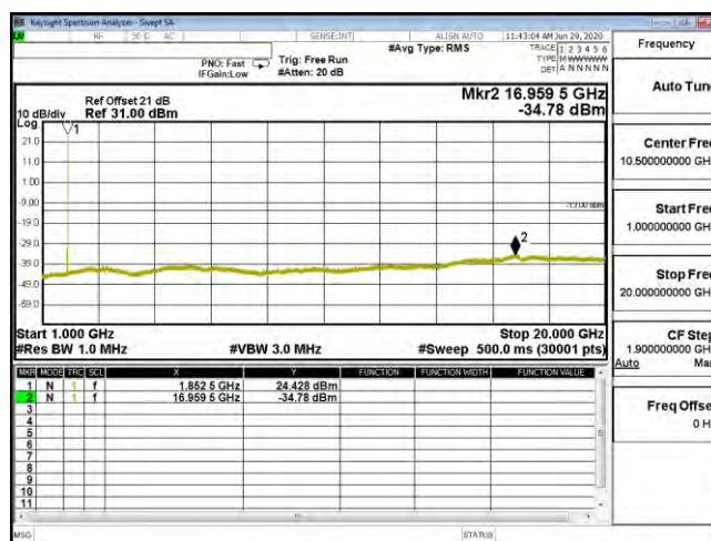
CSE B25 5M CH26065 16QAM(1,12) 1G-20G
