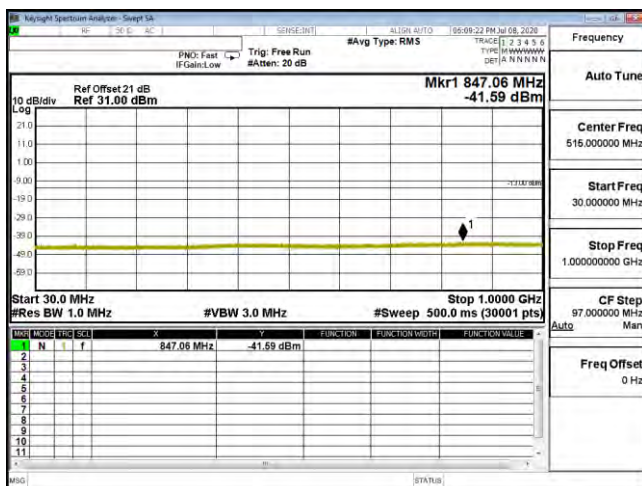
CSE B25 10M CH26365 16QAM(1,25) 30M-1G
