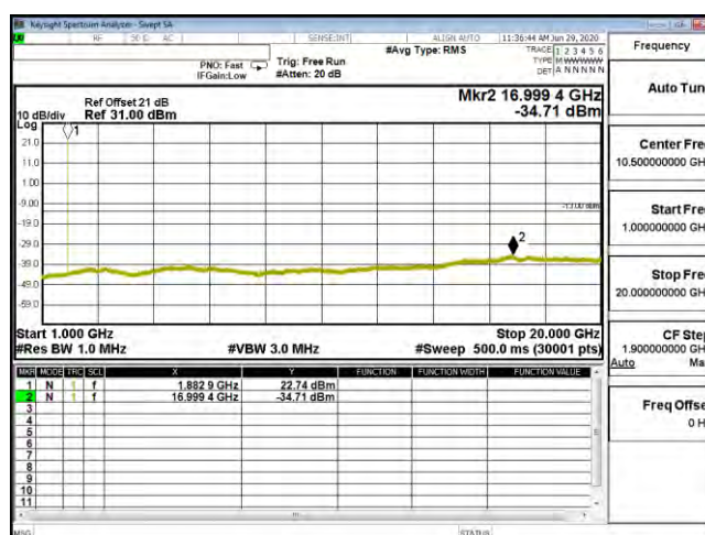
CSE B25 3M CH26365 64QAM(1,7) 1G-20G
