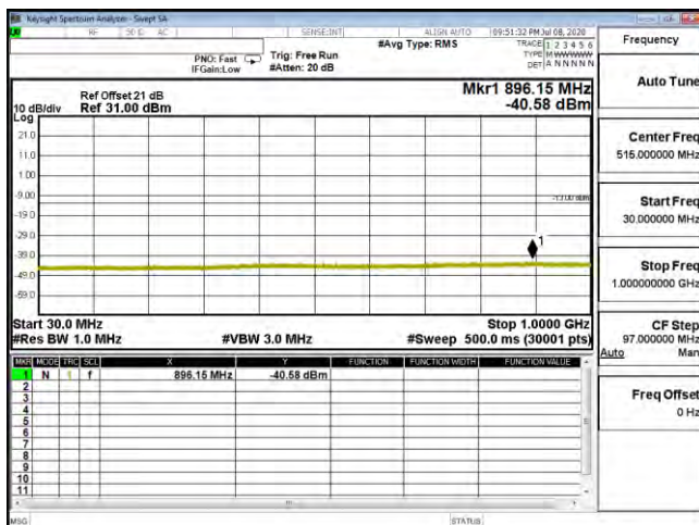
CSE B25 15M CH26615 64QAM(1,37) 30M-1G
