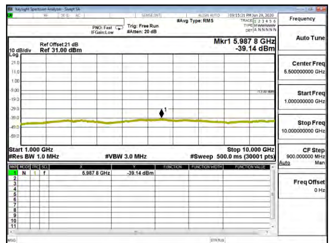
CSE B26 5M CH26815 16QAM(1,12) 1G-10G
