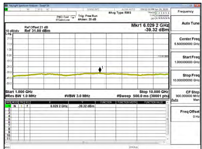
CSE B26 10M CH26915 16QAM(1,0) 1G-10G
