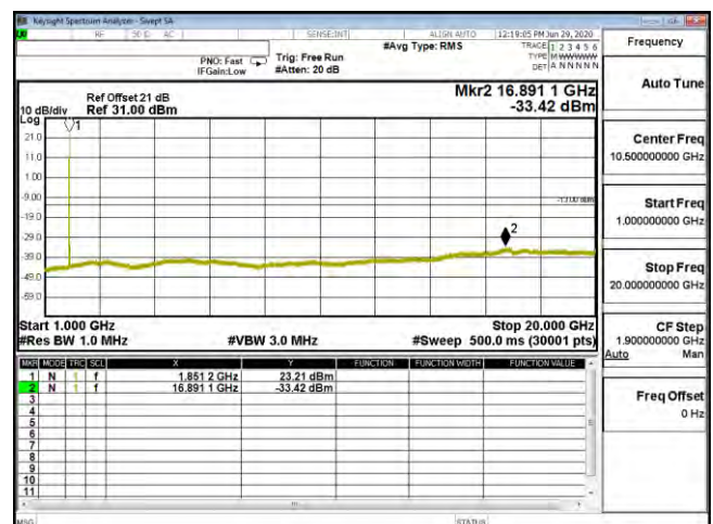
CSE B25 20M CH26140 64QAM(1,0) 1G-20G
