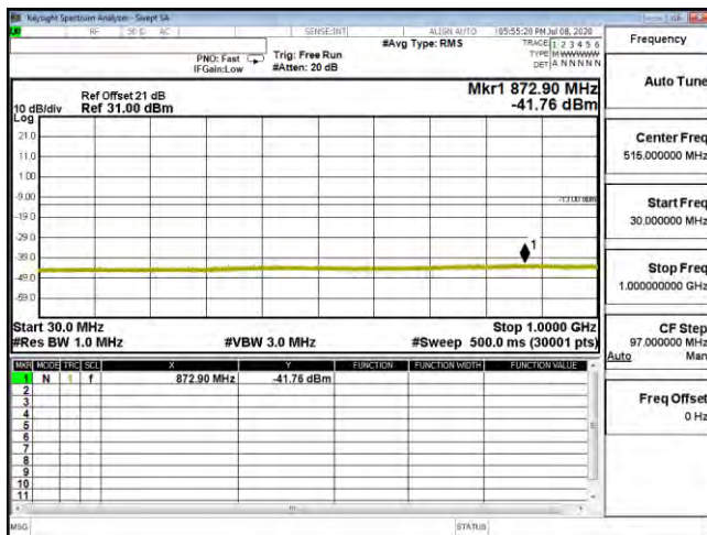
CSE B25 3M CH26055 16QAM(1,0) 30M-1G
