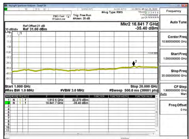
CSE B25 5M CH26665 64QAM(1,12) 1G-20G
