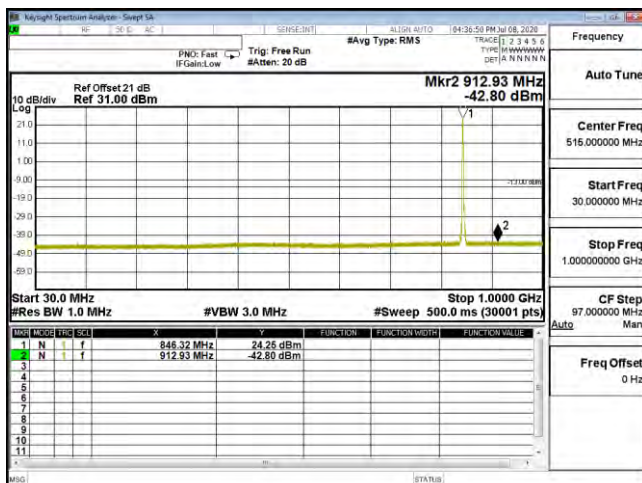
CSE B26 3M CH27025 64QAM(1,0) 30M-1G
