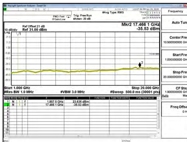
CSE B25 15M CH26115 64QAM(1,37) 1G-20G
