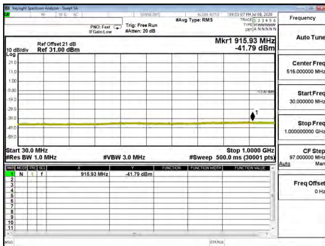
CSE B25 15M CH26615 16QAM(1,37) 30M-1G
