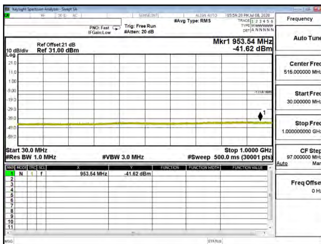
CSE B25 3M CH26675 16QAM(1,0) 30M-1G
