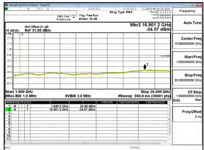
CSE B25 3M CH26055 16QAM(1,0) 1G-20G
