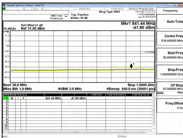
CSE B25 5M CH26665 16QAM(1,12) 30M-1G
