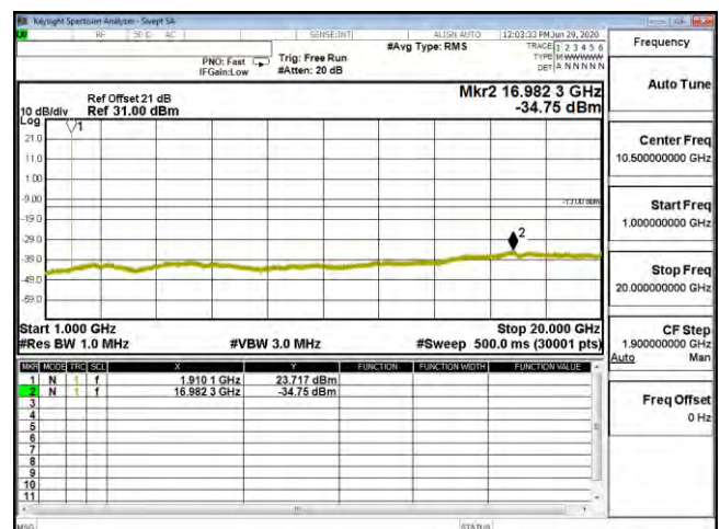
CSE B25 10M CH26640 64QAM(1,25) 1G-20G
