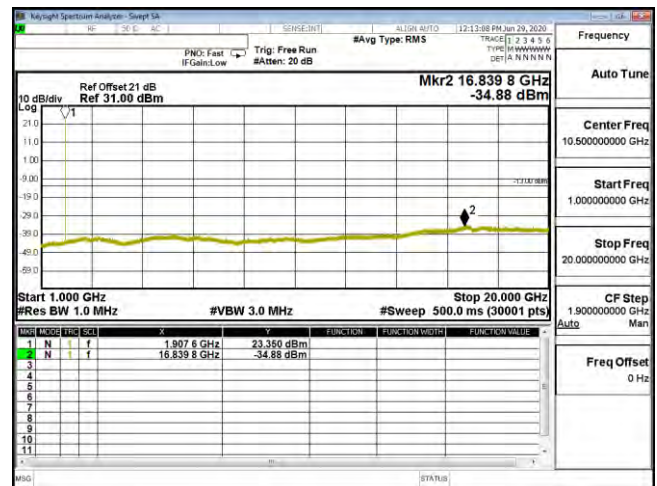
CSE B25 15M CH26615 16QAM(1,37) 1G-20G
