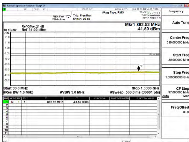
CSE B25 20M CH26590 64QAM(1,50) 30M-1G
