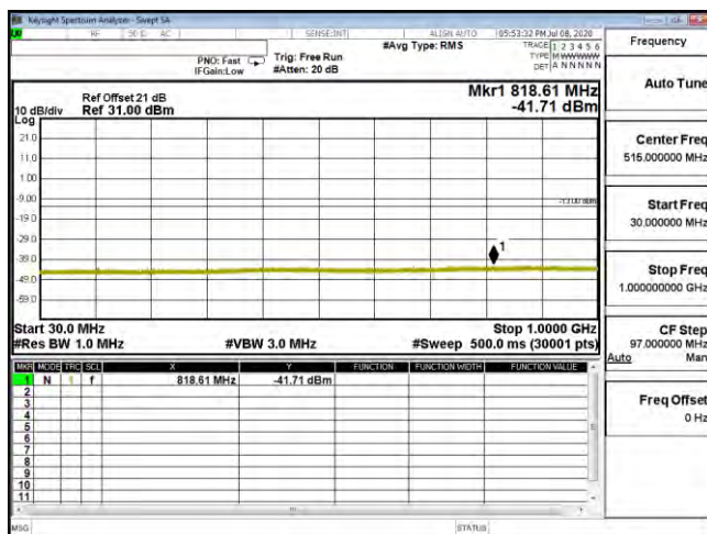
CSE B25 1.4M CH26683 16QAM(1,0) 30M-1G
