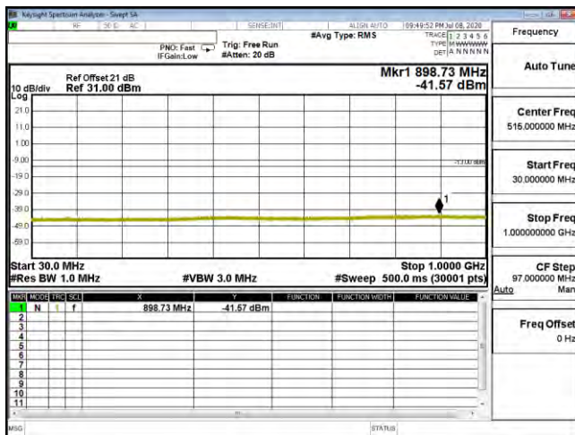
CSE B25 15M CH26365 16QAM(1,0) 30M-1G
