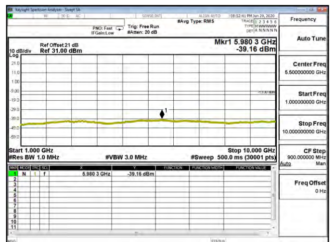
CSE B26 1.4M CH26915 64QAM(1,2) 1G-10G
