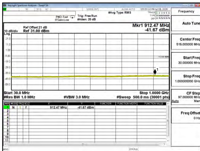
CSE B25 1.4M CH26683 QPSK(1,0) 30M-1G
