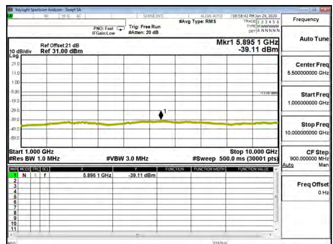
CSE B26 3M CH26805 64QAM(1,7) 1G-10G
