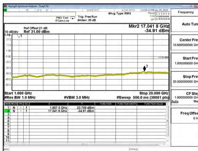
CSE B25 15M CH26115 16QAM(1,37) 1G-20G
