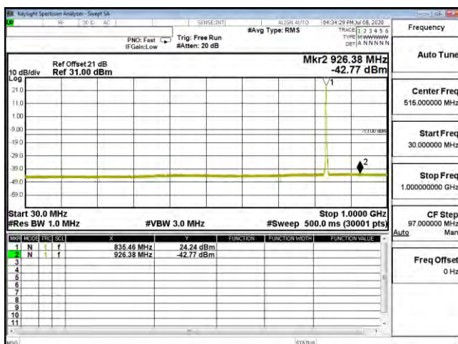
CSE B26 3M CH26915 64QAM(1,0) 30M-1G
