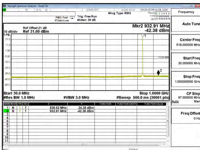
CSE B26 1.4M CH26915 64QAM(1,2) 30M-1G
