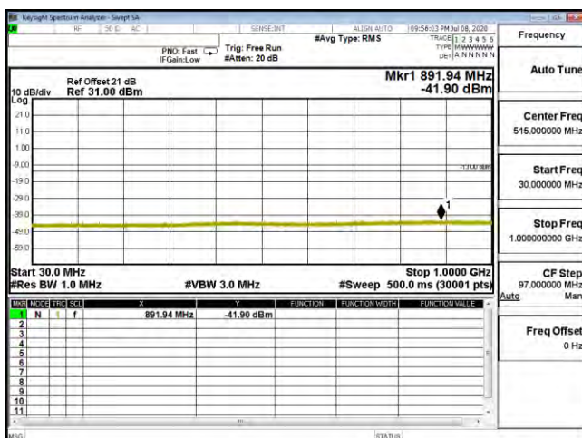
CSE B25 20M CH26365 64QAM(1,50) 30M-1G
