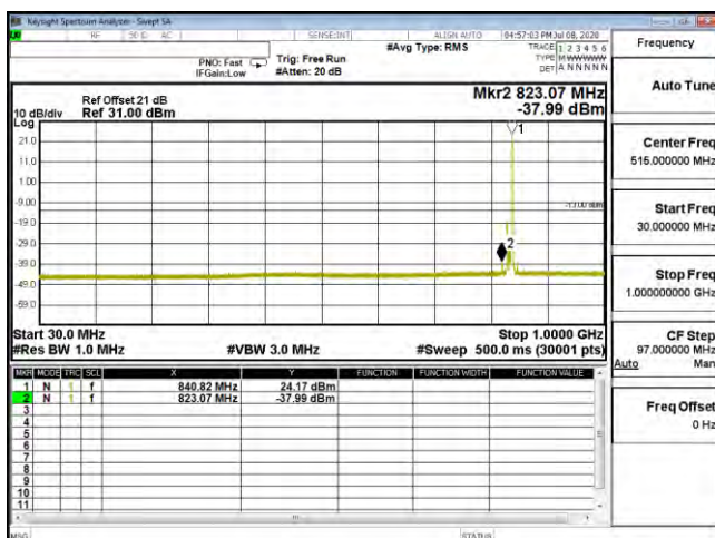
CSE B26 10M CH26915 64QAM(1,49) 30M-1G
