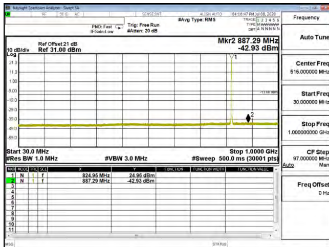
CSE B26 1.4M CH26797 16QAM(1,2) 30M-1G
