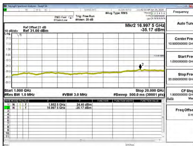
CSE B25 5M CH26065 QPSK(1,12) 1G-20G
