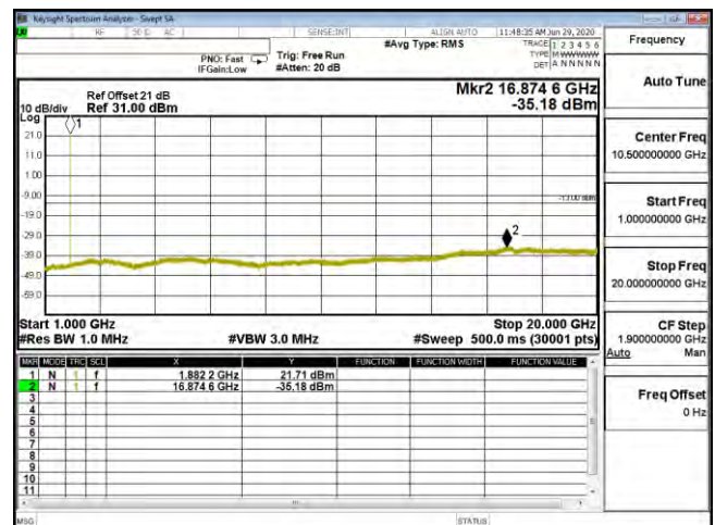
CSE B25 5M CH26365 64QAM(1,12) 1G-20G
