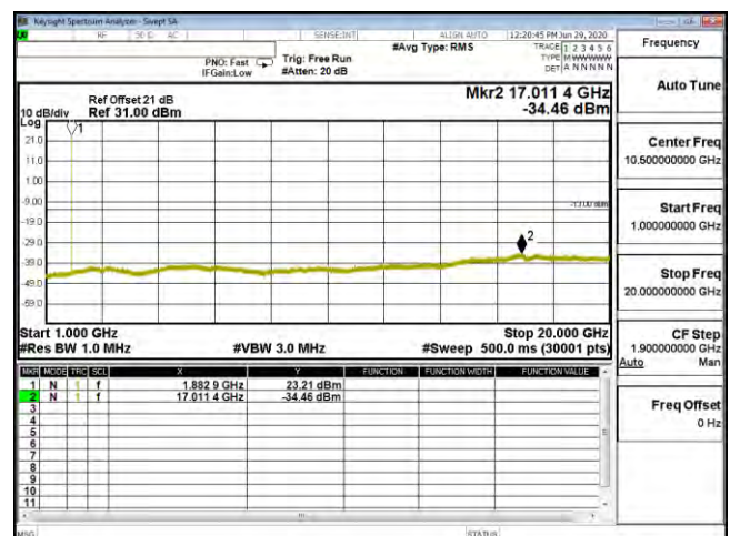
CSE B25 20M CH26365 64QAM(1,50) 1G-20G
