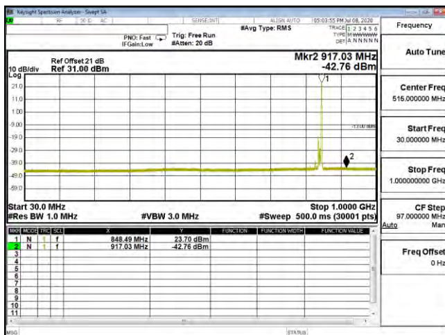
CSE B26 10M CH26990 64QAM(1,49) 30M-1G
