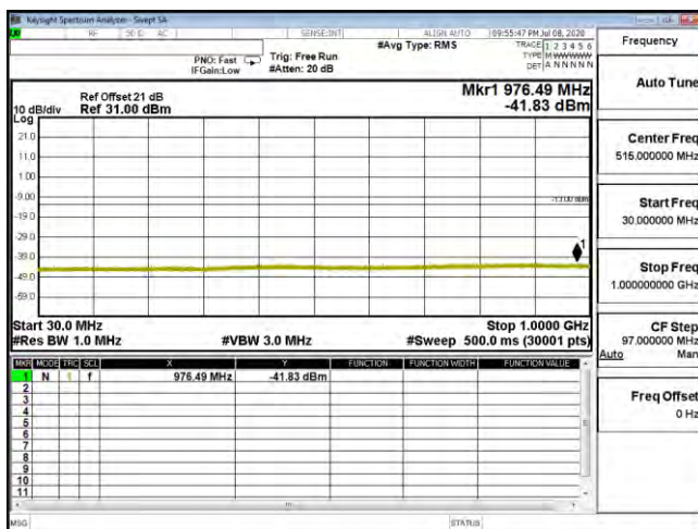
CSE B25 20M CH26365 16QAM(1,50) 30M-1G
