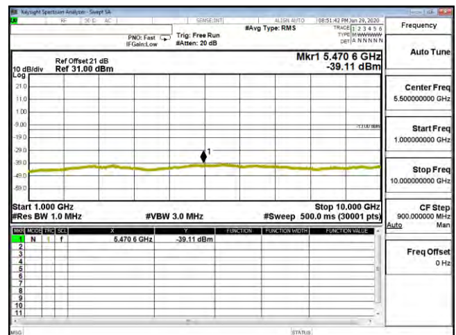
CSE B26 1.4M CH26797 64QAM(3,2) 1G-10G
