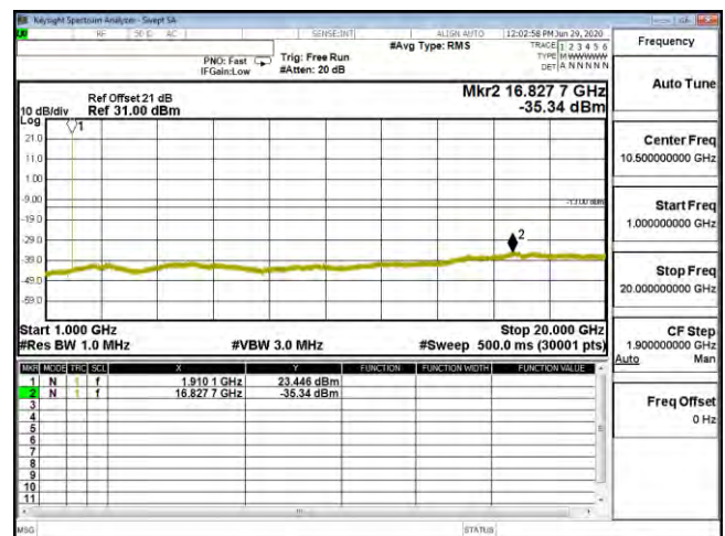
CSE B25 10M CH26640 16QAM(1,0) 1G-20G
