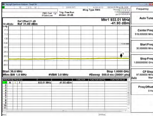
CSE B25 20M CH26140 16QAM(1,50) 30M-1G
