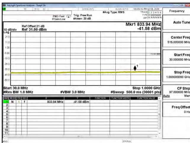
CSE B25 10M CH26090 16QAM(1,25) 30M-1G
