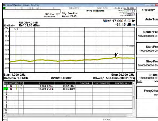
CSE B25 3M CH26365 16QAM(1,7) 1G-20G
