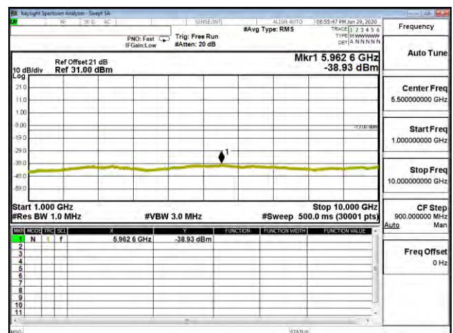
CSE B26 1.4M CH27033 64QAM(1,2) 1G-10G
