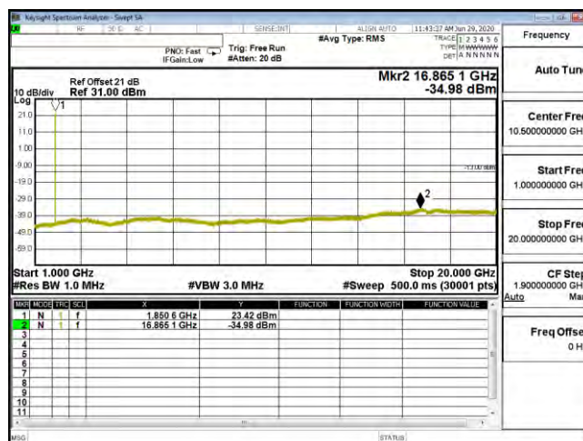
CSE B25 5M CH26065 64QAM(1,0) 1G-20G
