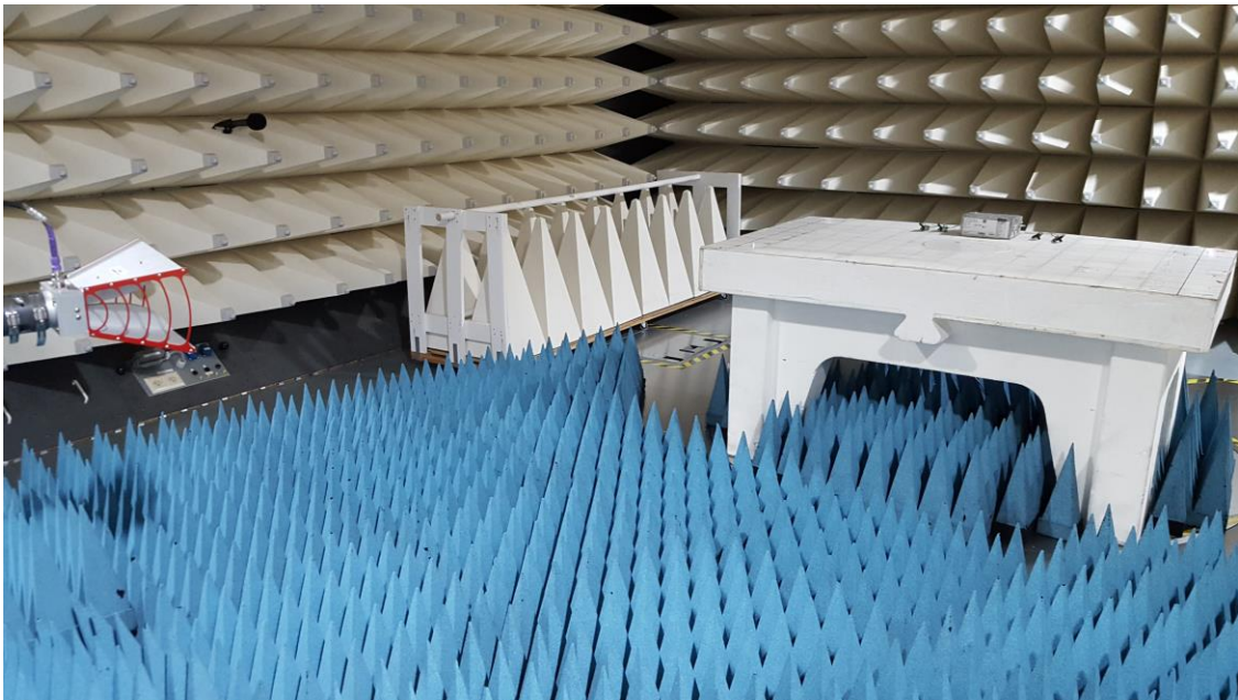
Figure C2. High Range Radiated Emission test setup 1-18GHz
