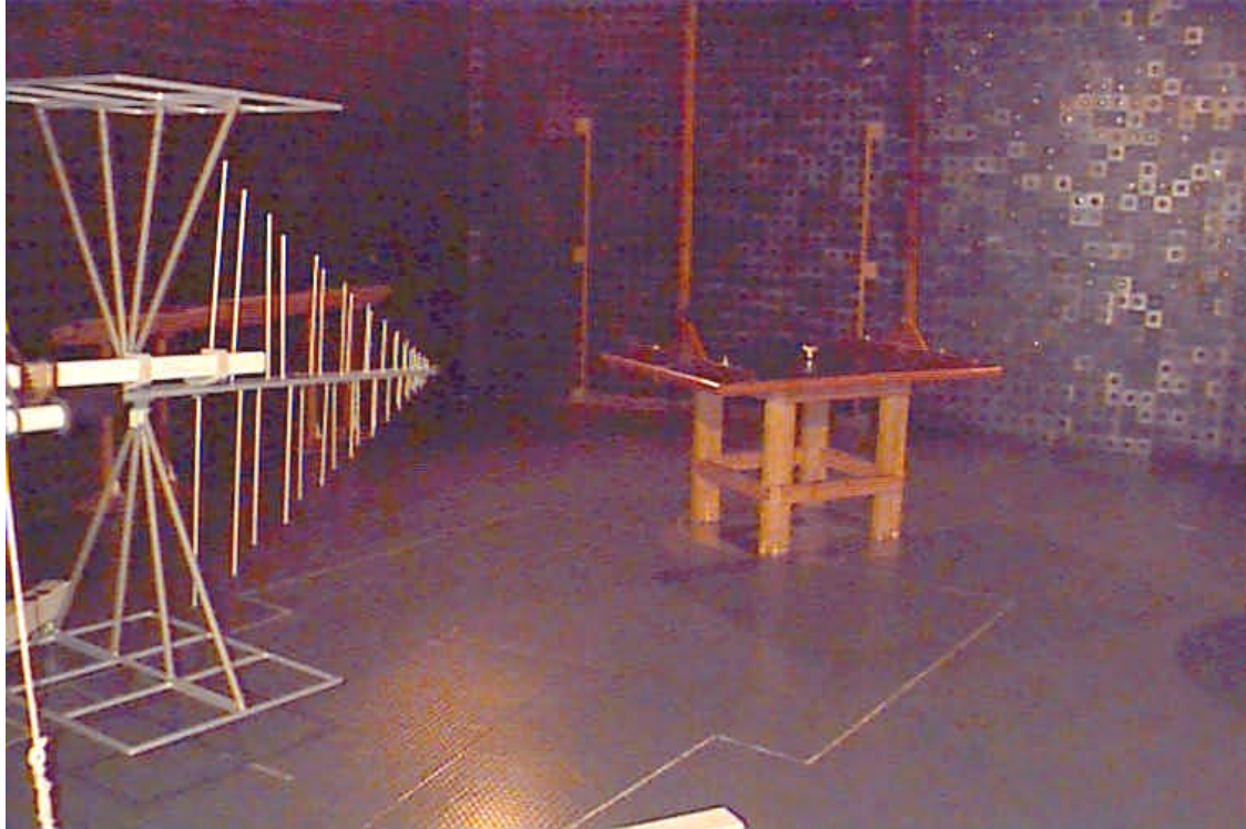
Setup for radiated measurements with biconilog antenna
