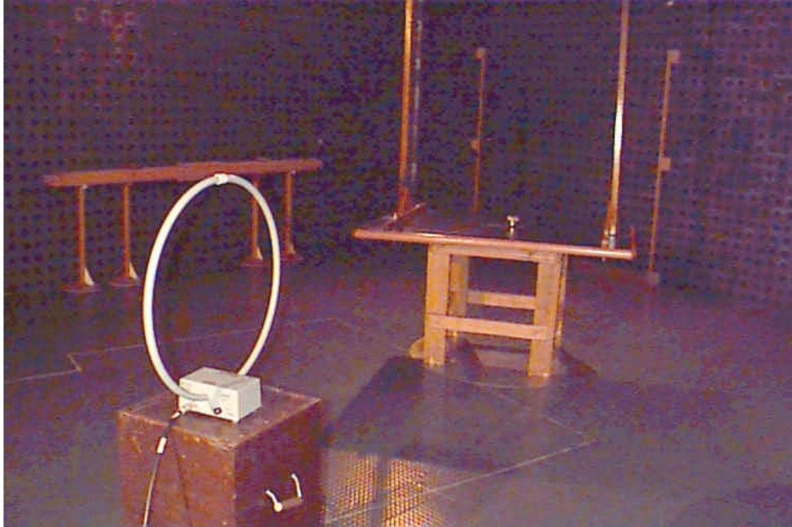
Setup for radiated measurements with loop antenna
