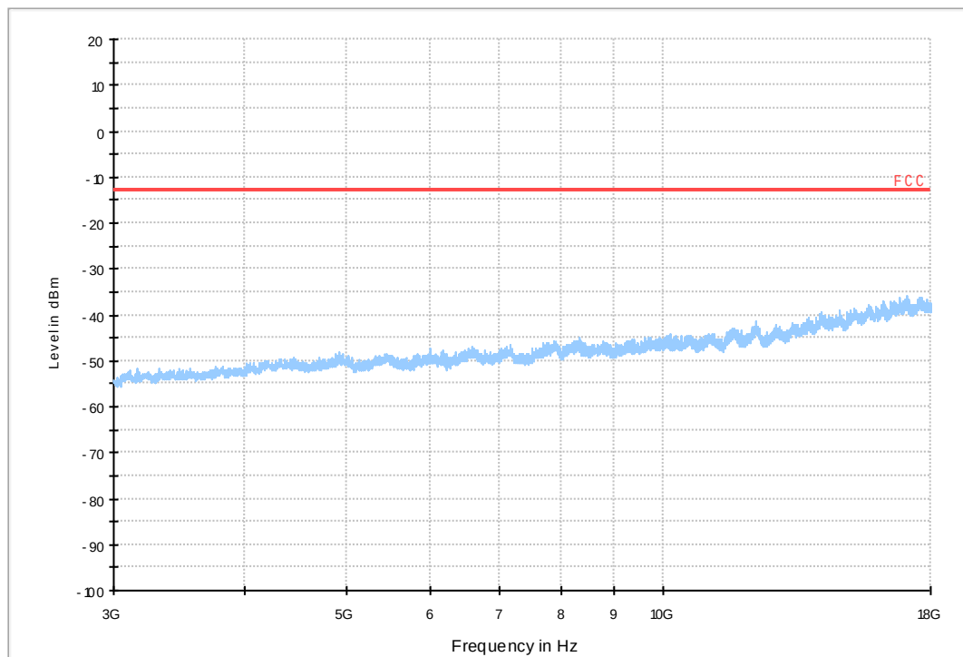
Band26(824-849MHz)/TM1_Ant2
