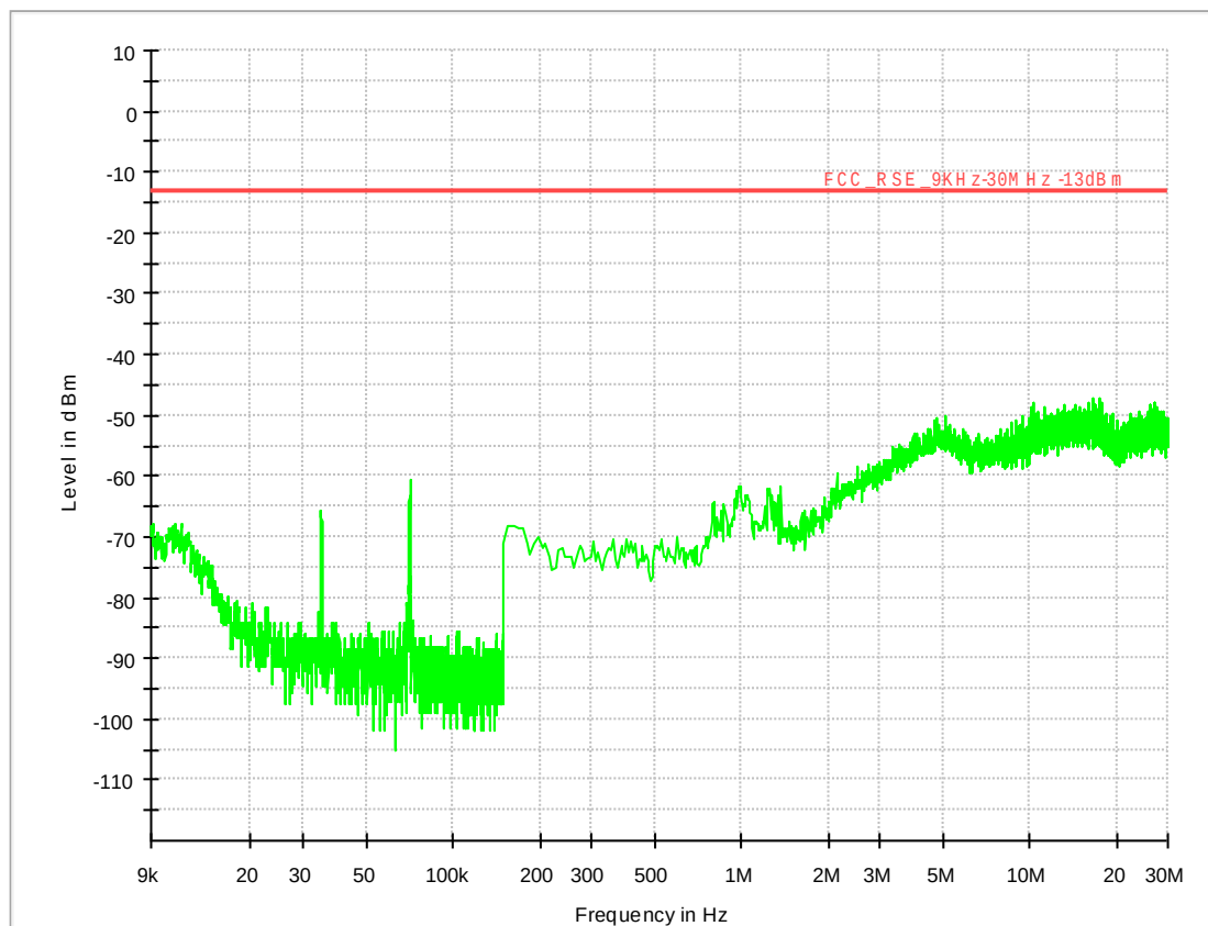
Band26(824-849MHz)/TM1_Ant2
