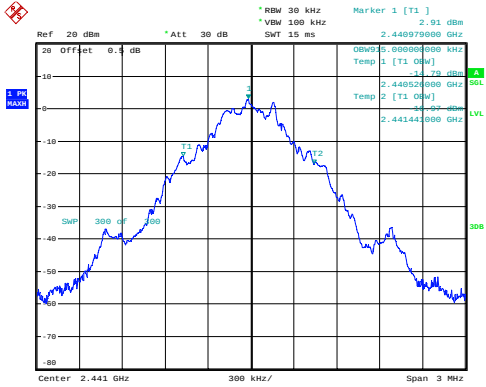
GFSK_Middle 0.915MHz
