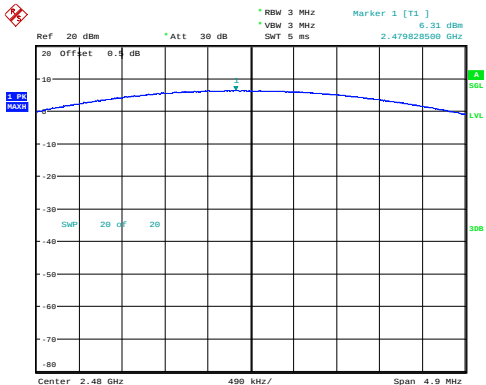
GFSK_High 6.31dBm
