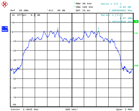
8DPSK_Low 1.001MHz
