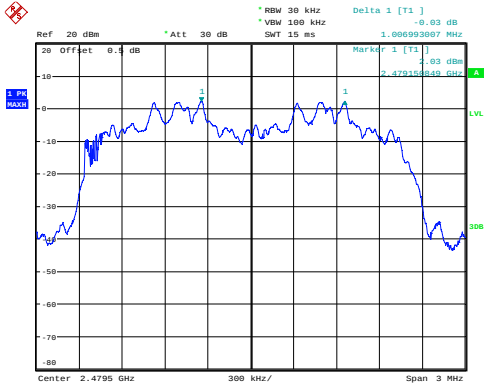
8DPSK_High 1.007MHz
