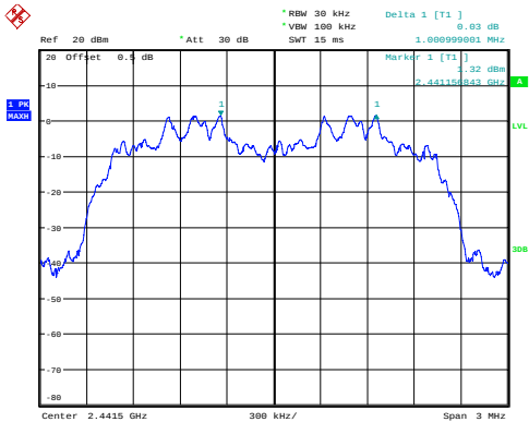
8DPSK_Middle 1.001MHz
