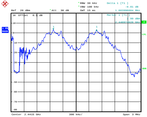
GFSK_Middle 1.004MHz
