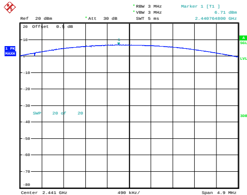
GFSK_Middle 6.71dBm
