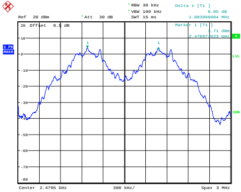
GFSK_High 1.004MHz
