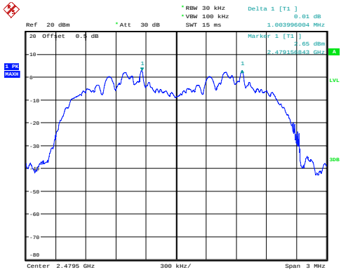
\pi/4 -DQPSK_High 1.004MHz
