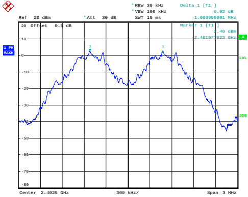
GFSK_Low 1.001MHz
