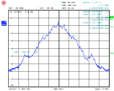
GFSK_Low 0.915MHz
