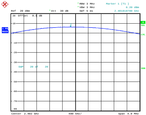
GFSK_Low 6.20dBm
