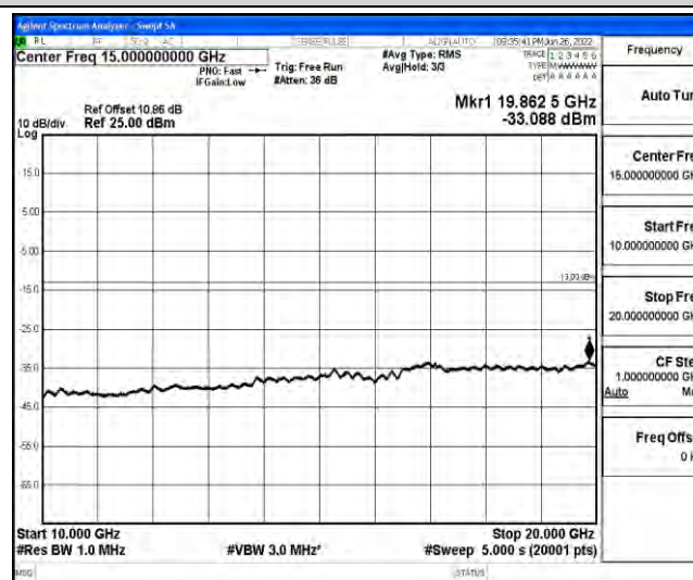
Band25-15MHz-16QAM-26365-1RB#0-Range5:10000~20000MHz
