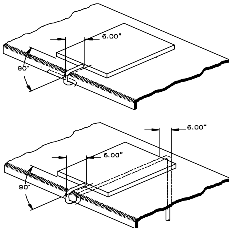
Figure 3.2.1 Pad Connection
