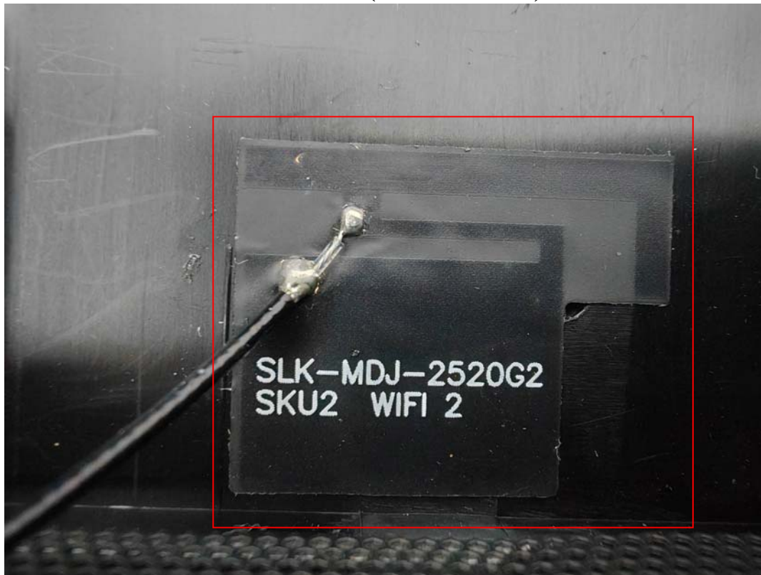
WLAN Antenna (Antenna 2, Chain 1)
