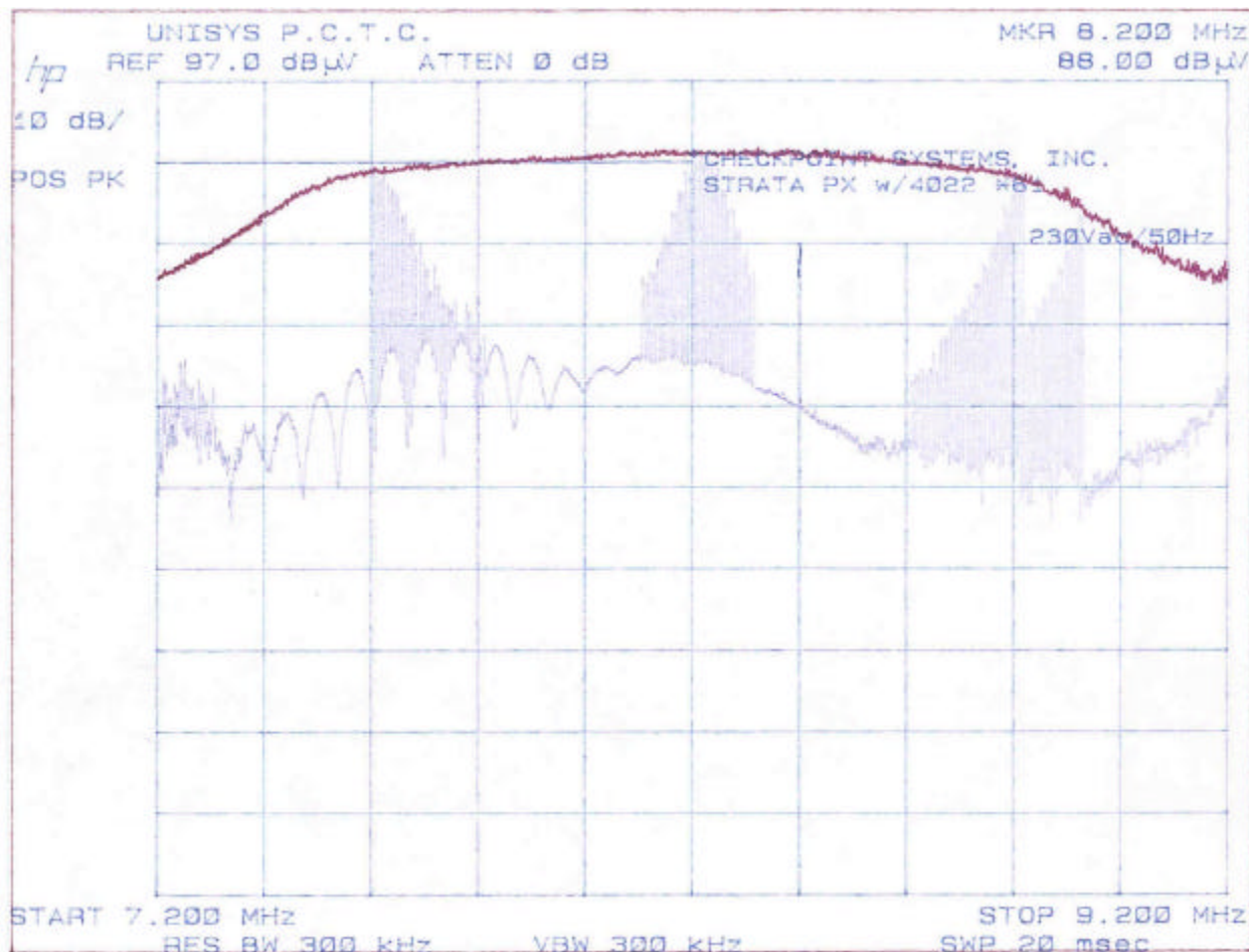
Photo 5 – Bandwidth Plot
