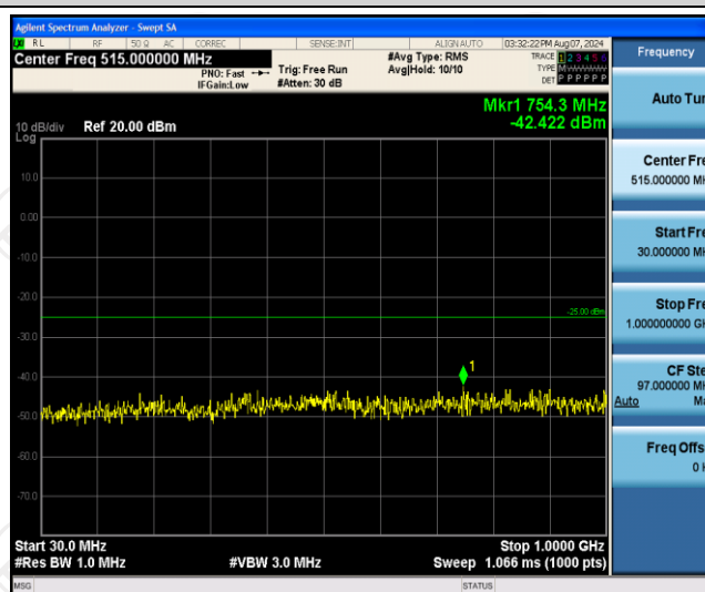
Band7-5MHz-16QAM-20775-1RB#0-Range1:30~1000MHz
