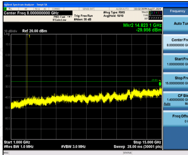
Band7-5MHz-16QAM-20775-1RB#0-Range2:1000~15000MHz
