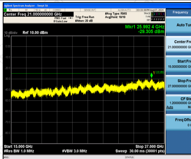
Band7-5MHz-QPSK-21100-1RB#0-Range3:15000~27000MHz
