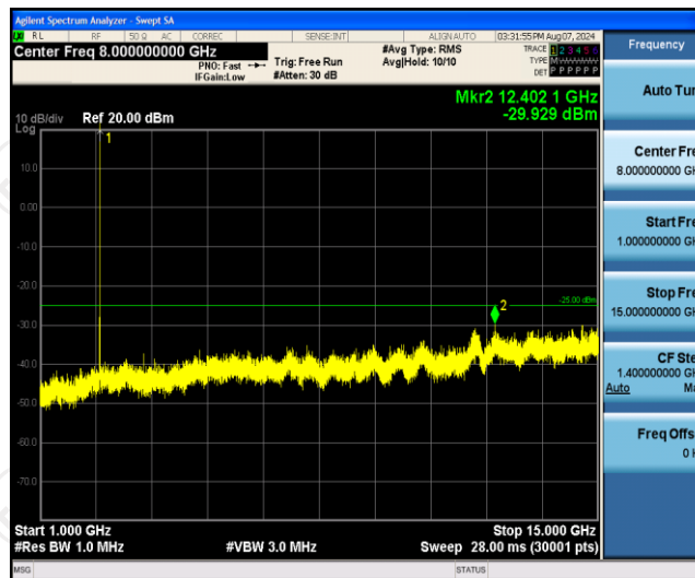
Band7-5MHz-QPSK-20775-1RB#0-Range2:1000~15000MHz
