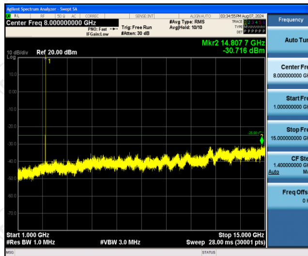
Band7-5MHz-QPSK-21425-1RB#0-Range2:1000~15000MHz
