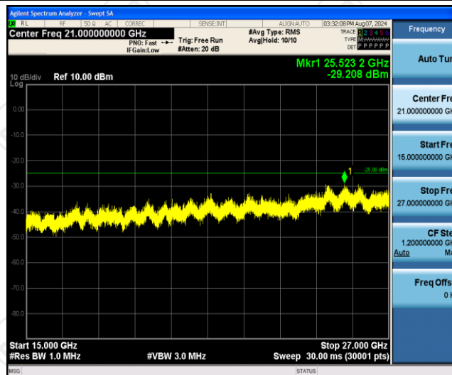
Band7-5MHz-QPSK-20775-1RB#0-Range3:15000~27000MHz
