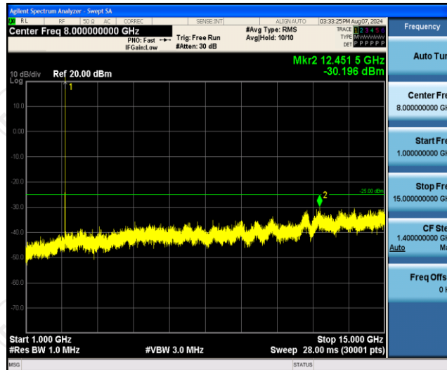
Band7-5MHz-QPSK-21100-1RB#0-Range2:1000~15000MHz
