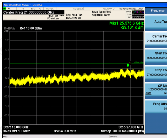
Band7-5MHz-16QAM-20775-1RB#0-Range3:15000~27000MHz
