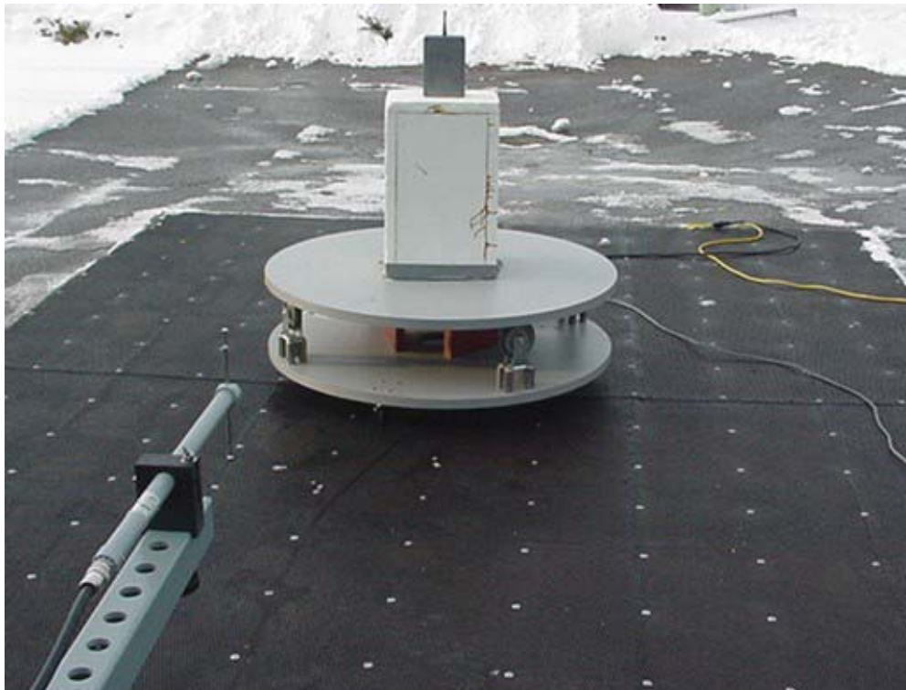
Radiated Measurement Test Setup Photograph
