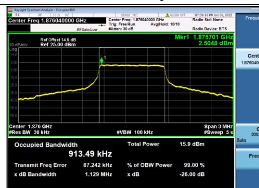
B2-10M-Mid CH-OBW-Q16
