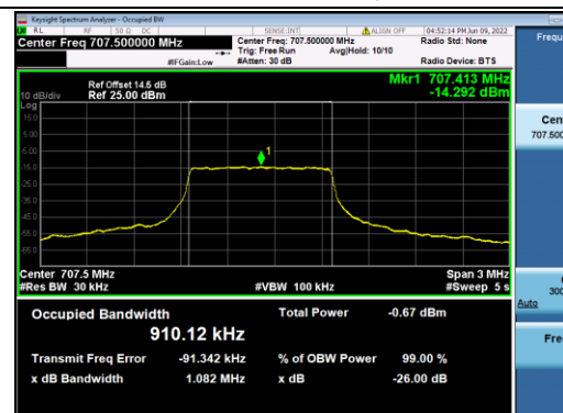
B12-1.4M-Mid CH-OBW-Q16
