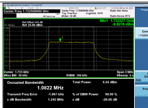
B4-1.4M-Mid CH-OBW-QPSK
