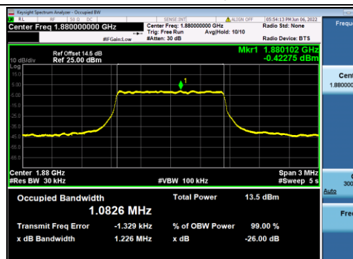
B2-1.4M-Mid CH-OBW-QPSK
