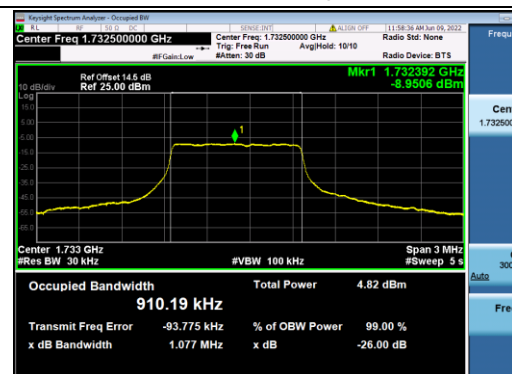
B4-1.4M-Mid CH-OBW-Q16
