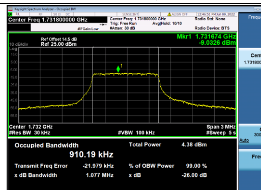
B4-3M-Mid CH-OBW-Q16
