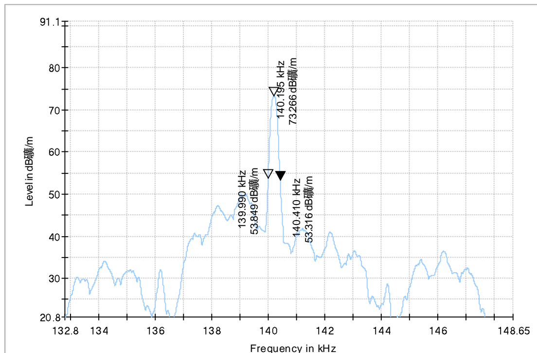
Fig. 1 Occupied Bandwidth (Set.WPT1)
