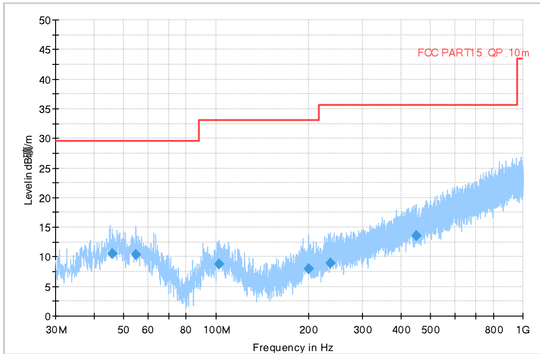
Fig. 3 Radiated Emission (Set.WPT1)
