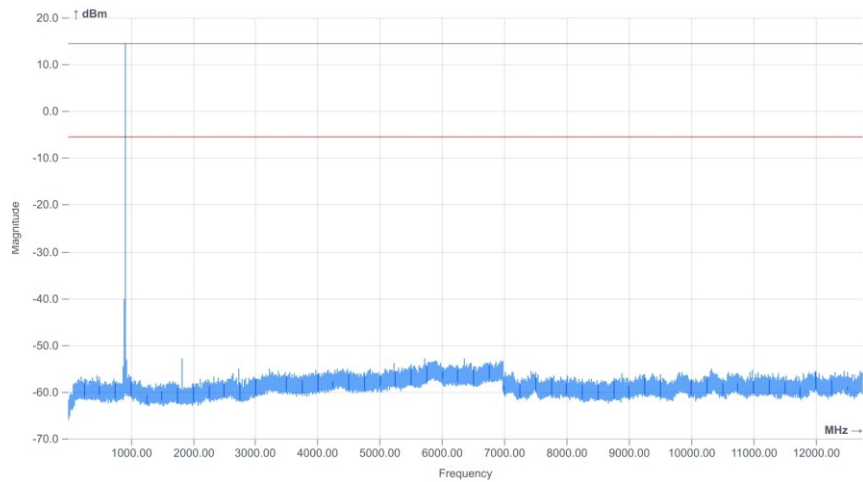
Plot 2: middle channel, 1 MHz – 12.75 GHz
