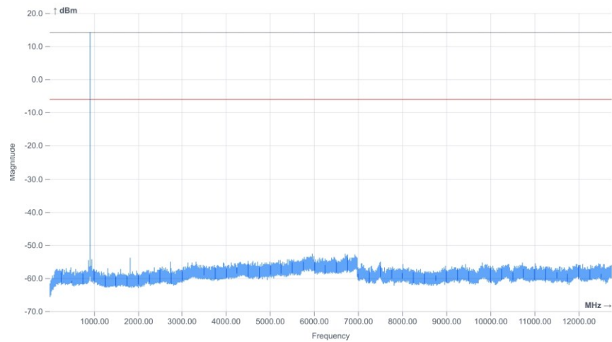
Plot 3: high channel, 1 MHz – 12.75 GHz
