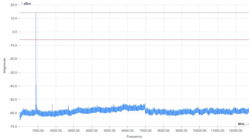
Plot 1: low channel, 1 MHz – 12.75 GHz
