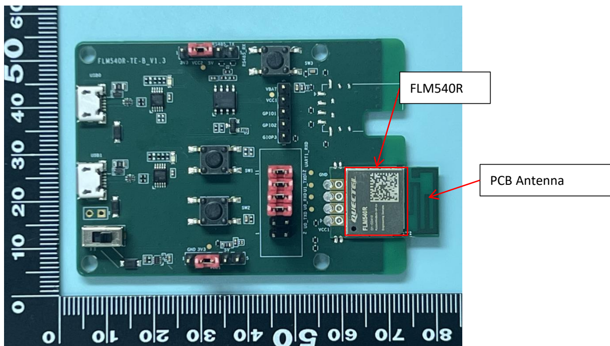
FLM540R + EVB_Top
