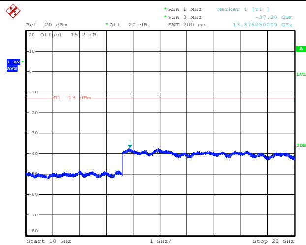
QPSK Middle channel-2
