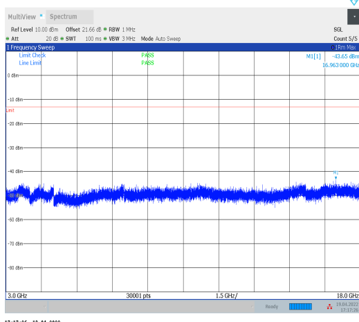
1-N70--15-15-H-1-DFT-PI2BPSK-Inner_1RB_Left-1 @1-3000-18000-Ant2--43.65--13-PASS
