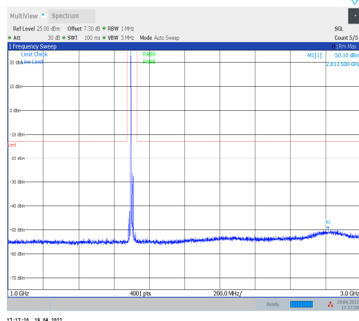
1-N70--15-15-H-1-DFT-PI2BPSK-Inner_1RB_Left-1 @1-1000-3000-Ant2--50.10--13-PASS
