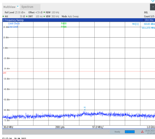
1-N70--15-15-H-1-DFT-PI2BPSK-Inner_1RB_Left-1 @1-30-1000-Ant2--60.82--23-PASS
