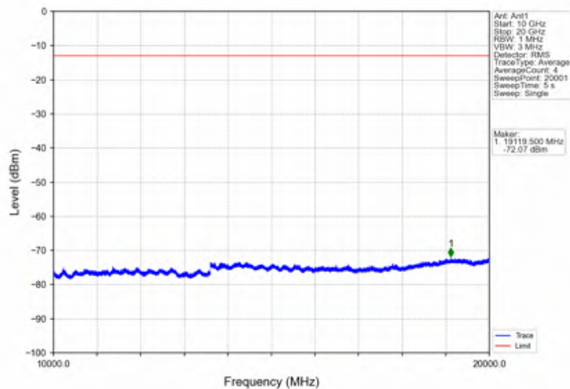
Band4_10MHz_256QAM_LCH_1715MHz_RB_50_0_NTNV
