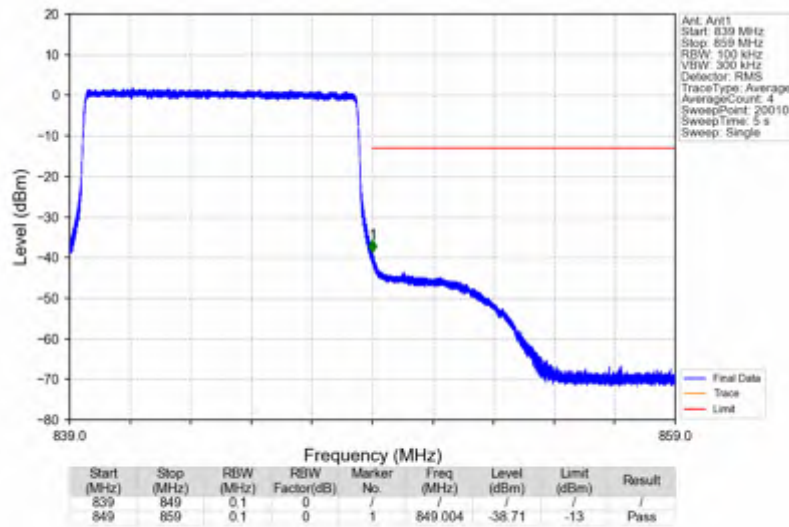
Band5_10MHz_256QAM_HCH_844MHz_RB_50_0_NTV
