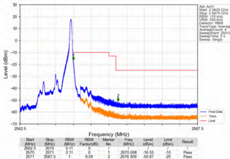
Band7_5MHz_256QAM_HCH_2567.5MHz_RB_1_24_NTNV
