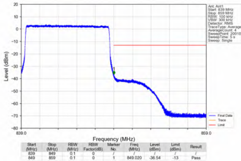
Band5_10MHz_64QAM_HCH_844MHz_RB_50_0_NTNV
