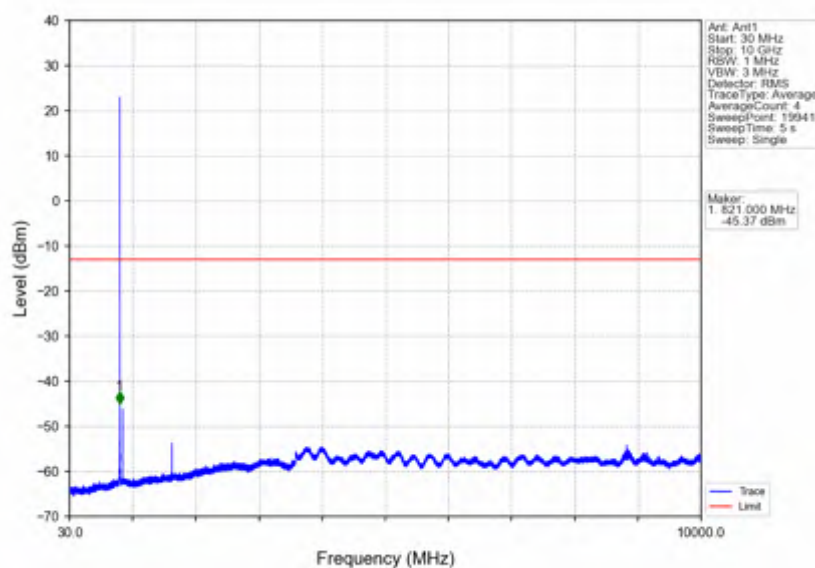
Band5_1.4MHz_QPSK_LCH_824.7MHz_RB_1_0_NTNV
