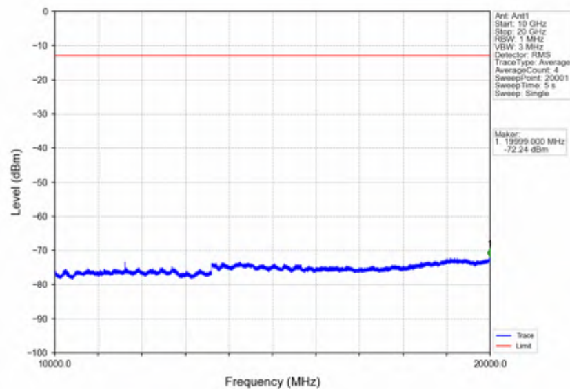
Band4_15MHz_QPSK_LCH_1717.5MHz_RB_75_0_NTNV
