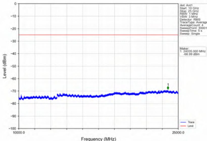
Band7_10MHz_256QAM_MCH_2535MHz_RB_1_0_NTNV
