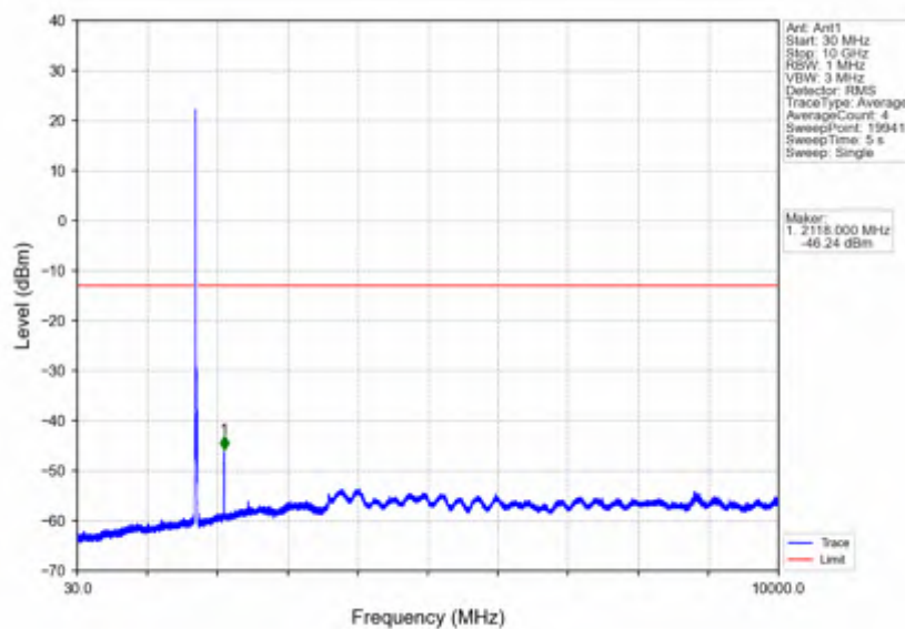
Band4_15MHz_16QAM_LCH_1717.5MHz_RB_1_0_NTNV
