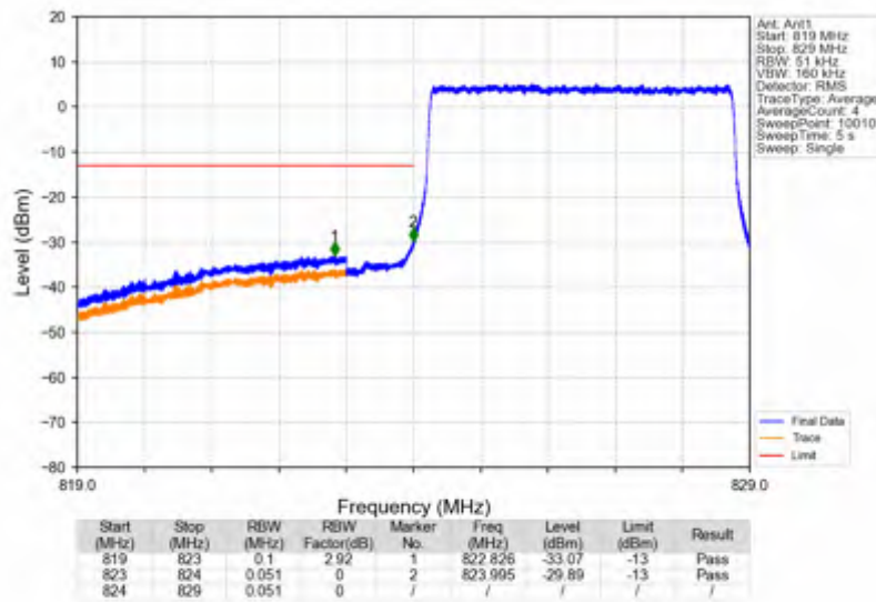
Band5_5MHz_QPSK_LCH_826.5MHz_RB_1_0_NTNV
