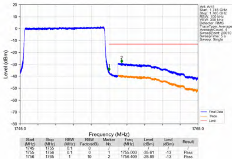
Band4_10MHz_256QAM_HCH_1750MHz_RB_50_0_NTNV
