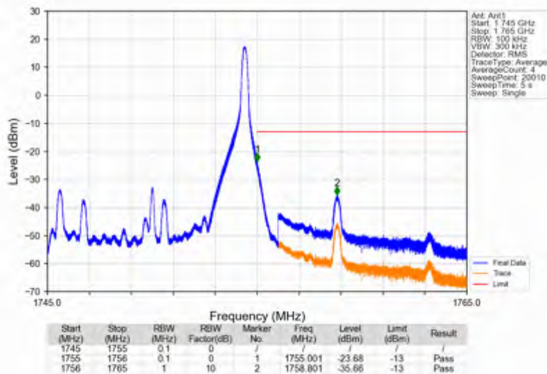
Band4_10MHz_256QAM_HCH_1750MHz_RB_1_49_NTNV
