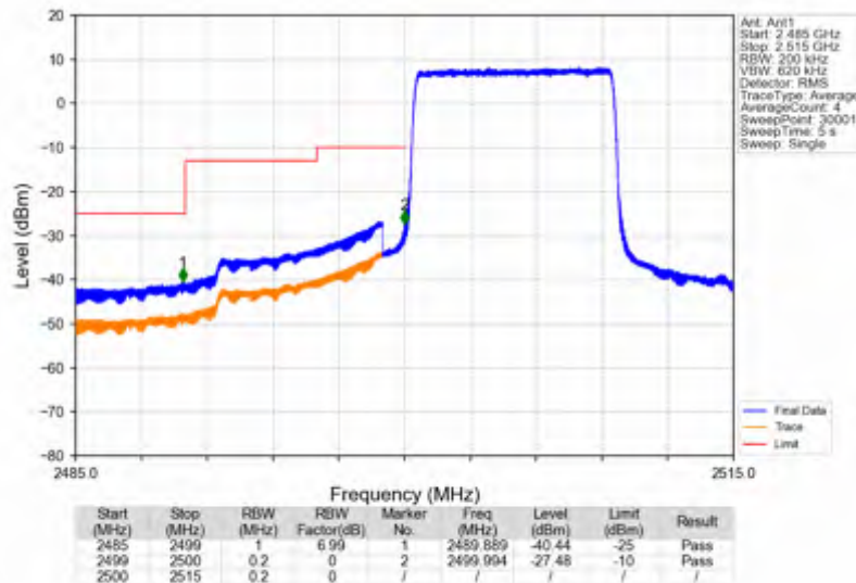
Band7_10MHz_16QAM_LCH_2505MHz_RB_50_0_NTNV
