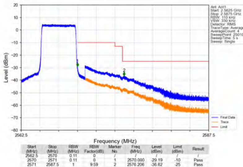
Band7_5MHz_256QAM_HCH_2567.5MHz_RB_25_0_NTNV
