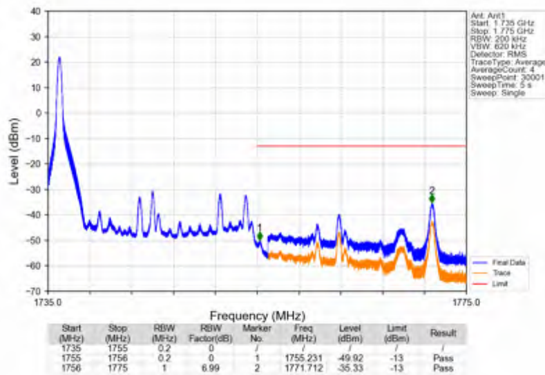
Band4_20MHz_64QAM_HCH_1745MHz_RB_1_99_NTNV
