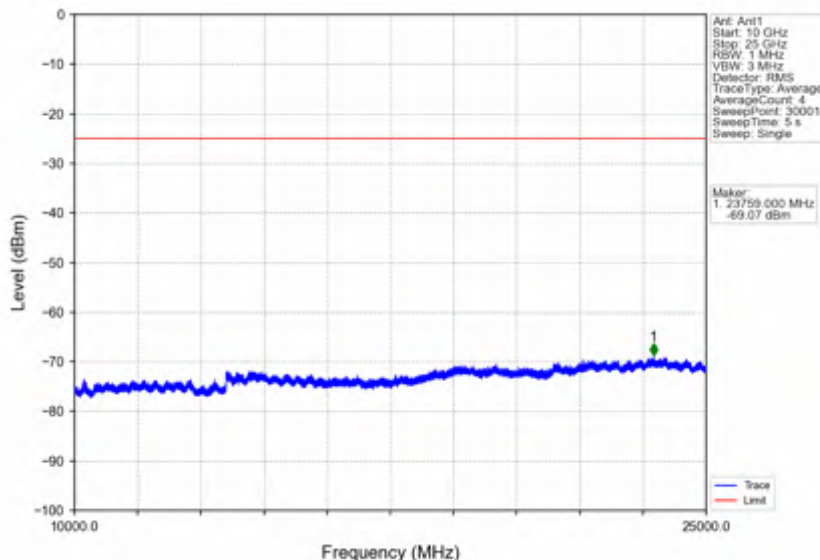
Band7_10MHz_256QAM_LCH_2505MHz_RB_1_0_NTNV
