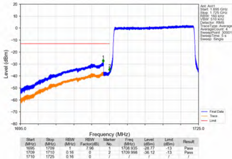
Band4_15MHz_256QAM_LCH_1717.5MHz_RB_75_0_NTNV
