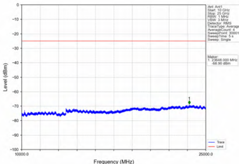
Band7_5MHz_64QAM_HCH_2567.5MHz_RB_1_0_NTNV
