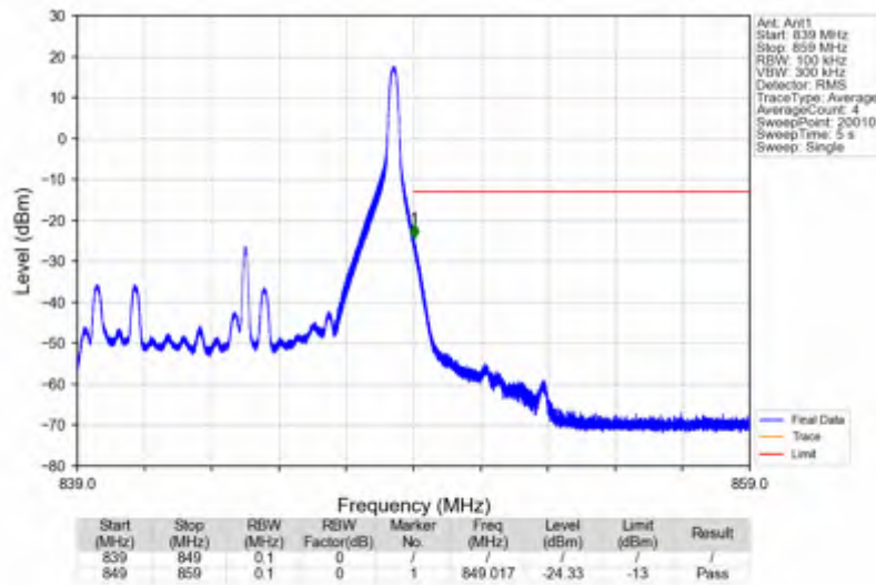
Band5_10MHz_256QAM_HCH_844MHz_RB_1_49_NTV
