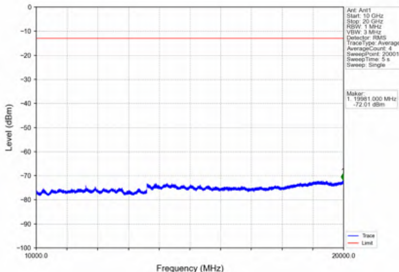
Band4_20MHz_256QAM_HCH_1745MHz_RB_1_0_NTNV
