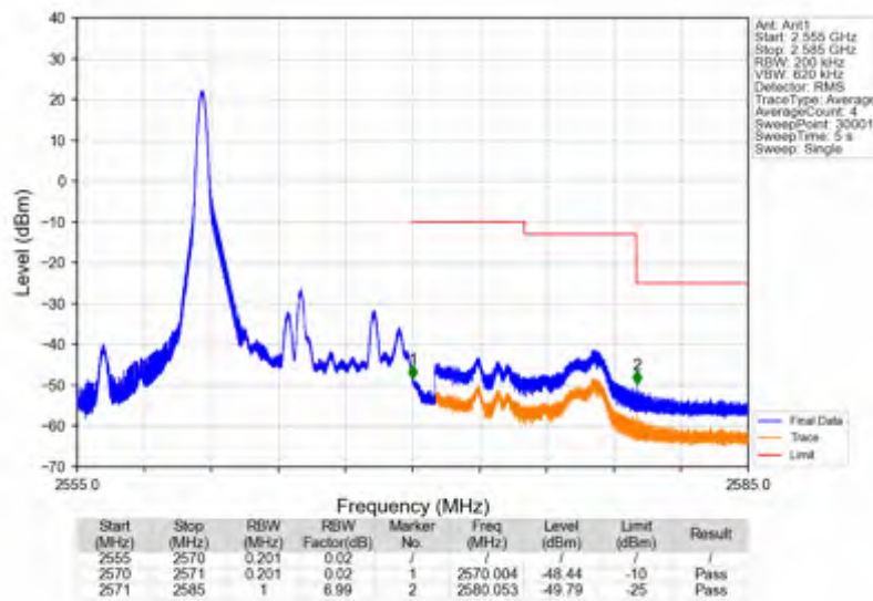
Band7_10MHz_64QAM_HCH_2565MHz_RB_1_49_NTNV
