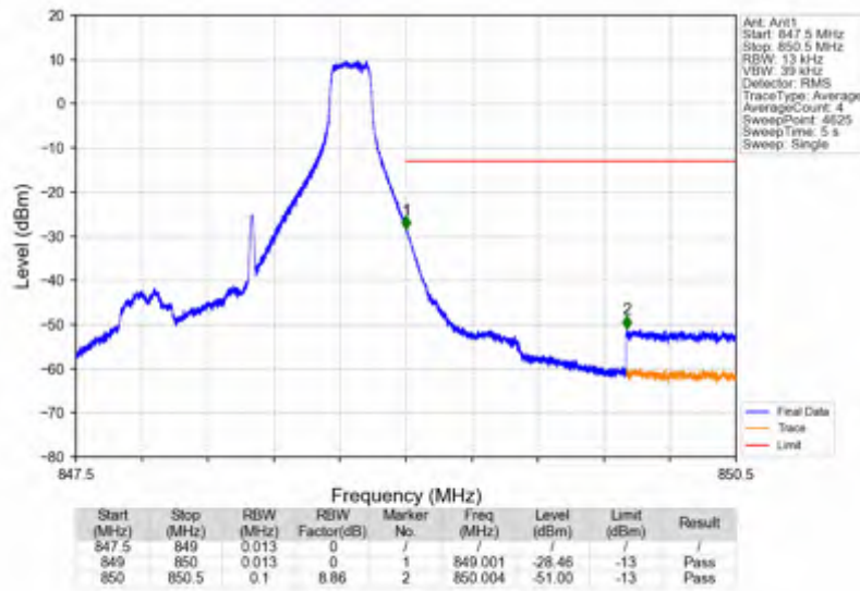
Band5_1.4MHz_256QAM_HCH_848.3MHz_RB_1_5_NTNV
