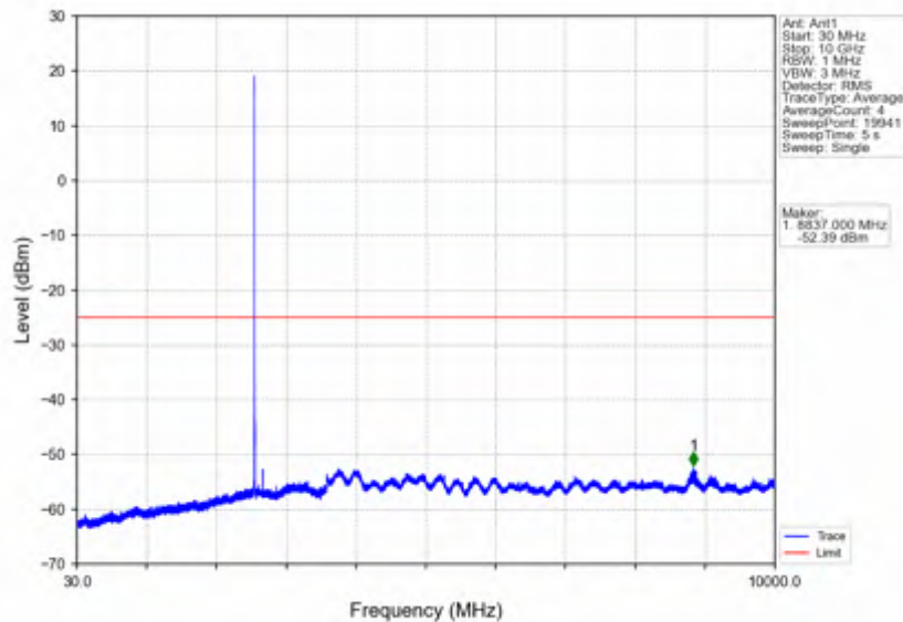
Band7_5MHz_256QAM_HCH_2567.5MHz_RB_1_0_NTNV
