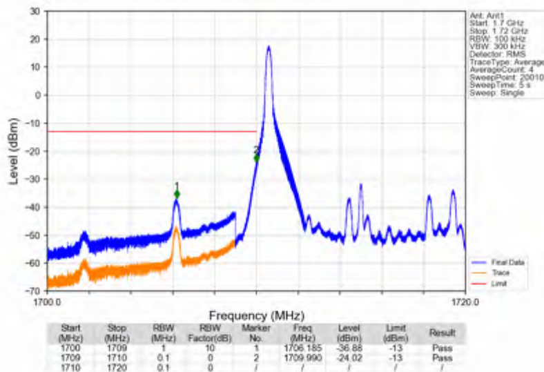
Band4_10MHz_256QAM_LCH_1715MHz_RB_1_0_NTNV
