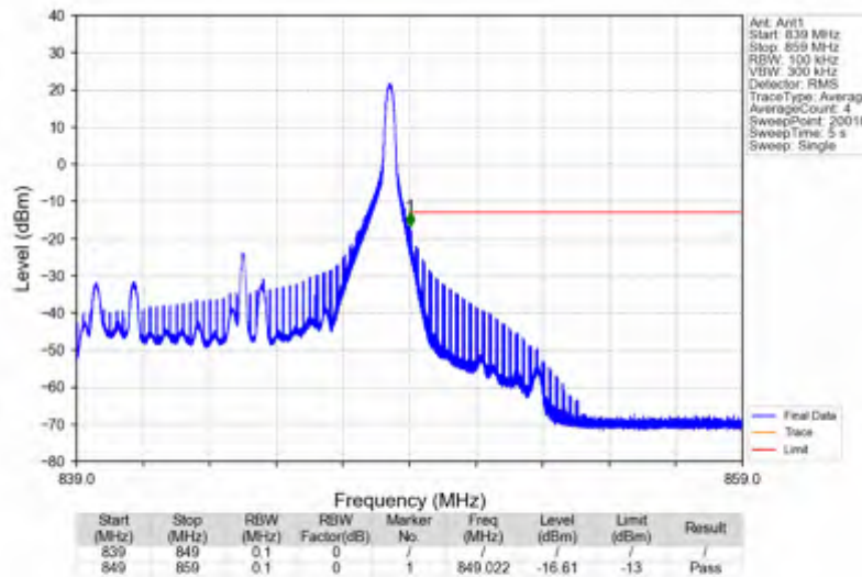
Band5_10MHz_16QAM_HCH_844MHz_RB_1_49_NTNV
