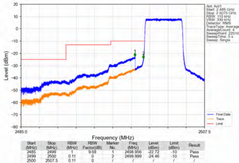
Band7_5MHz_16QAM_LCH_2502.5MHz_RB_25_0_NTNV
