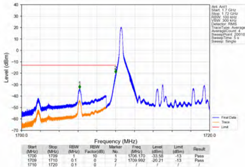
Band4_10MHz_QPSK_LCH_1715MHz_RB_1_0_NTNV
