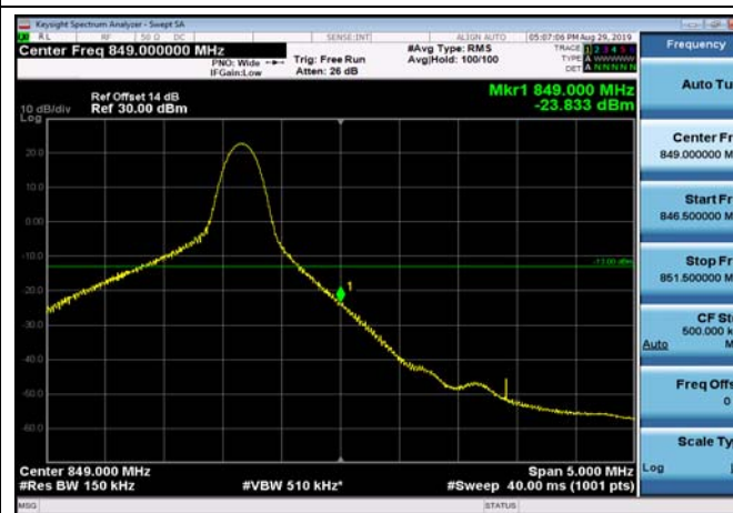
HighRange_FDD26_15MHz_841.5_fullIRB _High_QPSK
