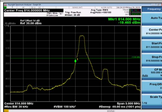
LowRange_FDD26_1.4MHz_814.7_fullRB _Low_QPSK
