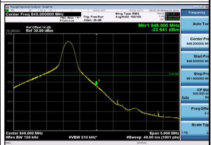
HighRange_FDD26_15MHz_841.5_fullIRB _High_Q16
