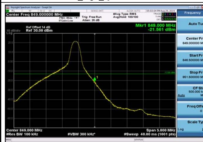
HighRange_FDD26_10MHz_844_OneRB _high_QPSK
