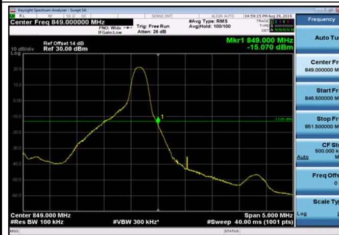
HighRange_FDD26_5MHz_846.5_fullRB _High_QPSK
