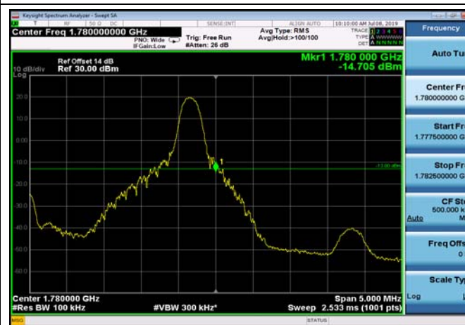
HighRange_FDD66_5MHz_1777.5_fullRB _High_QPSK
