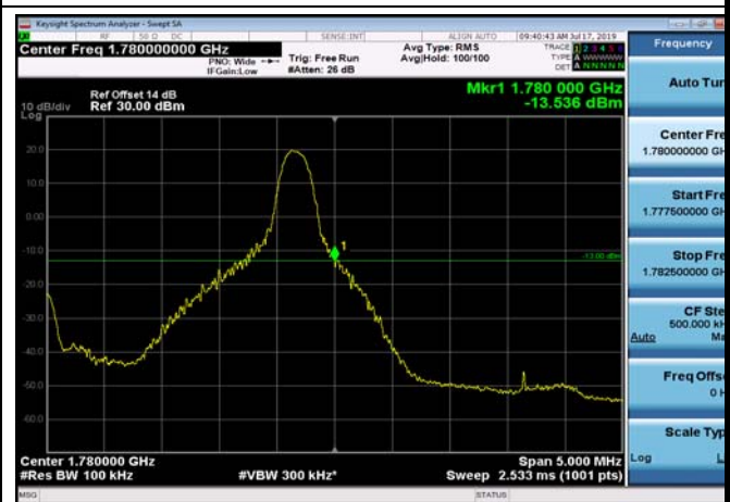
HighRange_FDD66_5MHz_1777.5_fullRB _High_Q16
