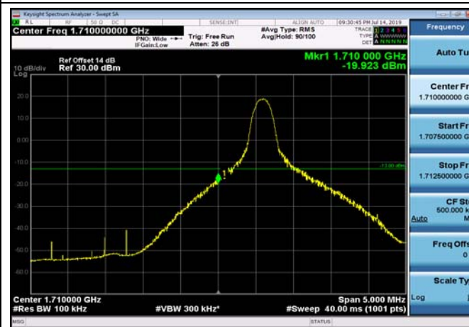
LowRange_FDD66_10MHz_1715_fullRB _Low_QPSK
