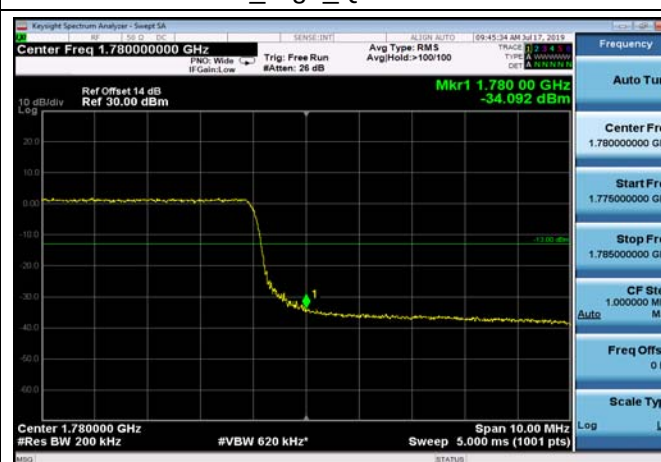
HighRange_FDD66_20MHz_1770_fullRB _High_QPSK
