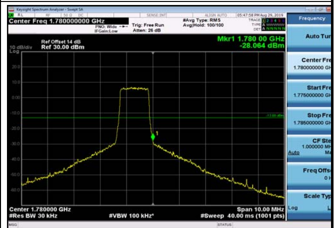
HighRange_FDD66_3MHz_1778.5_OneRB _high_Q16
