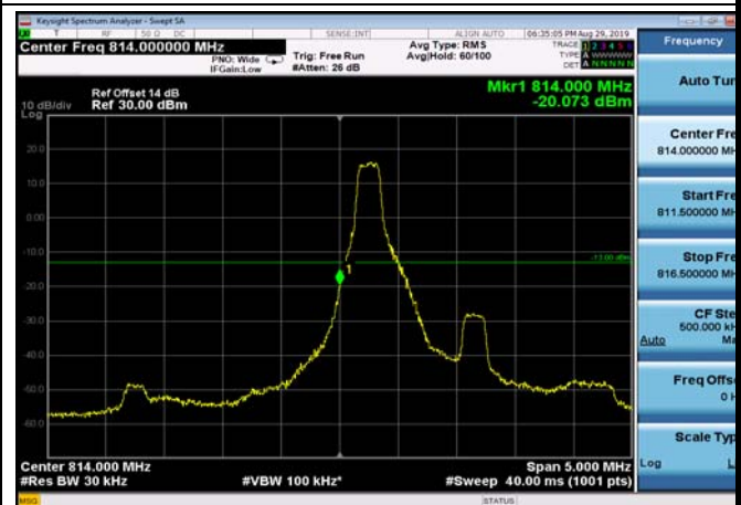
LowRange_FDD26_1.4MHz_814.7_fullRB _Low_Q16
