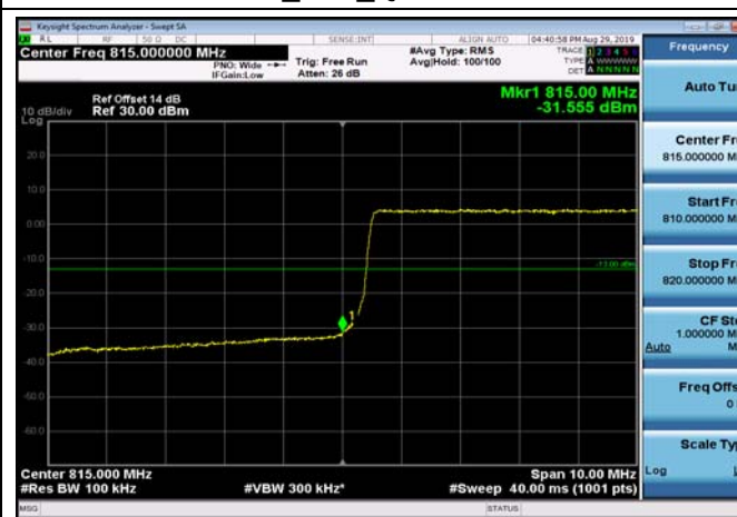
LowRange_FDD26_10MHz_820_fullRB _Low_QPSK
