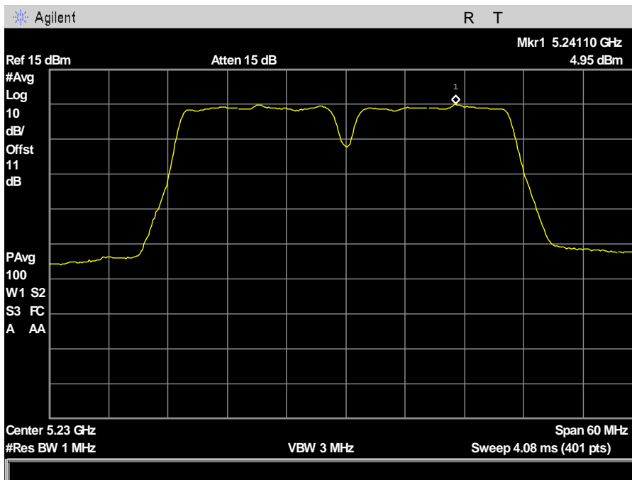
Plot 11. Power Spectral Density, 11 dBi configuration, CF 5230 MHz
