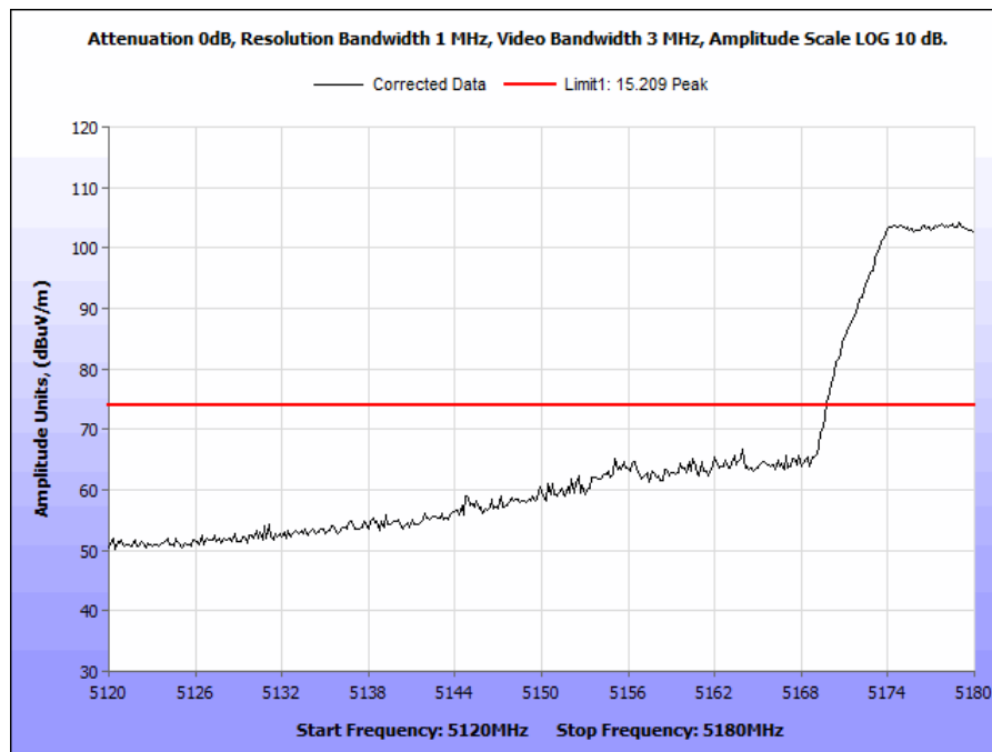
Plot 13. Radiated Bandedge, Peak, 5150 MHz, BW40, CF 5190 MHz, rx, 2 dBi
