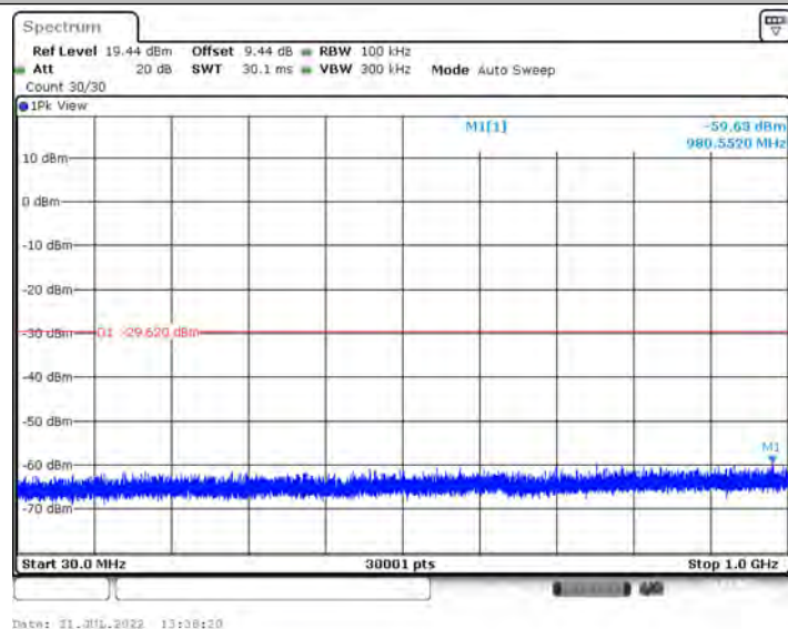
11N20SISO_Ant1_2412_0~Reference
