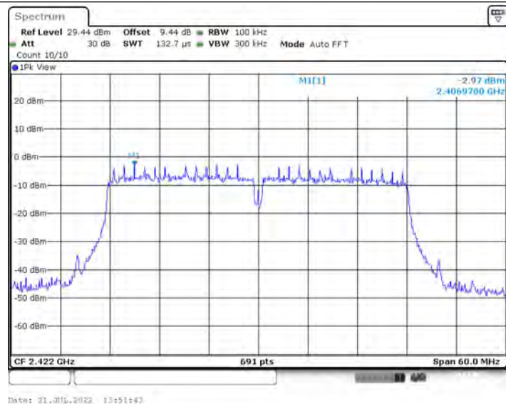
11N40SISO_Ant1_2422_0~Reference
